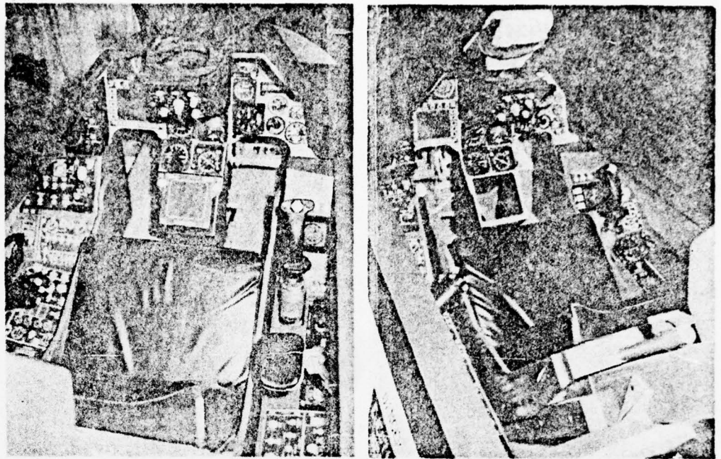
2 Views of F-16 Cockpit Mockup
