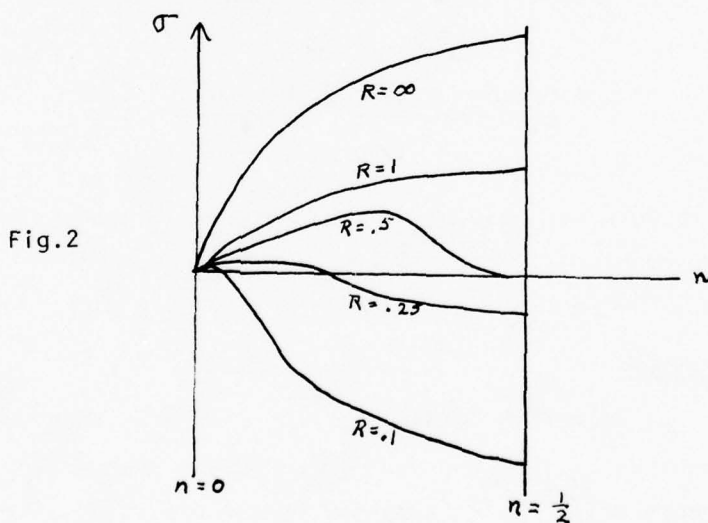
Graph of \sigma against n for 0 \leq n \leq \frac{1}{2} when \omega = 0 . (See section 2.4 for the explanation of these quantities.)
