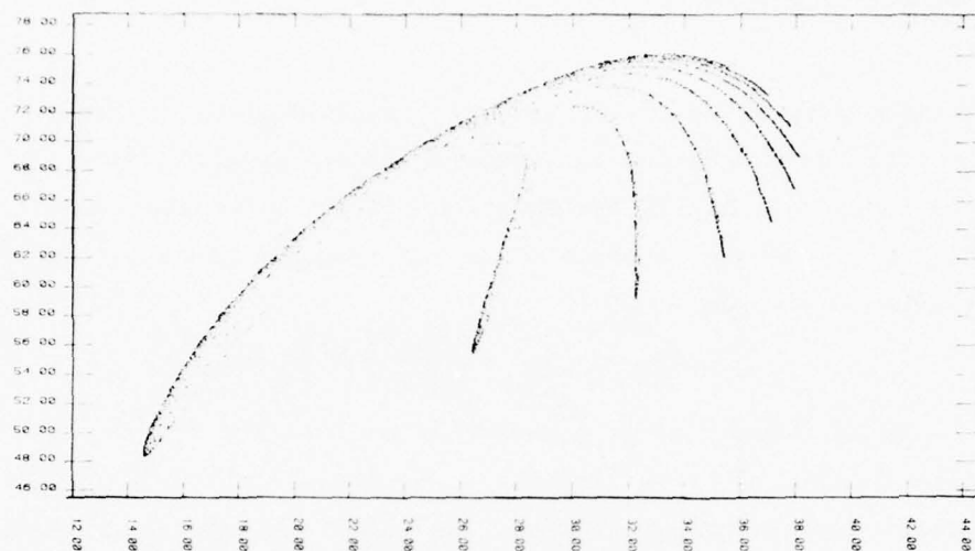
Fig.1. Surface of section ( s=0 ) in (E, B, s) space of the attractor of (1)-(4) for \mathcal{E} = .625 .
