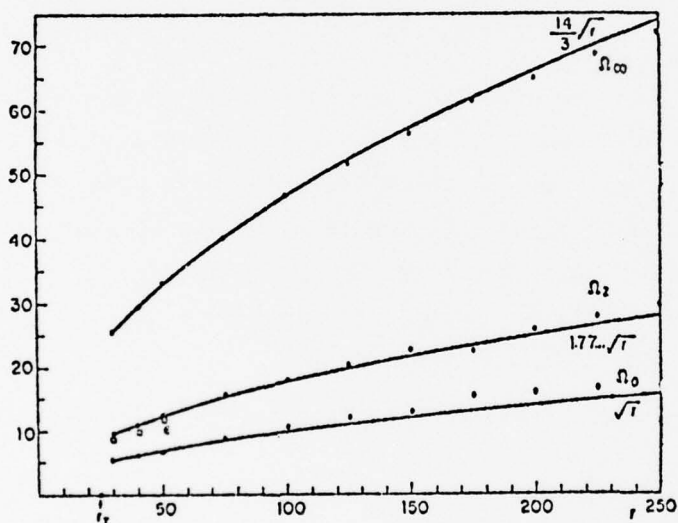
Characteristic frequencies (dots) of the model for various values of r . Solid lines denote the curves \sim \sqrt{r} , 1.77 \dots \sqrt{r} , and (14/3) \sqrt{r} , respectively. Squares represent the oscillation frequencies \epsilon of \phi_{33}(t) , according to Fig.5.
