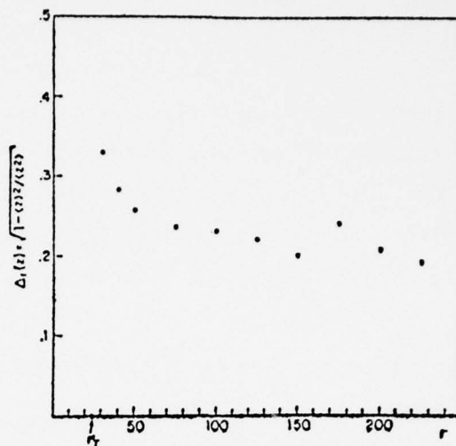
Average normalized fluctuations \Delta_r(z) = \Delta \langle z \rangle / \langle z^2 \rangle^{1/2} for various values of r . Fig.2
