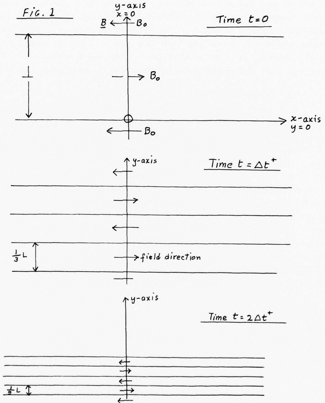
The stretching and folding procedure. (See Section 1.6.)
