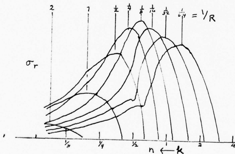
Fig.4. Numerical computation (G.O.Roberts, 1972) of the growth rate \sigma_r as function of k and \frac{1}{R} for \underline{u}_1 , given by (3.14).
