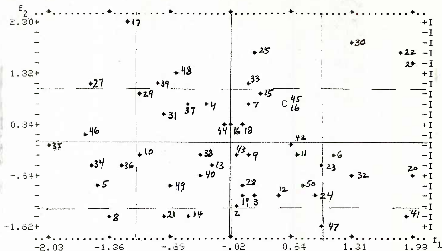
Figure 1. Scattergram of the Factor-Scores f_2 Versus f_1 for the Data of Table 5.
