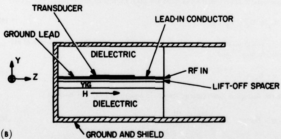
Figure 2. Delay Line Configuration for Magnetostatic Waves. a. A magnetostatic surface wave delay line configuration showing a grating and meander line transducer structure. b. Transducer connections to ground plane structures
