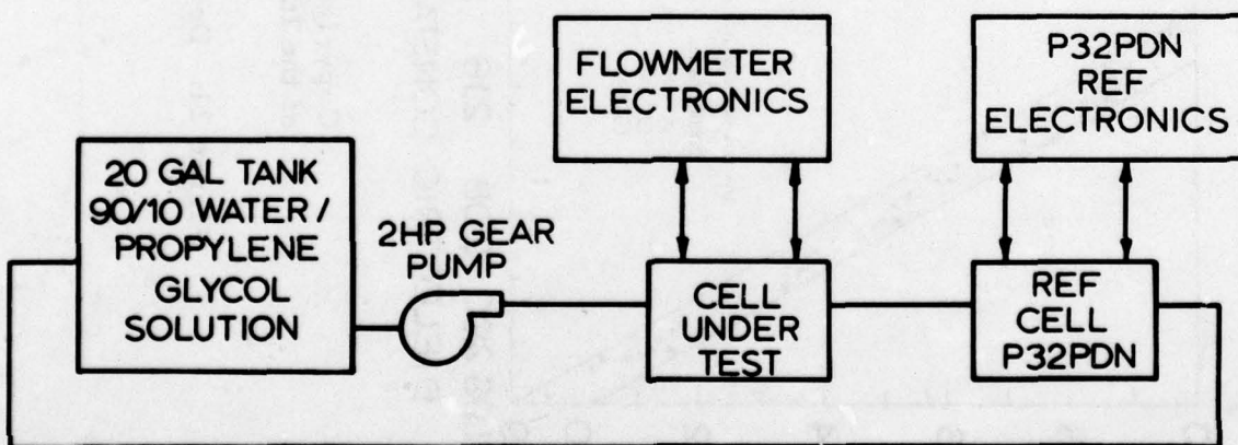
Figure 23. High-pressure test loop.
