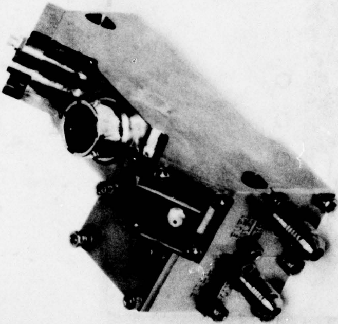
Above: Oblique view shows SS316 cell body; AN-3 and AN-4 fuel outlet and inlet, respectively; multipin electrical connector for \rho and V measurements; \mu dot connectors for testing ultrasonic transducers and velocimeter.
