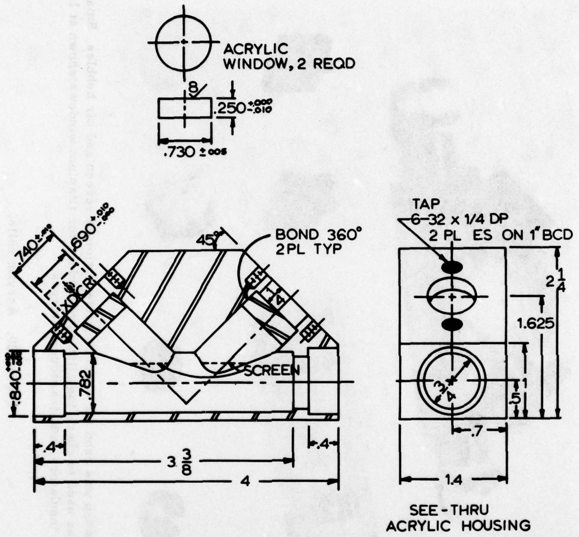
Figure 19. Transparent flow cell to test if screens trap vapor bubbles (e.g., air bubbles in water).
