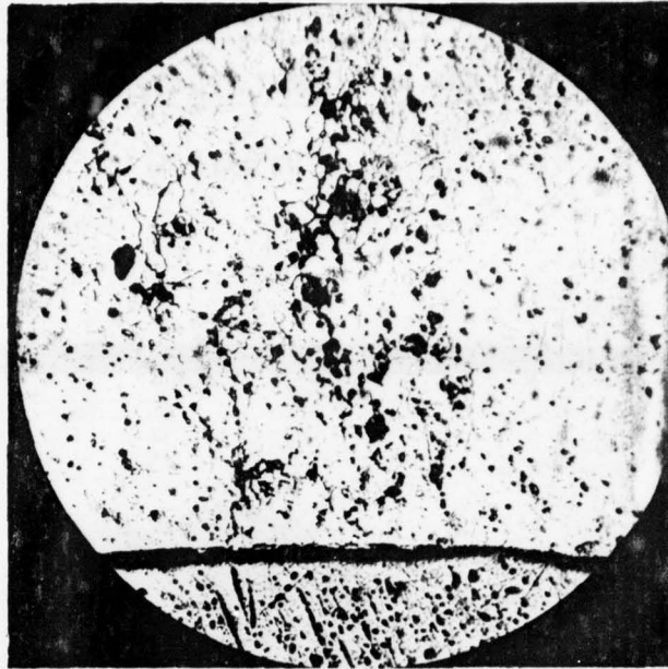
FIGURE 4 Intercrystalline corrosion and pitting on specimen 24.18.C (Stage I type) Dimensions of network { 0.022" Radially 0.019" Circumferentially (x 125)
