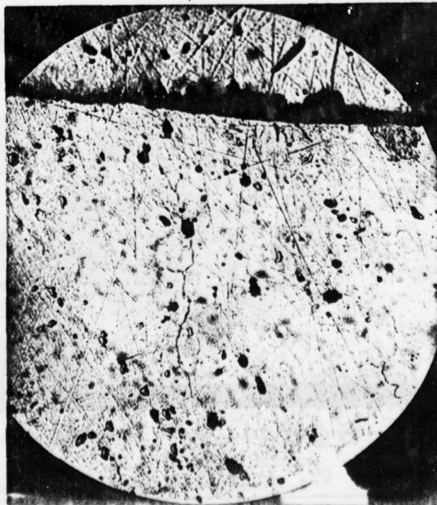
FIGURE 3. Incipient stress corrosion cracking on specimen 24.18.C (Stage I type) Approx. length 0.008" (x 312)
