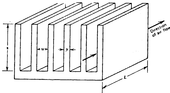
FIGURE D-2 Geometry of forced air cooled heat sink and important dimensions
