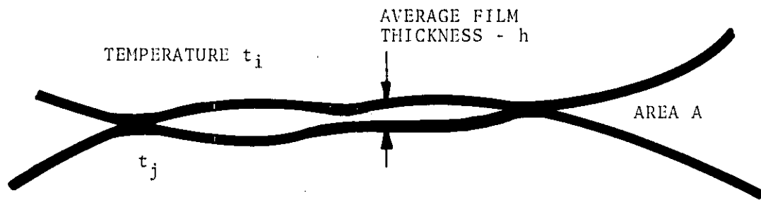
(a) Schematic Concentrated Contact
