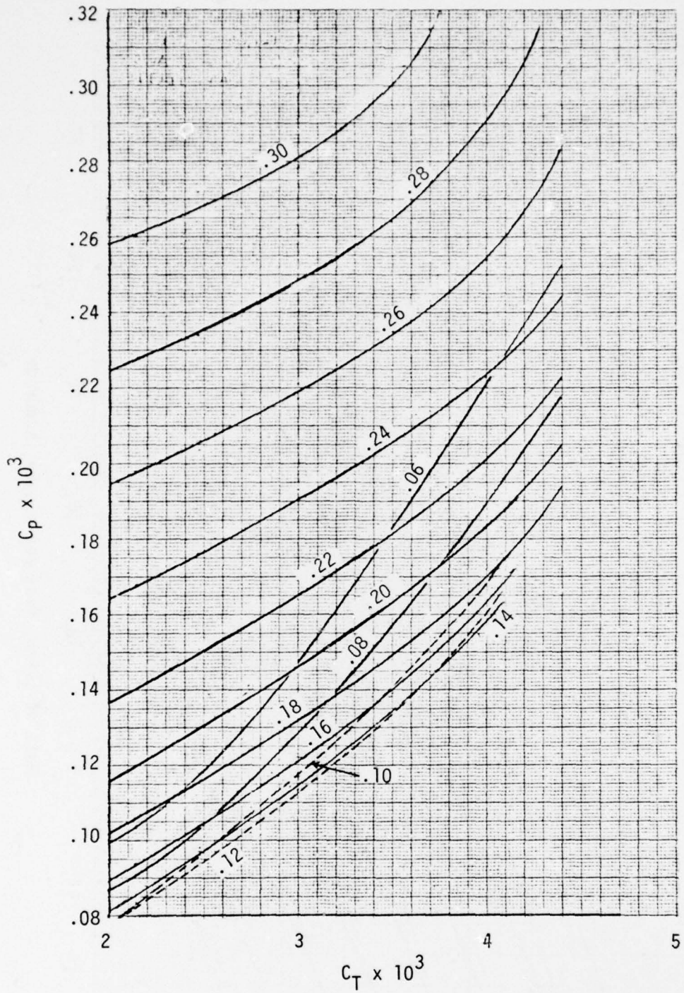
Figure 38. OH-58 C/A - K757 forward flight nondimensional performance data.
