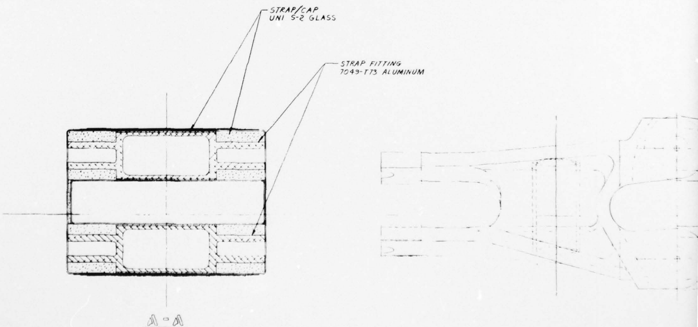
Figure 33. Root end details - configuration 111.
