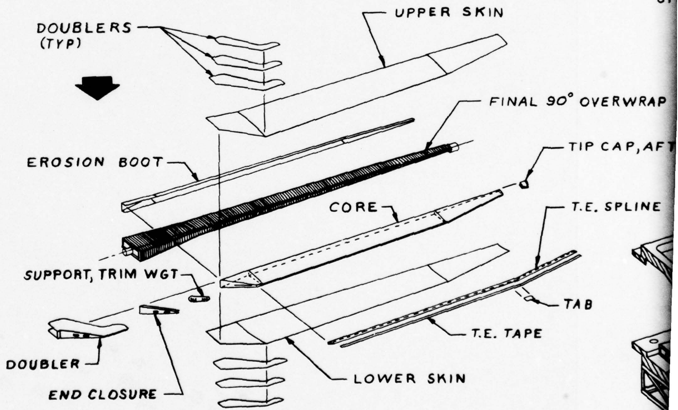
Figure 61. Manufacturing sequence.
