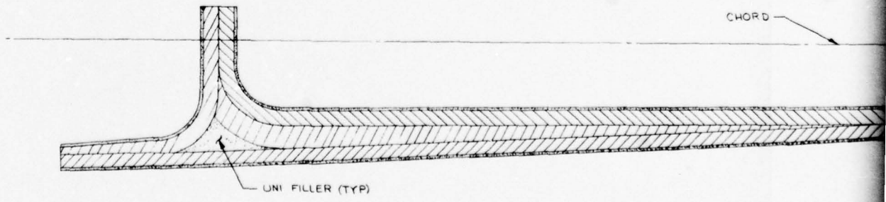
Figure 10. Two-piece pultruded afterbody.
