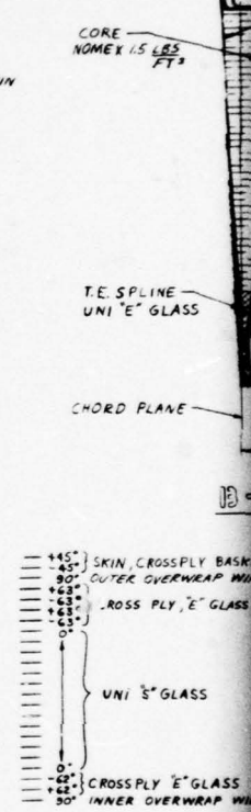
LAYUP SCHEDULE AT STA 36.5
