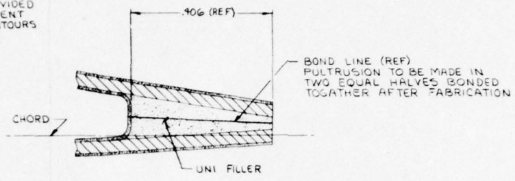
DETAIL B SCALE 10:1
