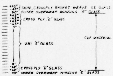
D LAYUP SCHEDULE AT STA 36.5
