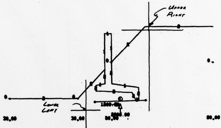
Figure 13. Window command
