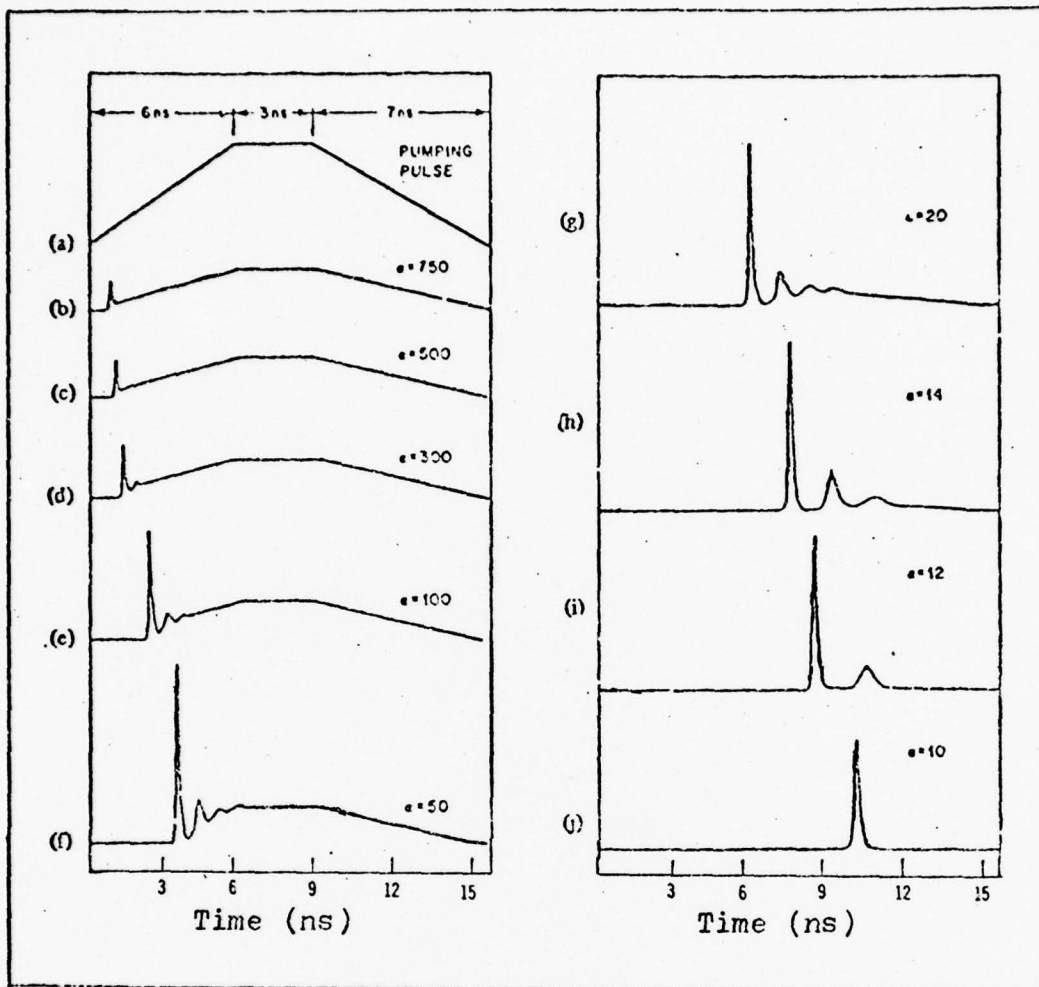
Figure IV-1: Results of C. Lin (Ref 7:607). \tau_c is 50ps, \alpha is the level of pumping above threshold and is indicated for each plot. Figure (a) is the pump pulse used.
