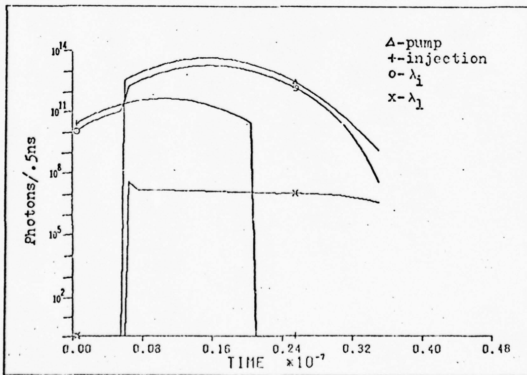
Figure IV-10: Computer solution for a delay time of 5 ns, \lambda_l is at 590 nm, and \lambda_i is at 600 nm.
