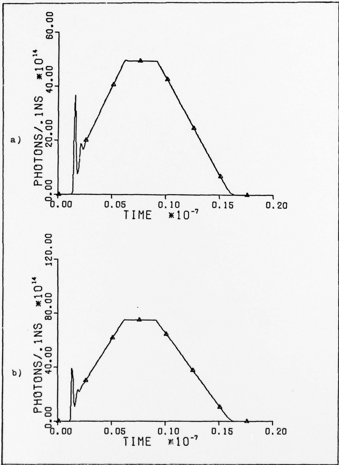
Figure B-3: Plots of the solutions of the rate equations. Figure (a) is for 500 times the threshold pump rate and (b) is for 750 times threshold.
