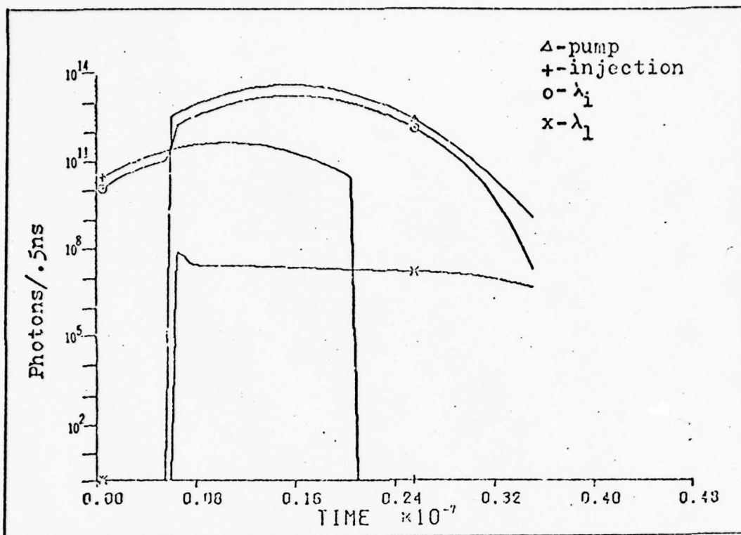
Figure IV-9: Computer solution for a delay time of 5 ns, \lambda_l is at 590 nm, and \lambda_i is at 620 nm.
