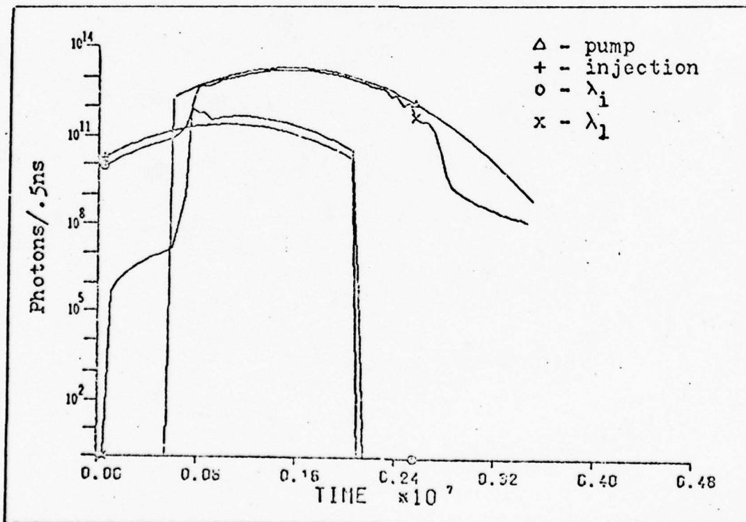
Figure IV-12: Computer solution for a delay time of 5 ns, \lambda_i is at 580 nm, \lambda_1 is at 590 nm, and the mirror reflectivity is 20%. Injection locking is still not achieved, but the output at the desired wavelength is larger than that obtained for mirror reflectivities of 95%.
