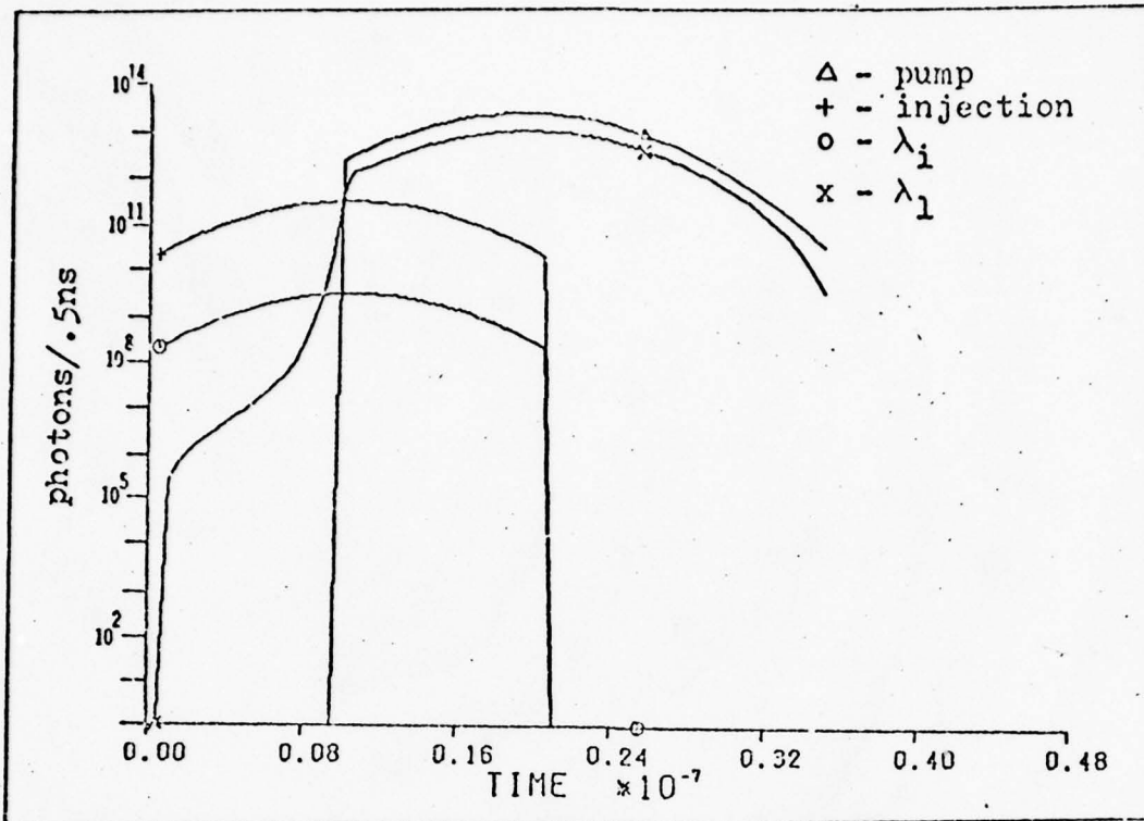
Figure IV-11: Computer solution for a delay time of 9 ns, \lambda_i is at 560 nm, and \lambda_1 is at 590 nm. The injection causes the cavity to begin lasing at 590 nm due to the strong reabsorption and \lambda_i .
