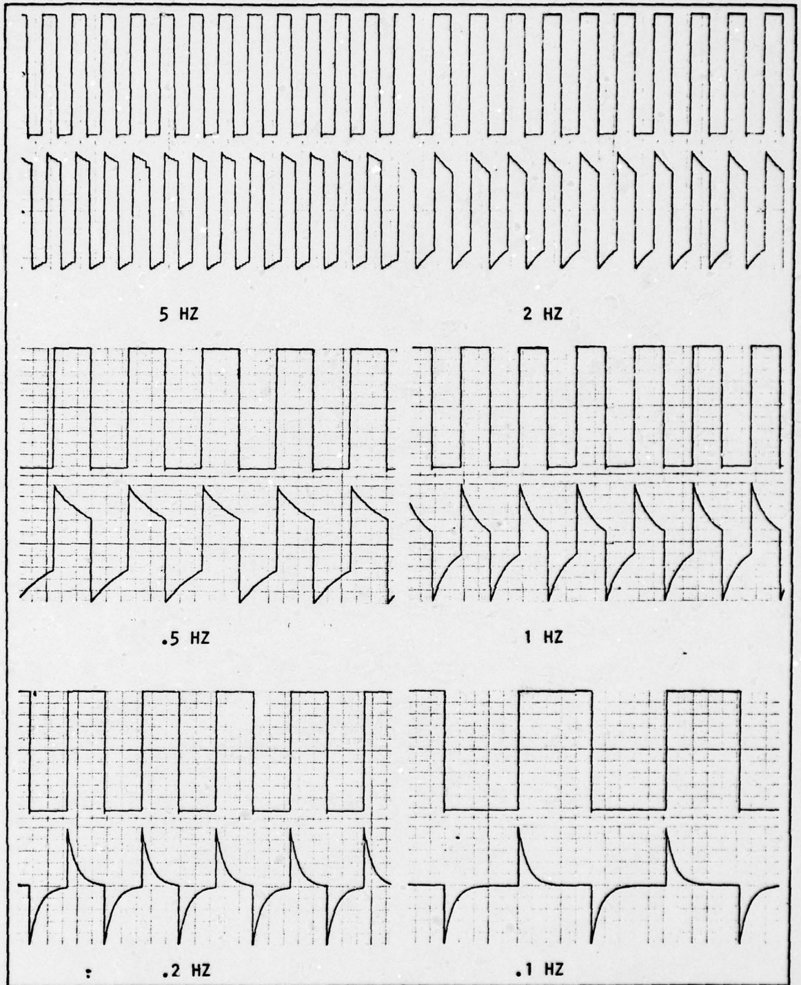
Figure 7-4: Frequency Response of Digital Filter (Square Wave)
