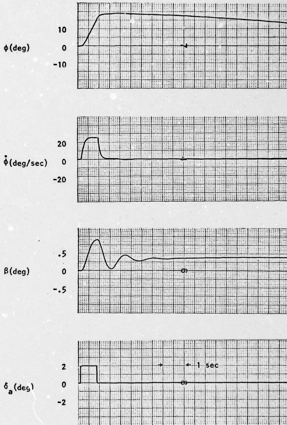
Figure A-44: Free RPV Airframe Response to a Pulse Aileron Deflection (Case 11); Without Actuator
