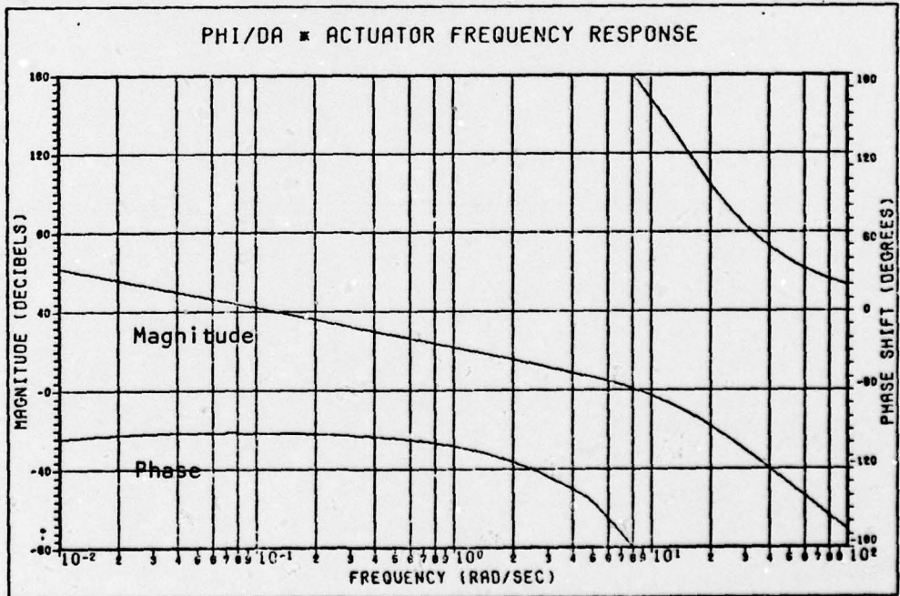
Figure A-4b: \phi/\delta_a * Actuator Frequency Response
