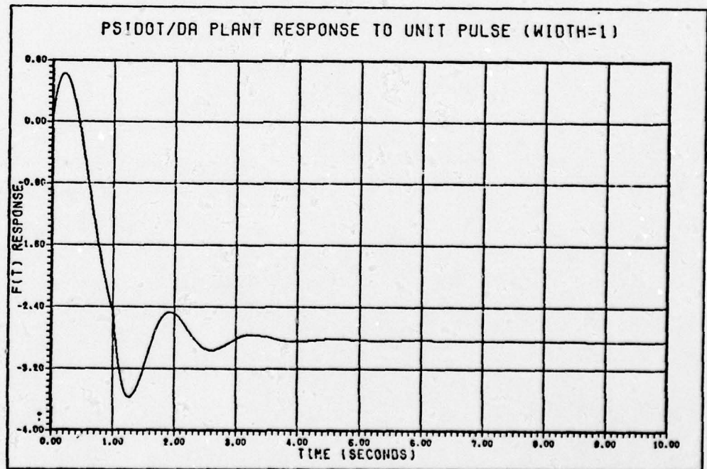
Figure A-19b: \psi/\delta_a Time Response
