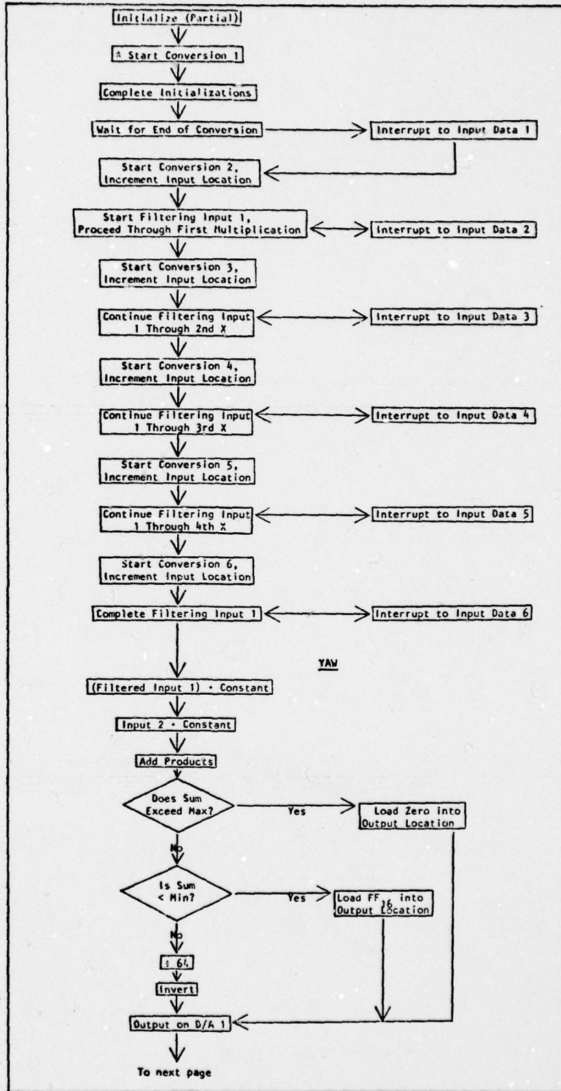
Figure 6-4: 3-Axis Flowchart
