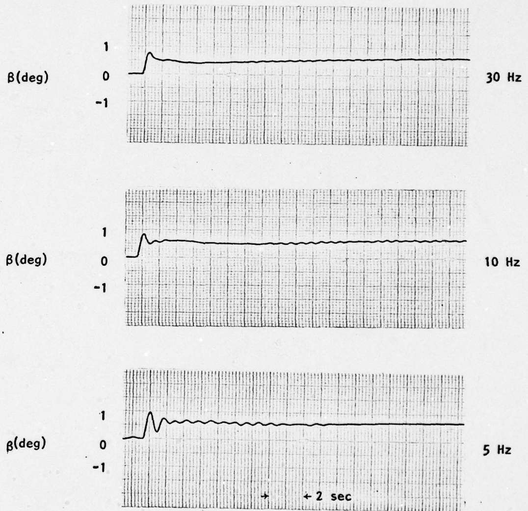
Figure 7-17: Sideslip Angle( \beta ) Response to 20 Degree Step Roll Right Command( \phi ) Versus Sampling Frequency( f_s ); Full Digital Controller Engaged
