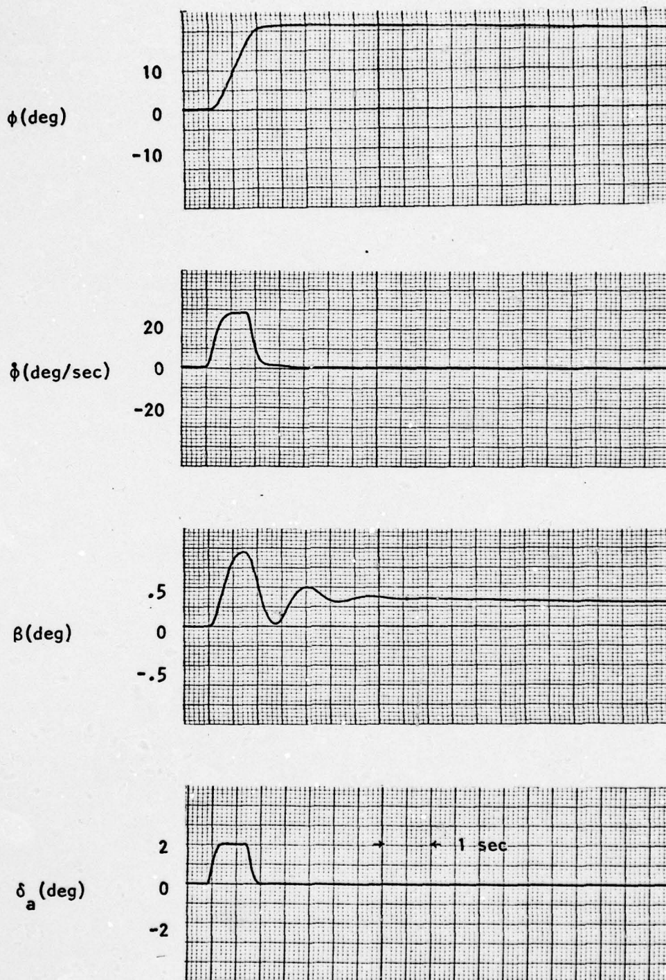
Figure A-45: Free RPV Airframe Response to a Pulse Aileron Deflection (Case II); With Actuator
