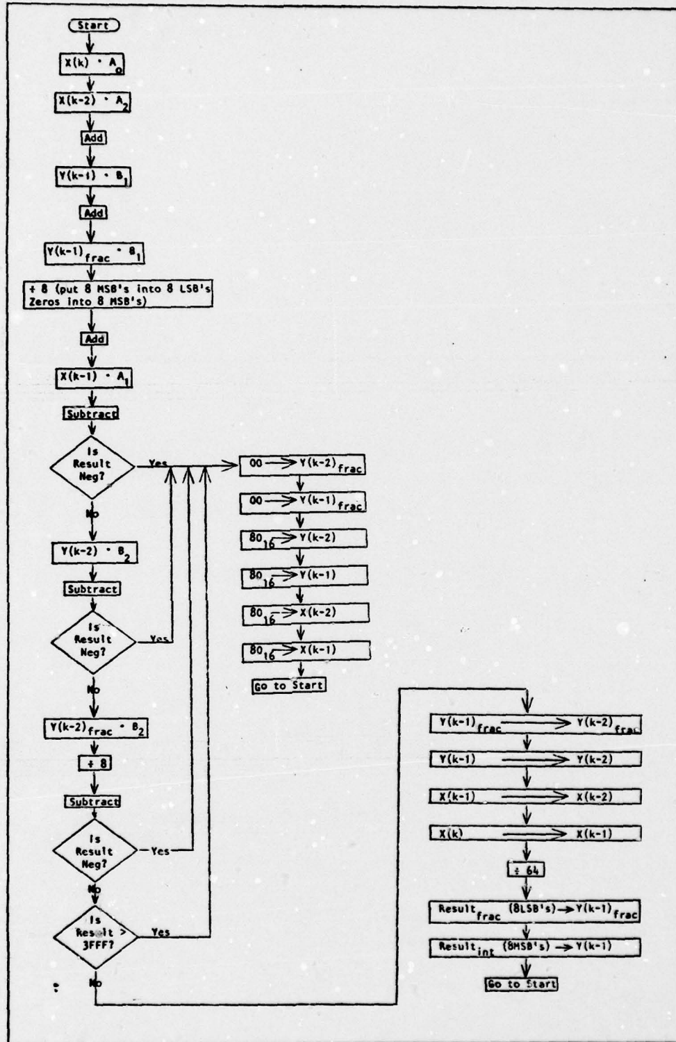
Figure 6-3: Filter Flowchart
