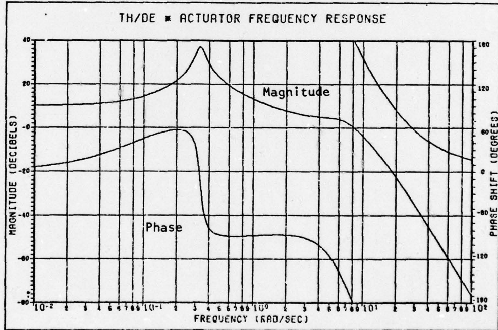
Figure A-1b: \theta/\delta_e * Actuator Frequency Response
