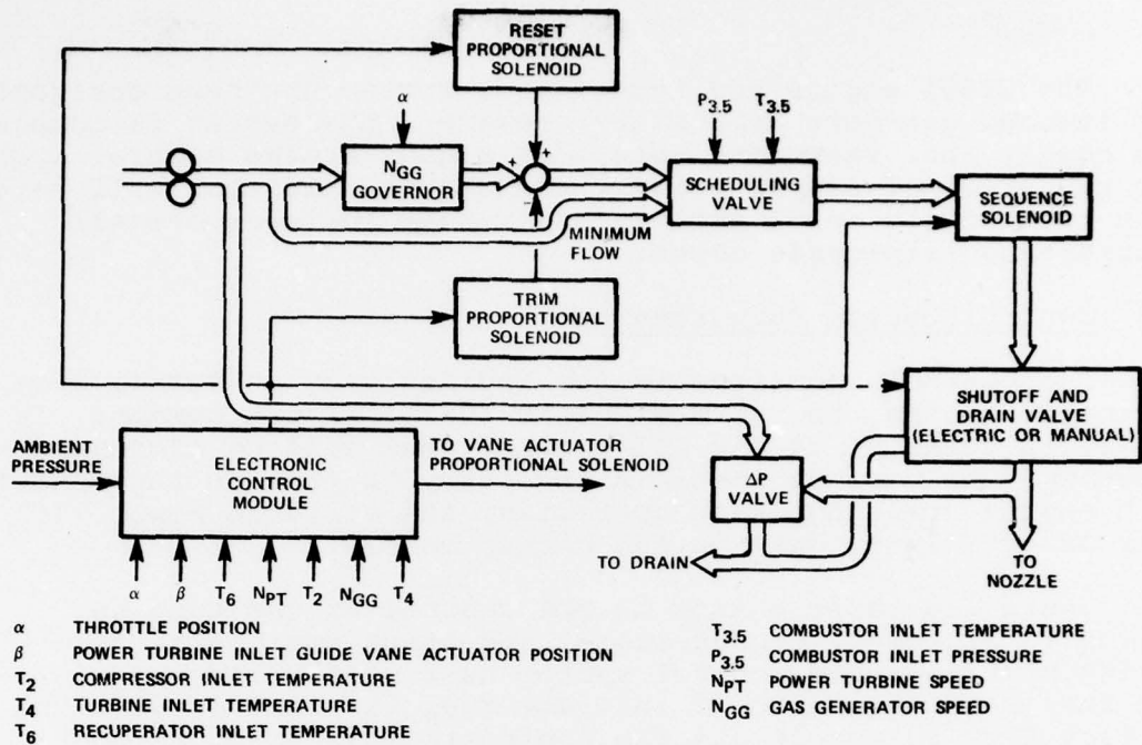
Figure 4. Block diagram of existing fuel control system for GT601 engine.
