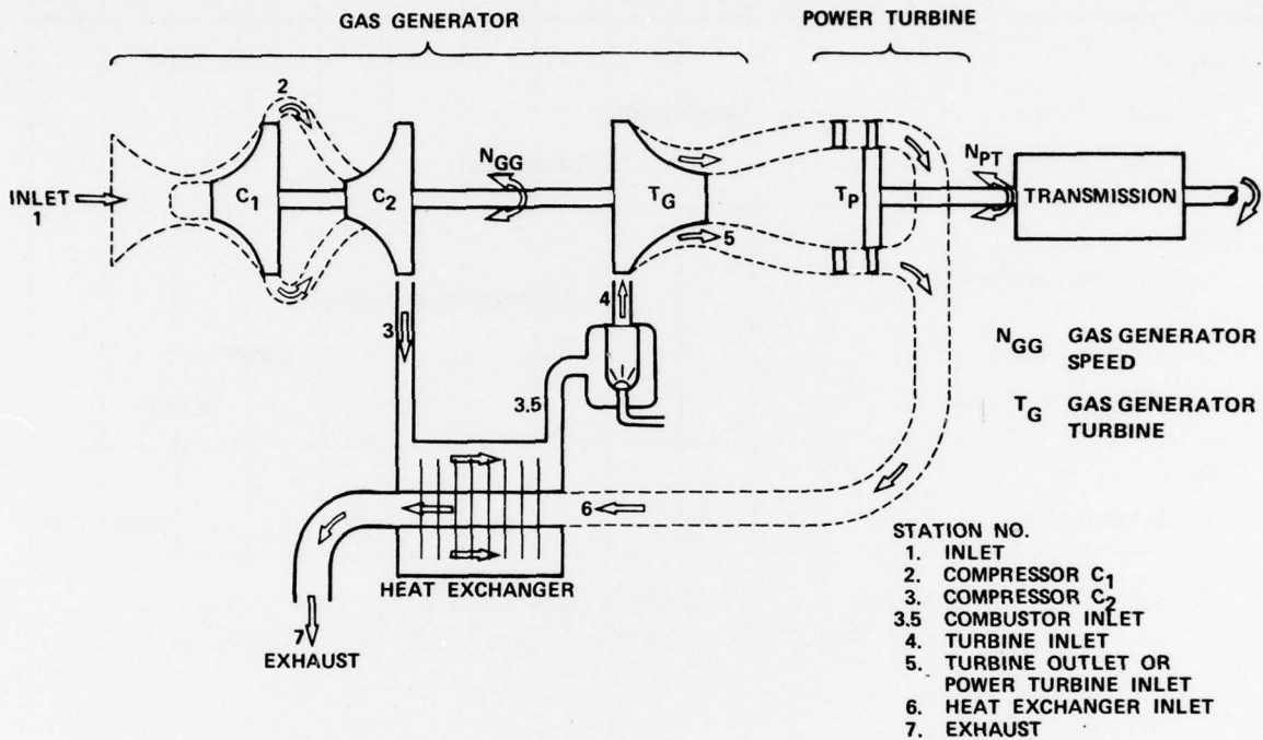
Figure 2. Schematic diagram of typical military automotive gas turbine engine.
