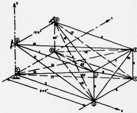
Figure 3. Twenty-two Member Space Truss
