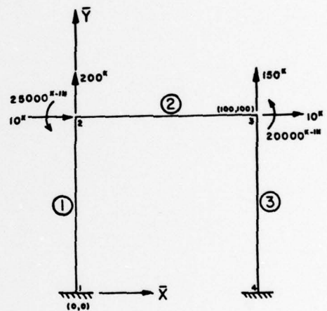
Figure 7. Three Member Frame
