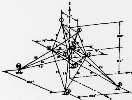
Figure 4. Twenty-five Bar Transmission Tower Truss
