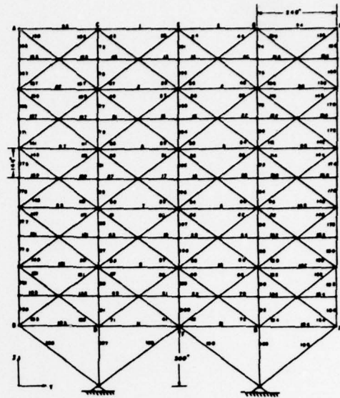
Figure 6. Two Hundred Member Planar Truss
