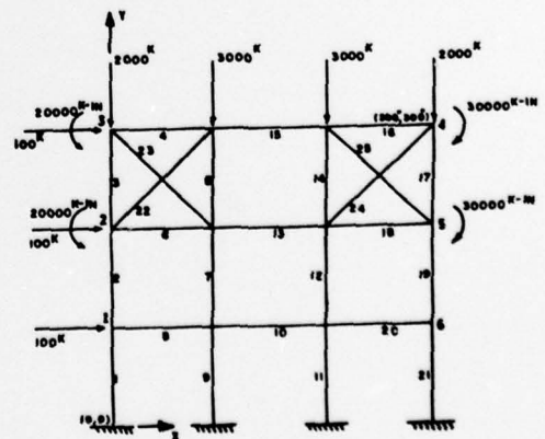
Figure 8. Twenty-five Member Frame
