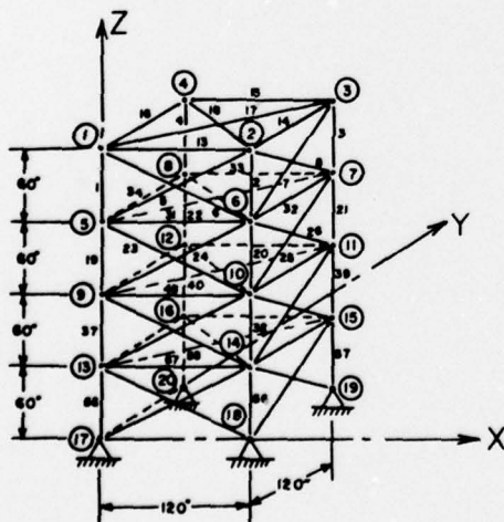
Figure 5. Seventy-two Member Space Truss
