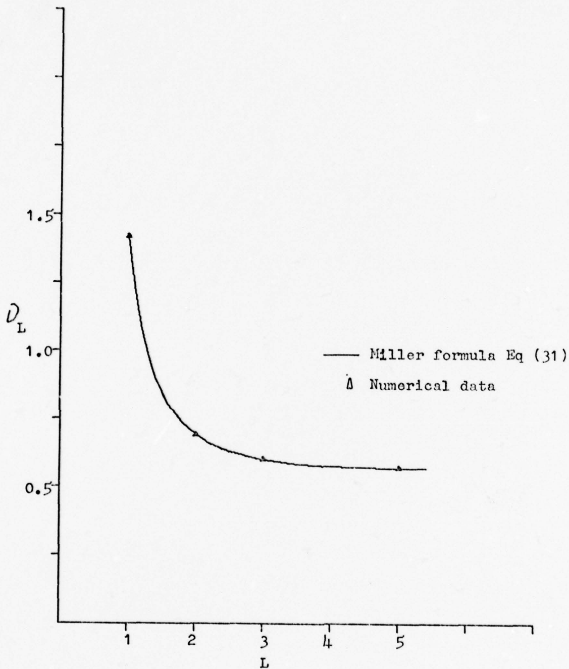
Figure 13. Limiting currents for a=0.0 , b=1.0 , \zeta_0=2.0
