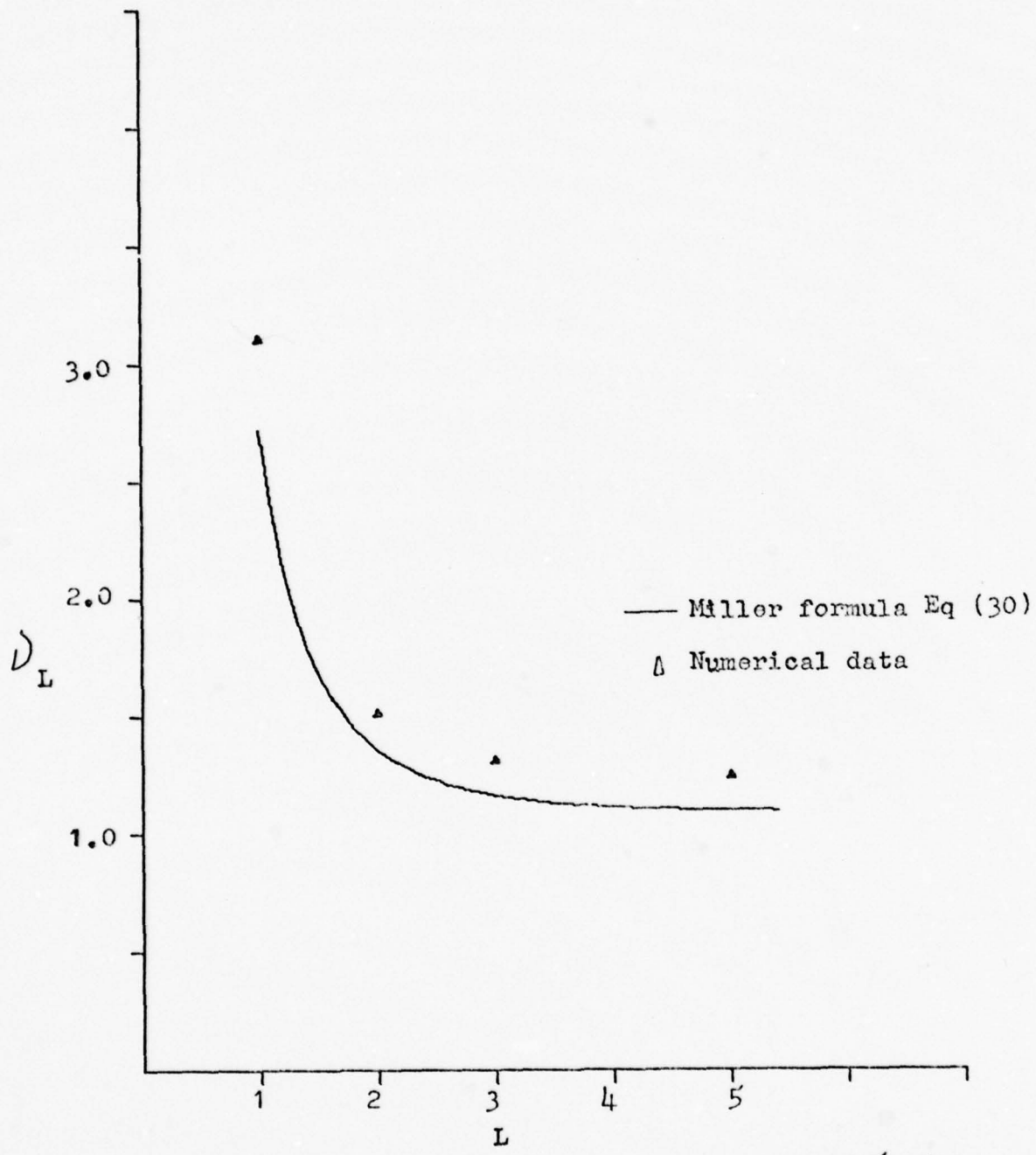
Figure 5. Limiting currents for a=0.0 , b=0.5 , \zeta_0=5.0
