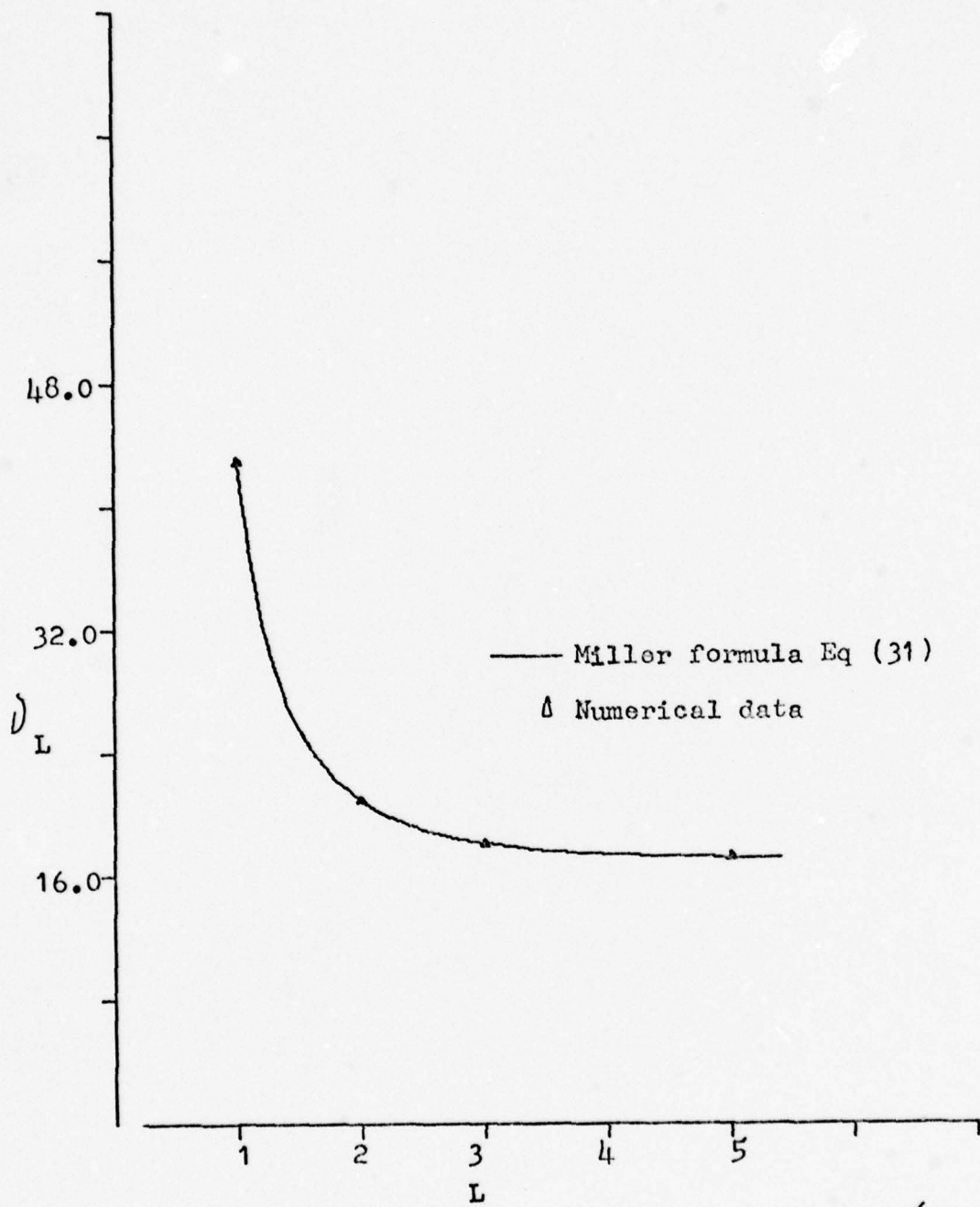
Figure 15. Limiting currents for a=0.0 , b=1.0 , \gamma_0=20.0
