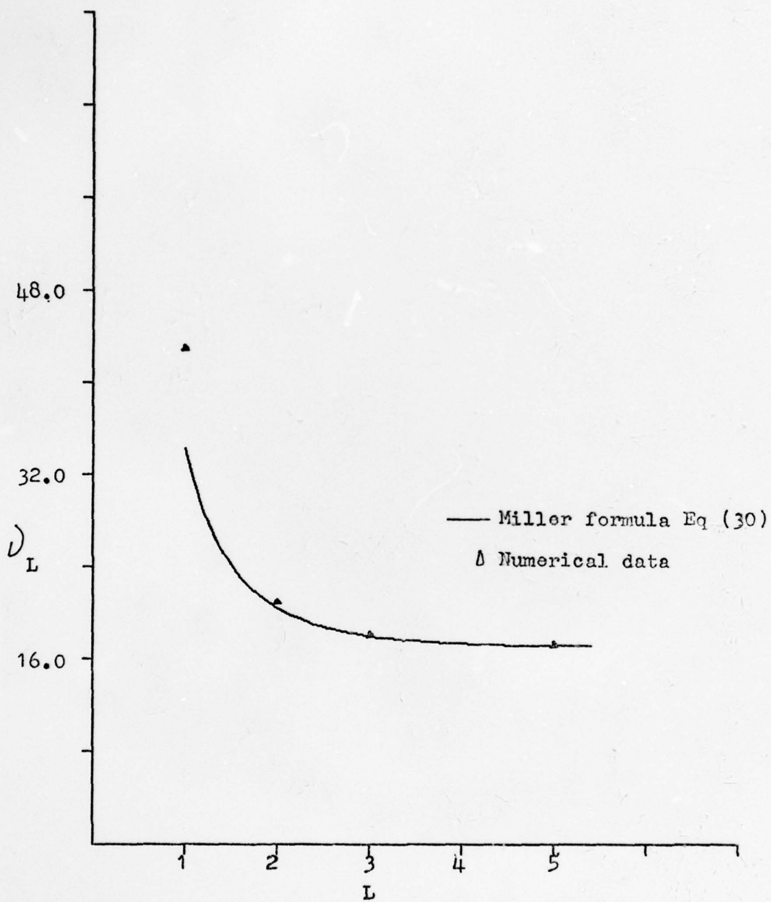
Figure 9, Limiting currents for a=0.0 , b=1.0 , \gamma_0=20.0
