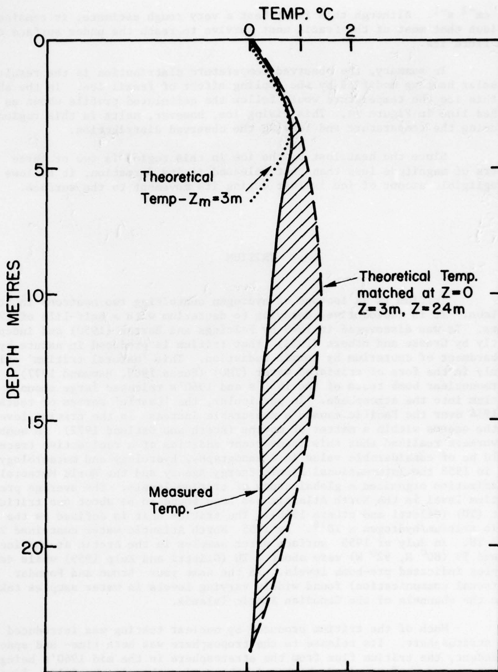
Fig. 19: Measured and calculated temperature profiles.
