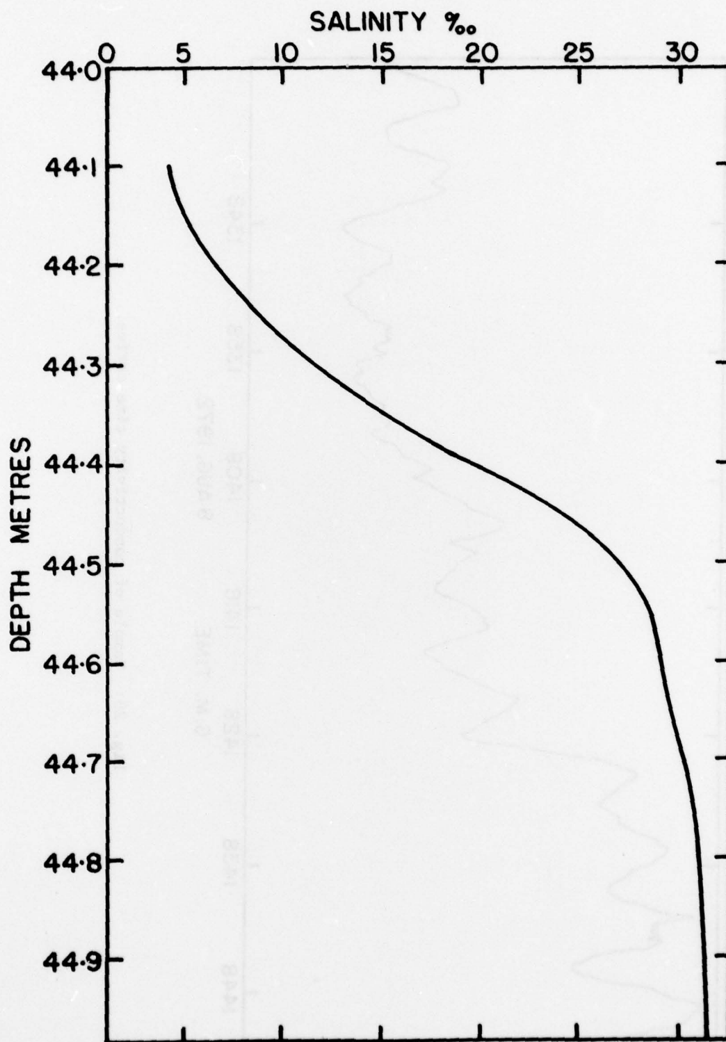
Fig. 28: Salinity profile across the halocline.
