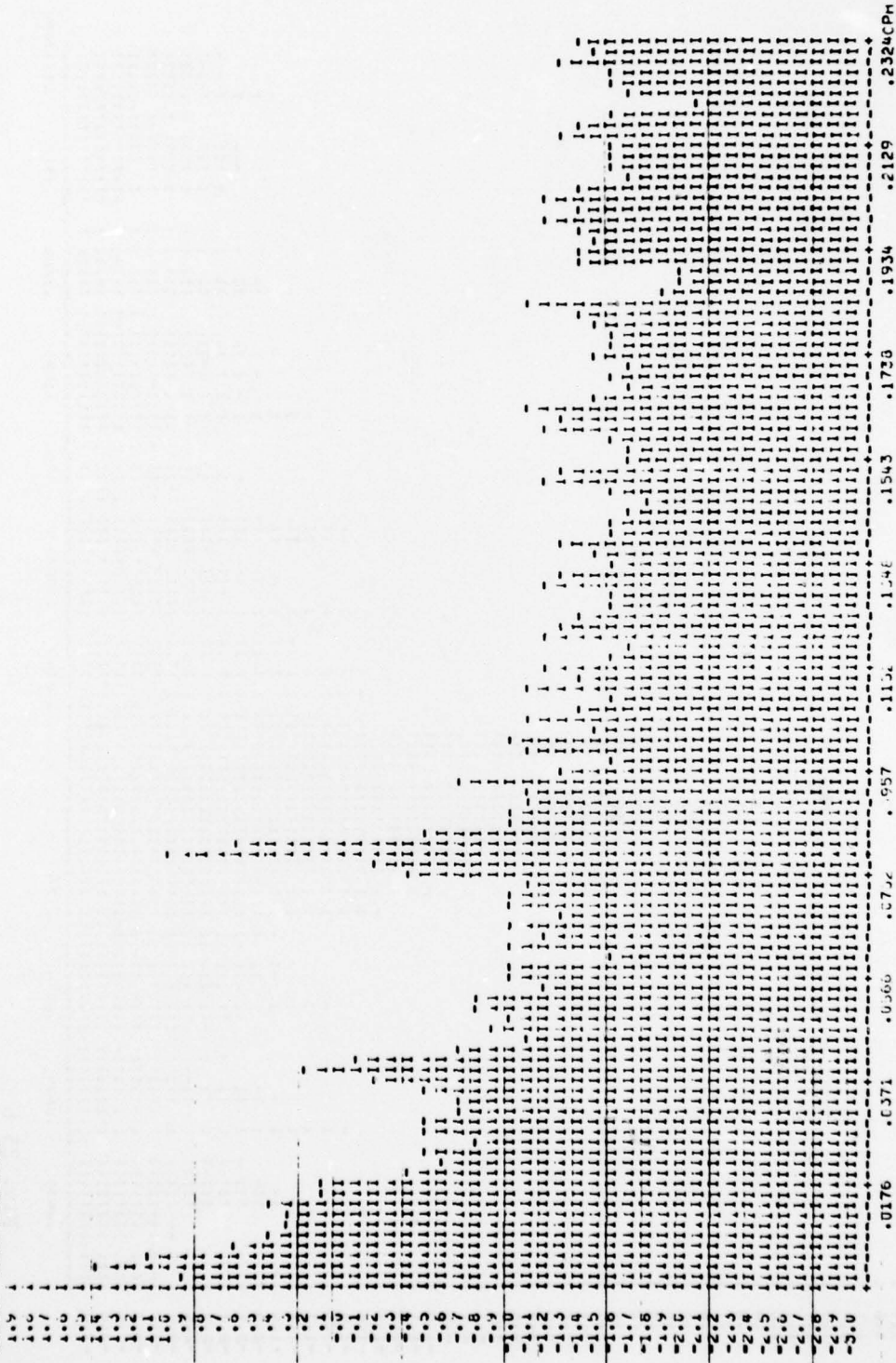
Fig. 26: Power spectrum of the residuals showing peaks at about 12 and 24 hours.
