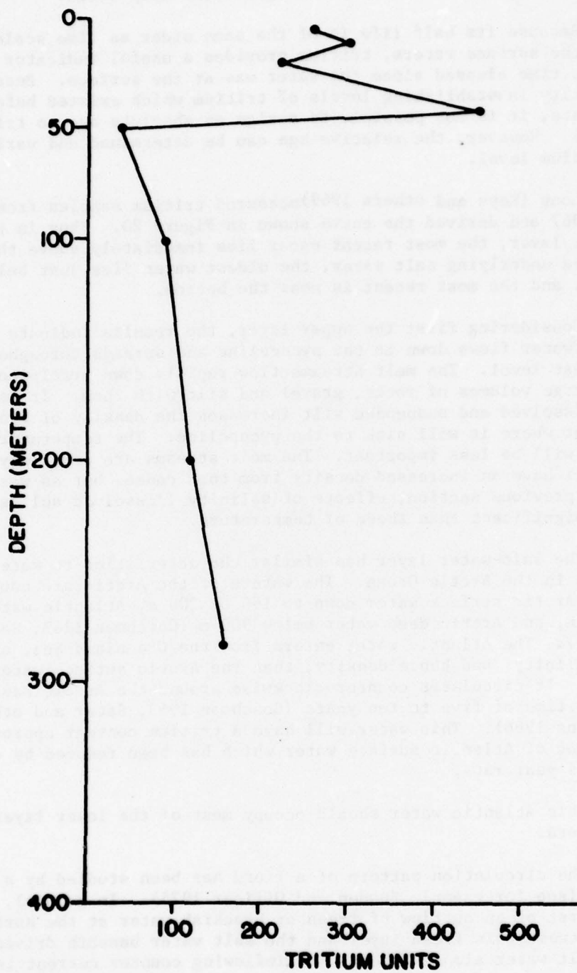
Fig. 20: Tritium concentration in tritium units, as a function of depth. Age of the water varies inversely as tritium concentration.
