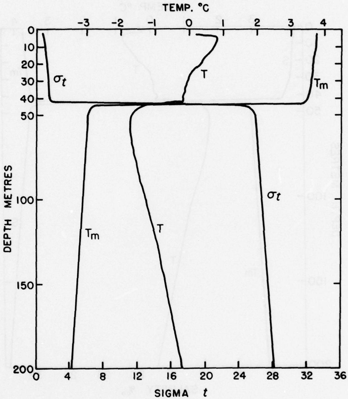
Fig. 18: Density in terms of sigma t (CGS units), Temperature (T), and Temperature of maximum density ( T_m ) as functions of depth.
