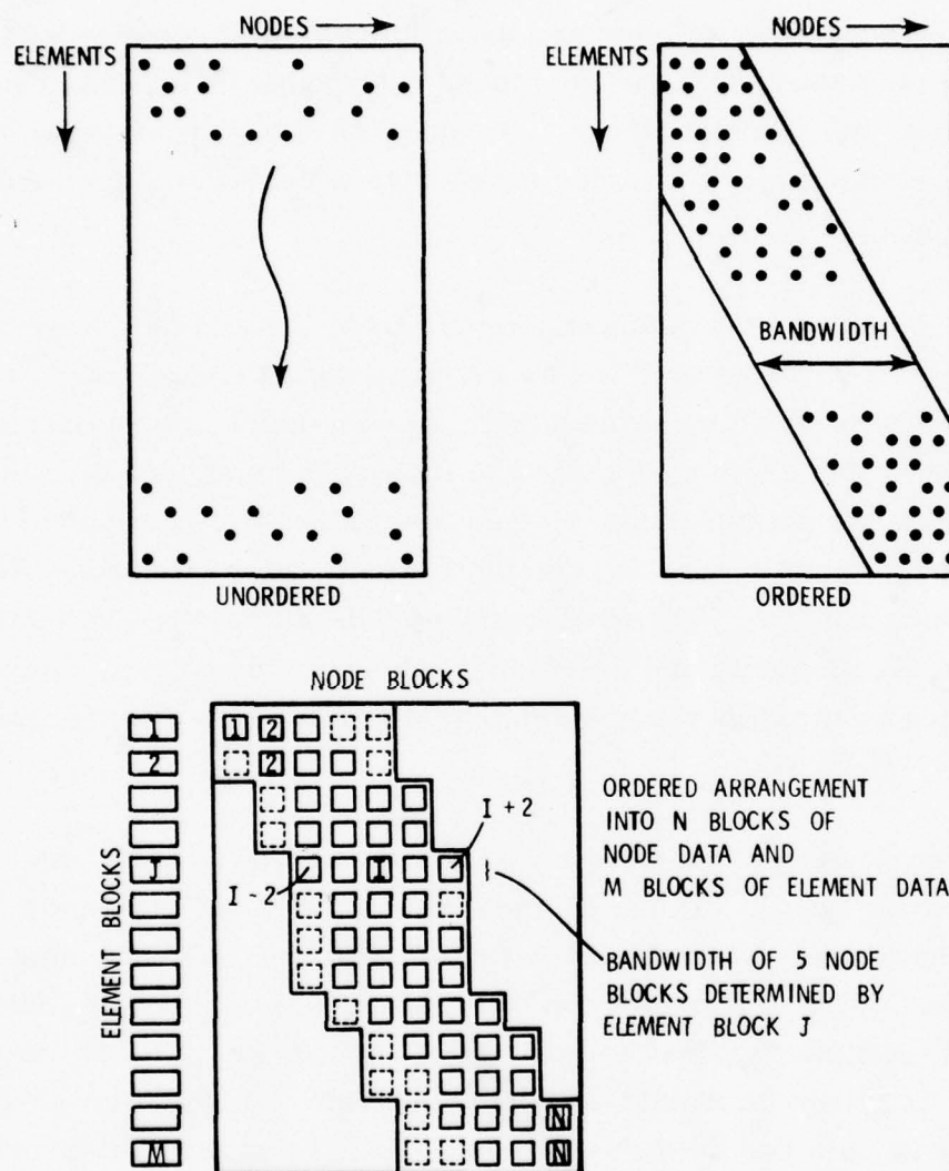
Figure 11. Bandwidth Representation for Node-Element Connectivity
