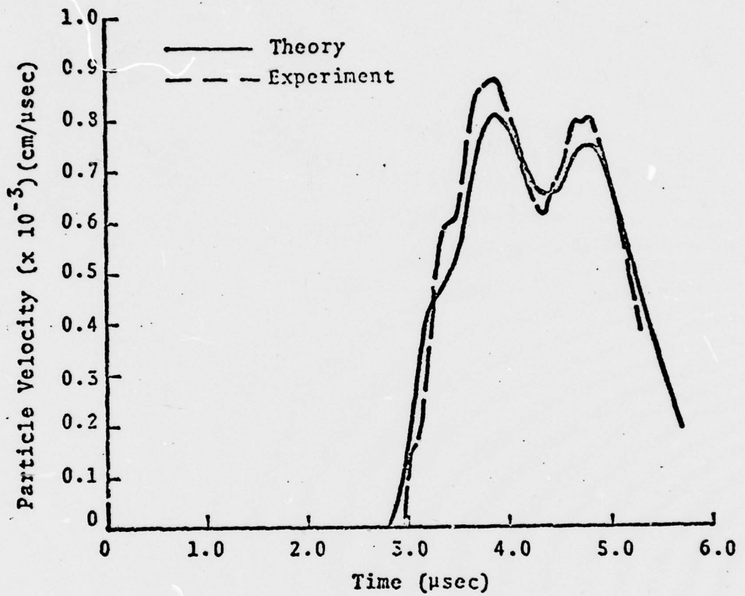
Fig. 18. Comparison of theory with experiment No. 7.
