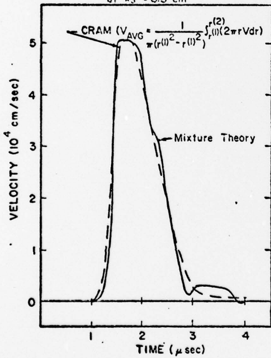
VELOCITY IN PHENOLIC SHEATH (MATERIAL 2) at x_3 = 0.5 cm
