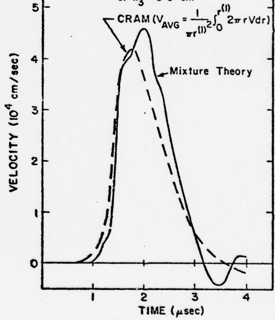
VELOCITY IN RADIAL FIBER (MATERIAL 1) at x_3 = 0.5 cm
