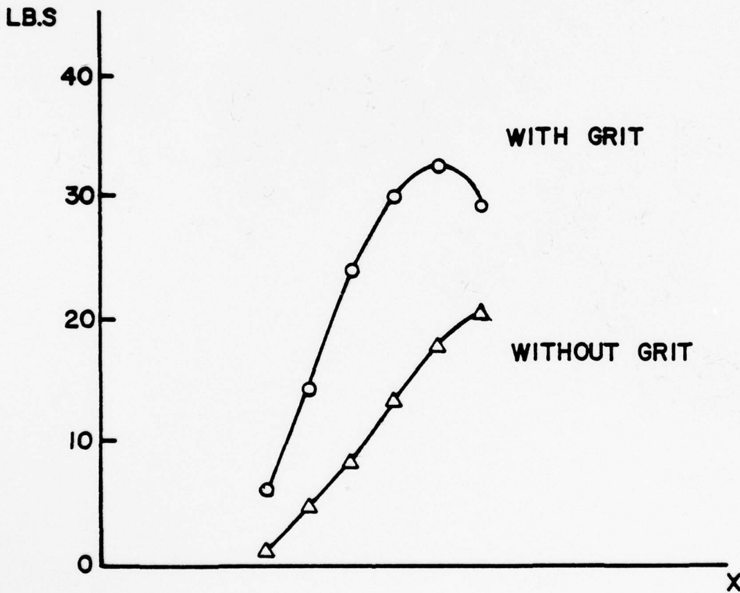
FIGURE 15 SIDE FORCE DISTRIBUTION ( M=0.3 , Re=2 \times 10^6 , \alpha=45^\circ )
