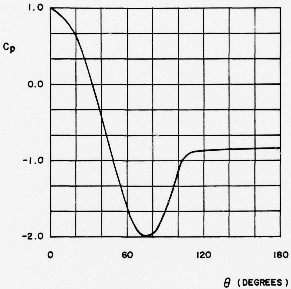
FIGURE 7 PRESSURE DISTRIBUTION CURVE FOR ROSHKO'S CIRCULAR CYLINDER
