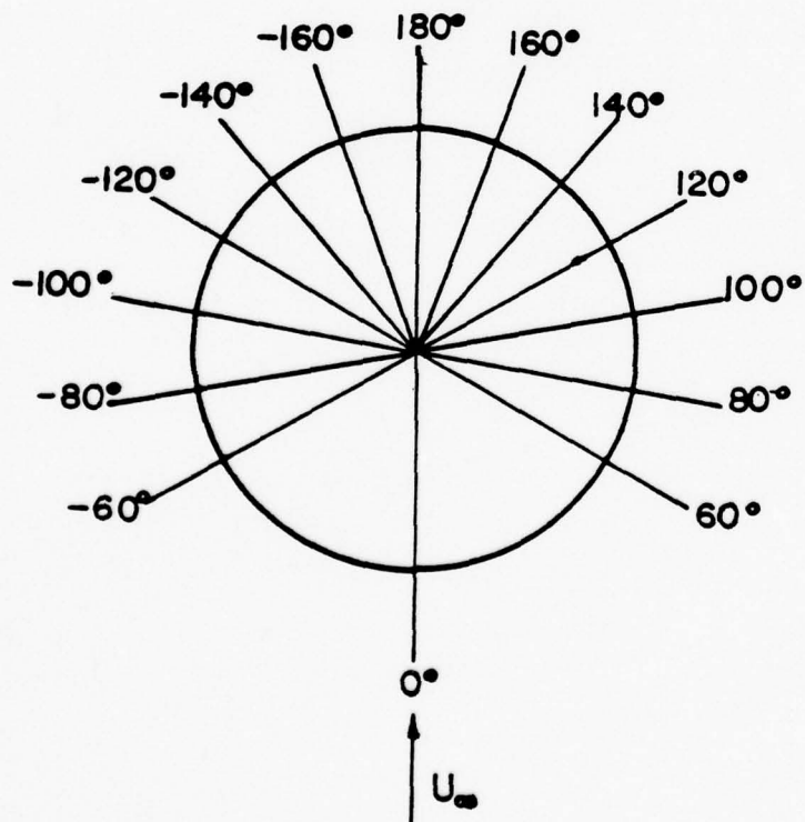
FIGURE 12 LOCATION OF PRESSURE TAPS ON AFFDL MODEL
