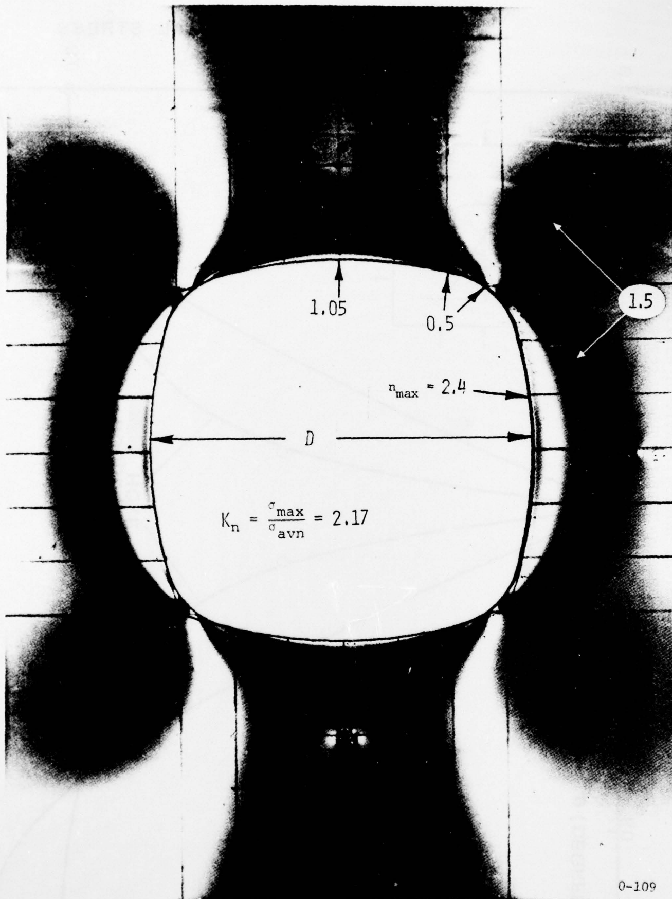
FIG. 7 STRESSES AT THE BOUNDARY OF A DOUBLE BARREL HOLE IN A LARGE PLATE ( \frac{D}{W} = 0.163 ) SUBJECTED TO UNIAXIAL LOAD
