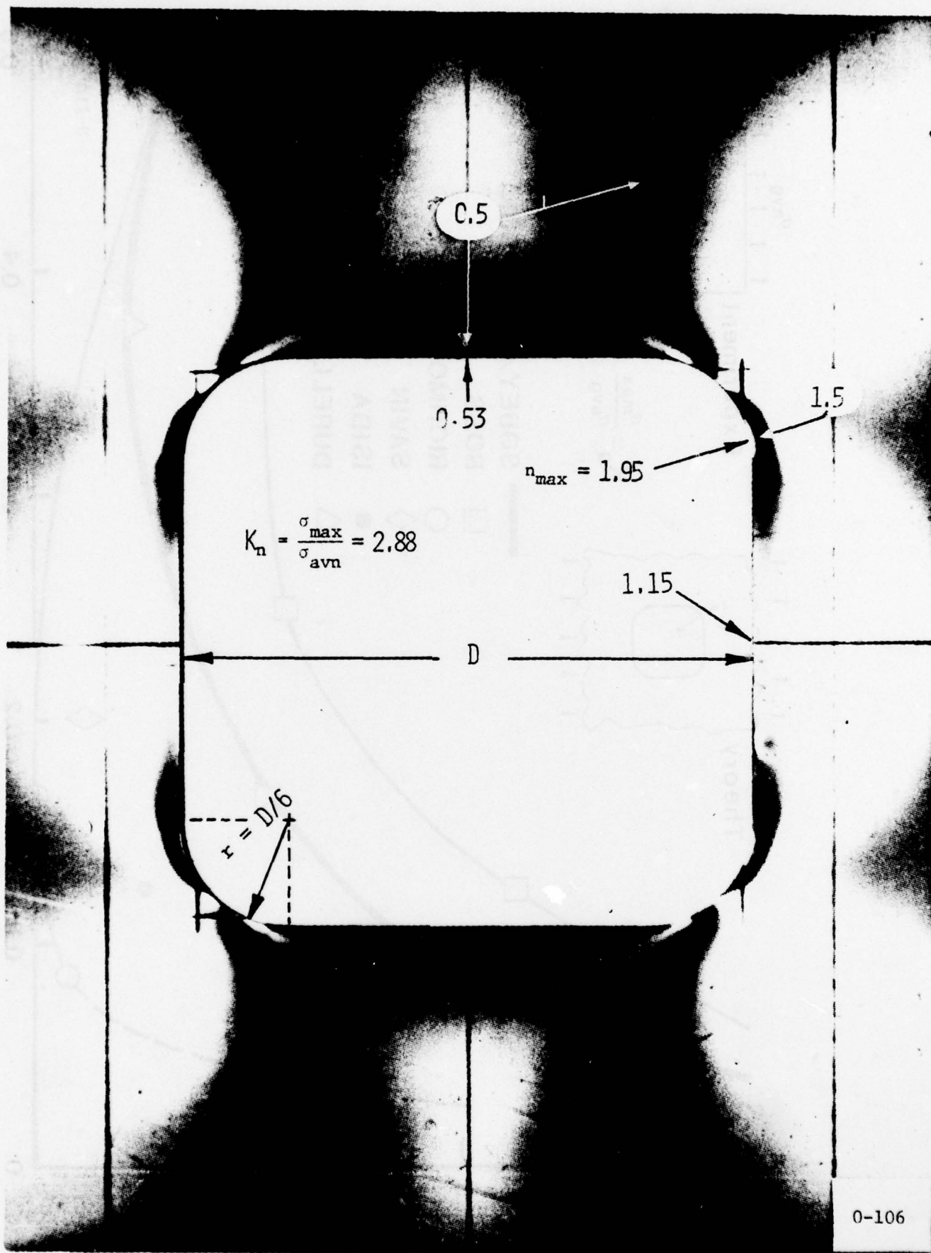
FIG. 2 STRESSES AT THE BOUNDARY OF A SQUARE HOLE WITH A ROUNDED CORNER ( r=D/6 ) IN A LARGE PLATE ( \frac{D}{W} = 0.136 ) SUBJECTED TO UNIAXIAL LOAD
