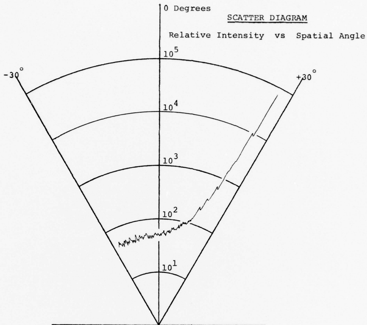
Figure 4. Plot of relative scatter intensity for mirror #449. Point of incidence at location 3. Angle of incidence = 30 degrees.
