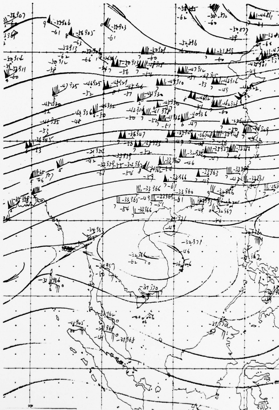
Fig. 20. ROHK 300 mb streamline analysis, 0000GMT 3 December 1974.
