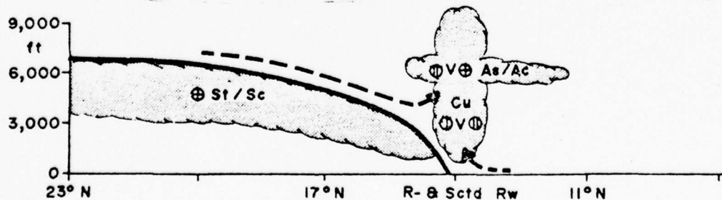
Figure 4. Western South China Sea Winter-Season Frontal Sequence Model, North-South Vertical Cross Section (Low stratiform clouds representative of Tonkin Gulf inshore waters and coastal areas).
