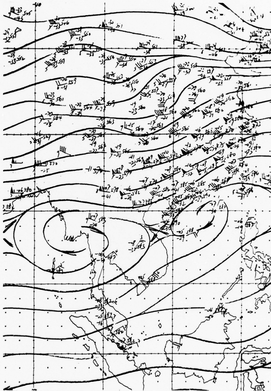
Fig. 49. ROHK 500 mb streamline analysis, 0000GMT 10 December 1974.
