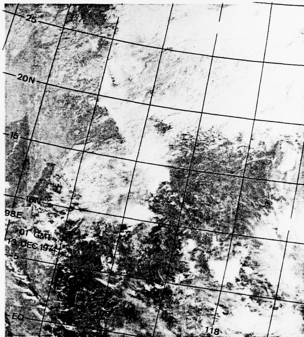
Fig. 60. DMSP VHR PHOTOGRAPH, 0100GMT 13 DECEMBER 1974.
