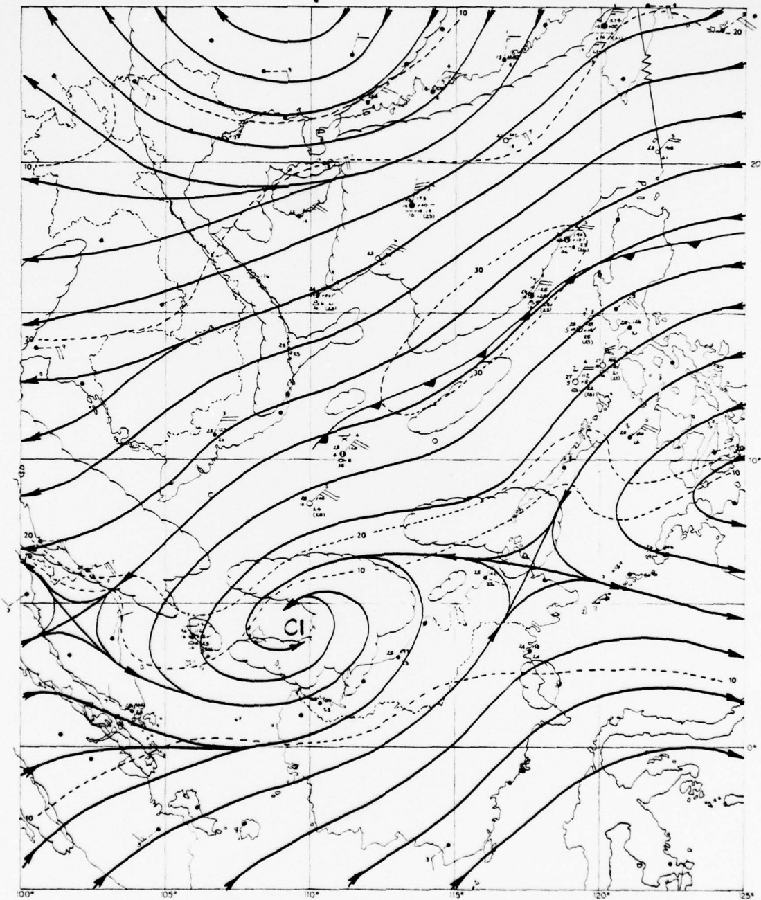
Fig. 30. 850 mb/surface streamline-isotach analysis, 0000GMT 6 December 1974.
