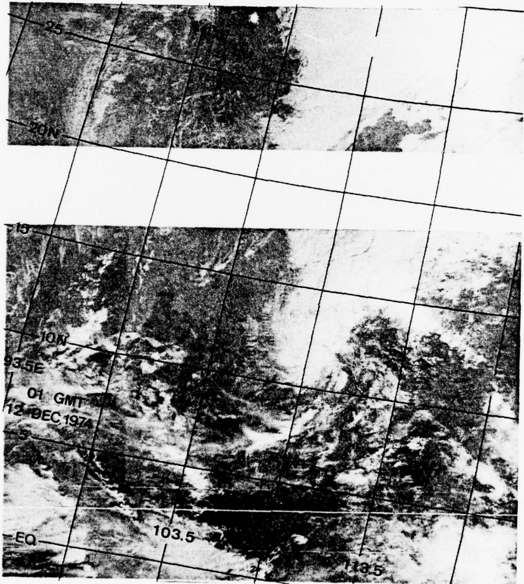
Fig. 59. DSP VHR PHOTOGRAPH, 0100GMT 12 DECEMBER 1974.
