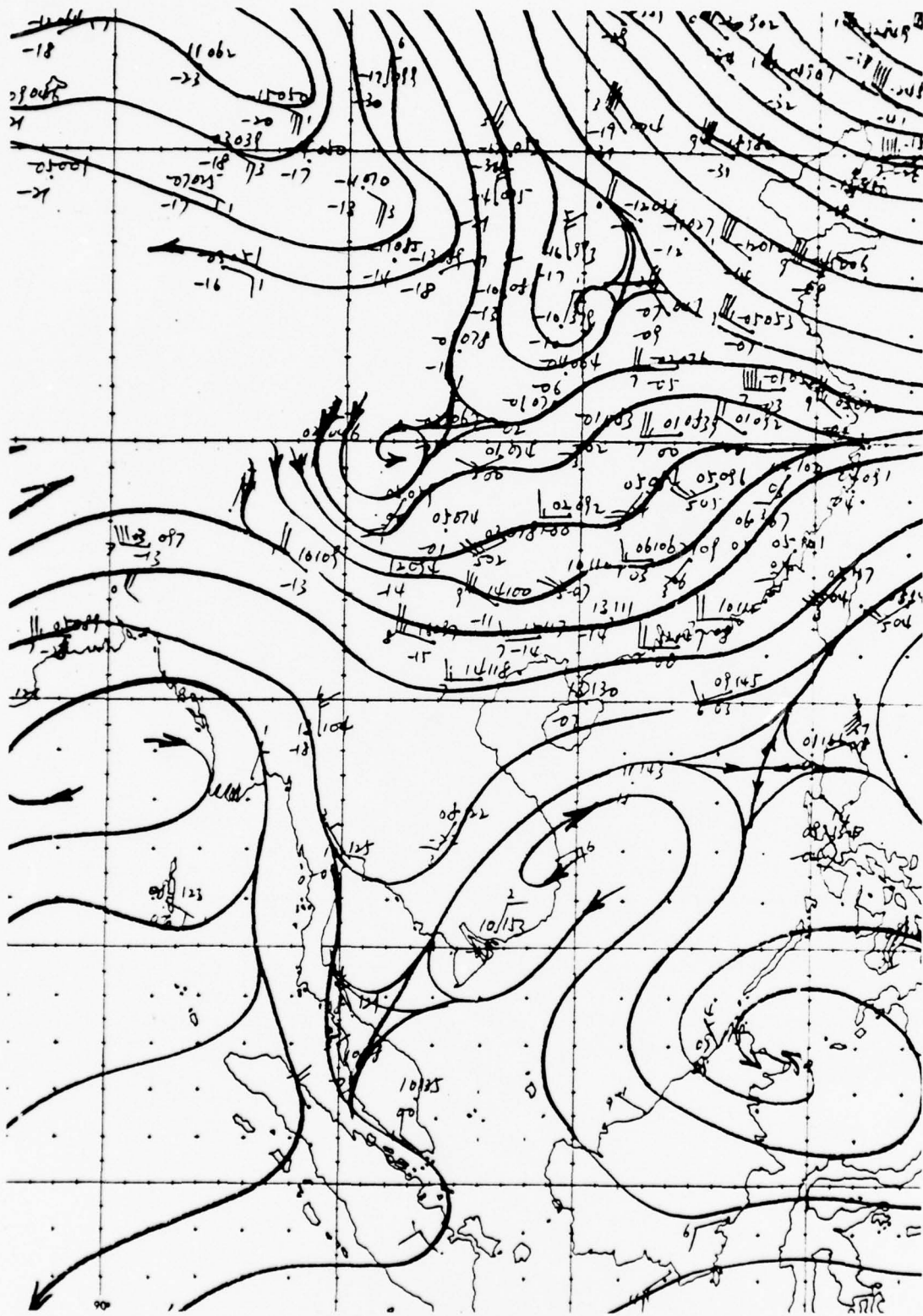
Fig. 9. ROHK 700 mb streamline analysis, 0000GMT 3 December 1974.
