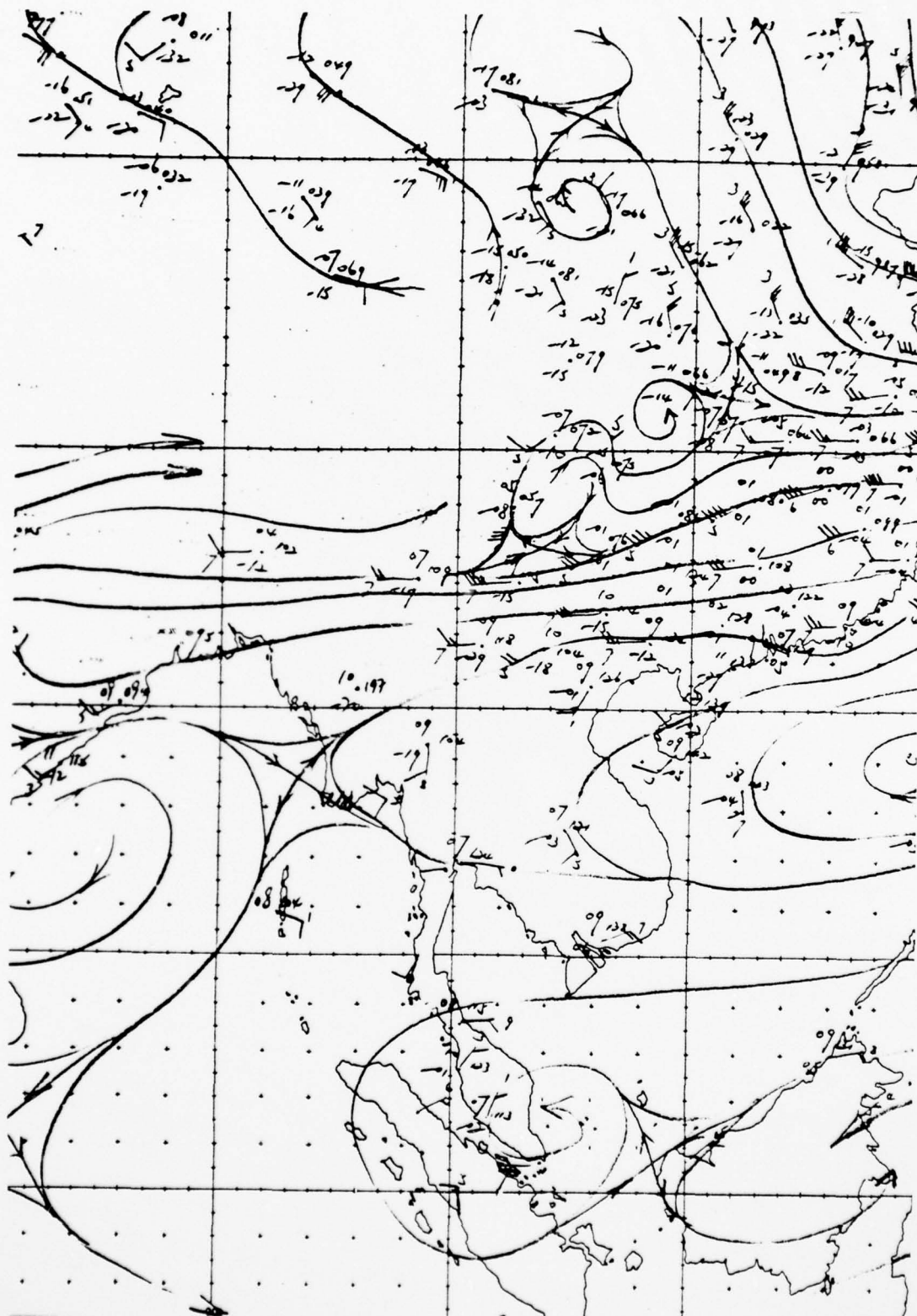
Fig. 25. ROHK 700 mb streamline analysis, 0000GMT 5 December 1974.
