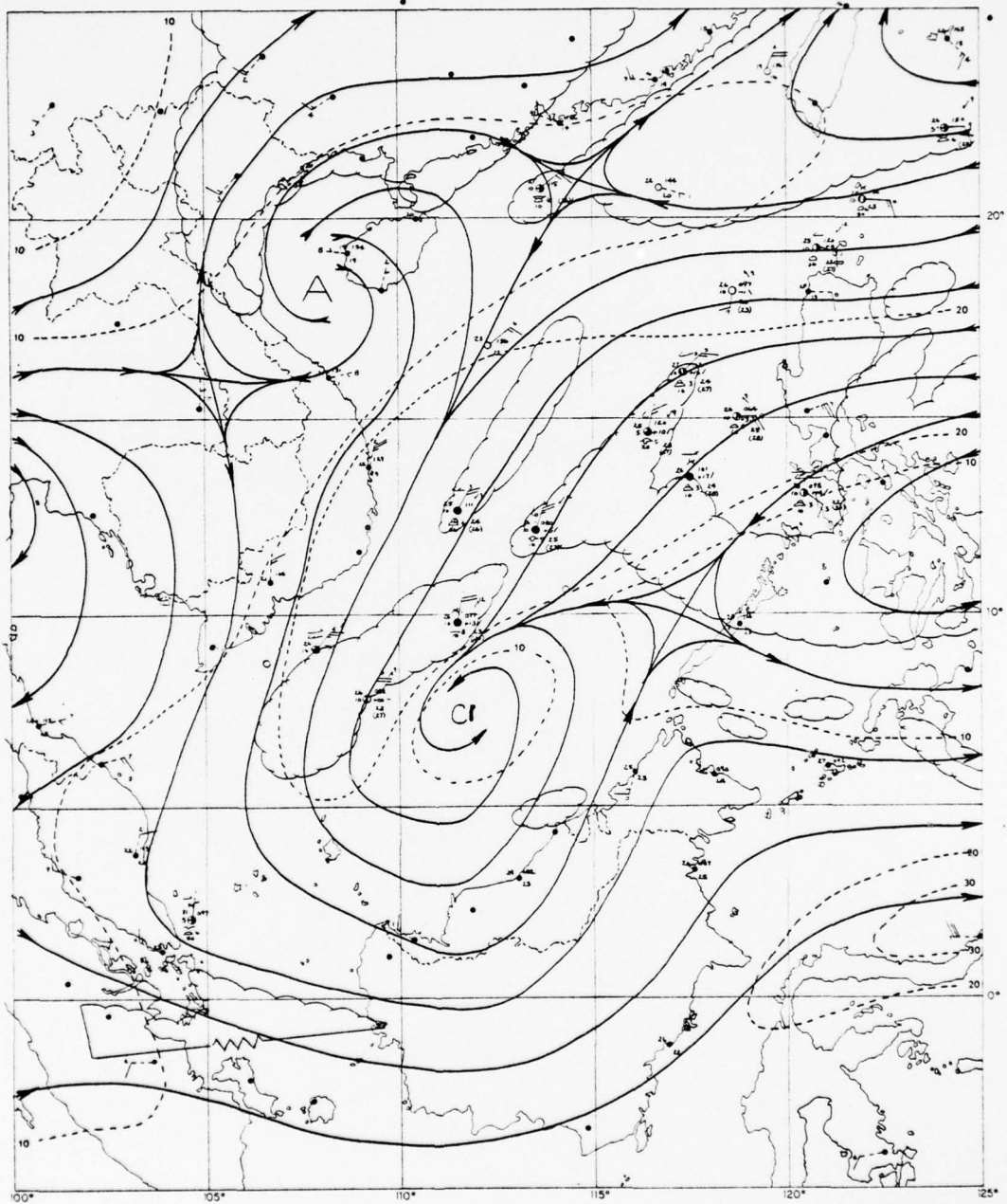
Fig. 39. 850 mb/surface streamline-isotach analysis, 0000GMT 8 December 1974.
