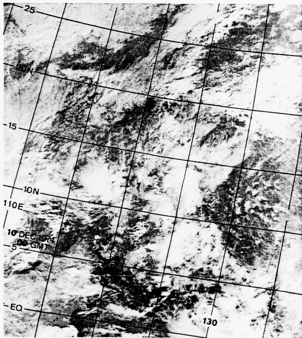
Fig. 50. DMSP VHR PHOTOGRAPH, 0000GMT 10 DECEMBER 1974.
