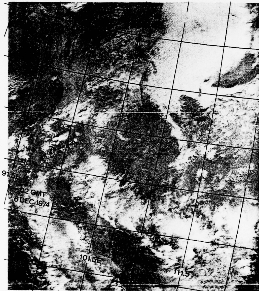
Fig. 32. D'SP VHR PHOTOGRAPH, 0200GMT 6 DECEMBER 1974.
