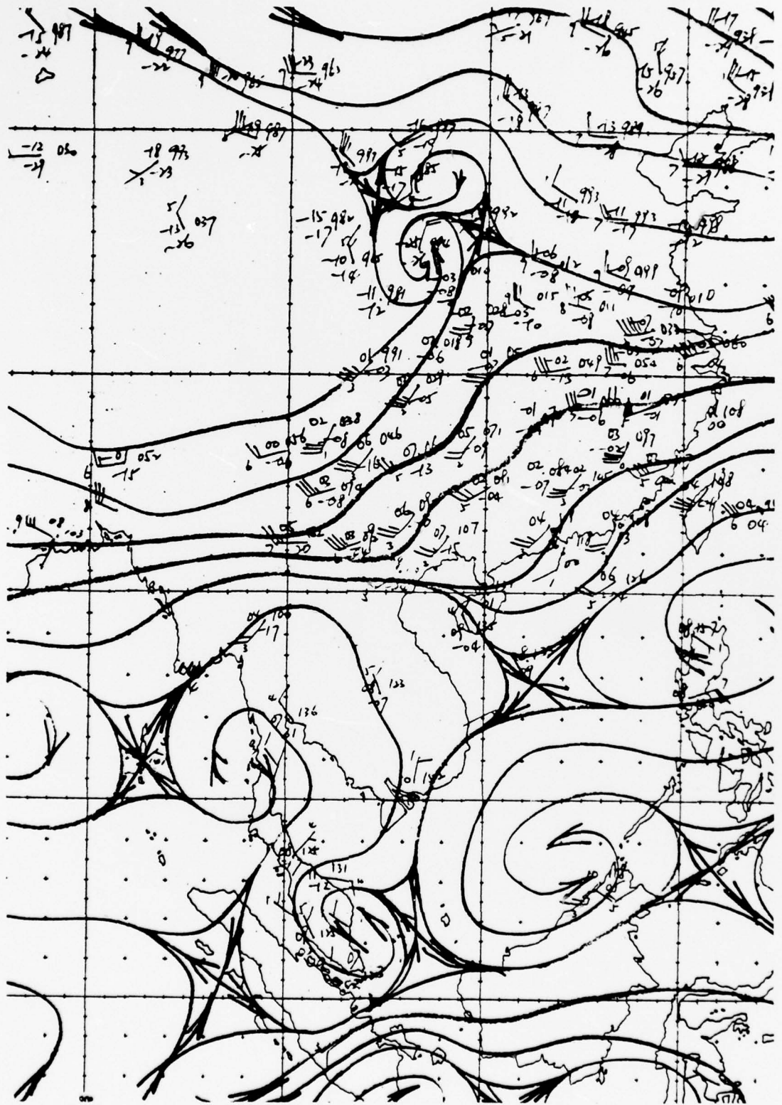
Fig. 41. ROHK 700 mb streamline analysis, 0000GMT 3 December 1974.
