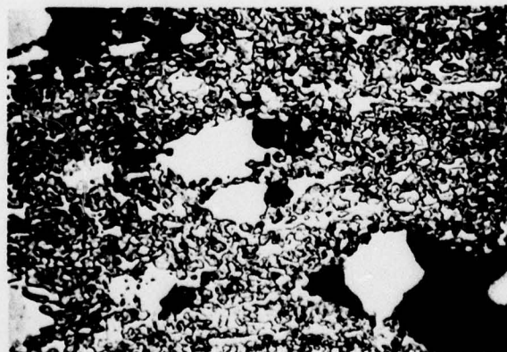
Figure 13. Shown above are further examples of the cavitation described in Figure 12. As may be seen from the center micrograph, in areas free from carbides of > \sim 10 \mu\text{m} in size, there is no cavitation.
