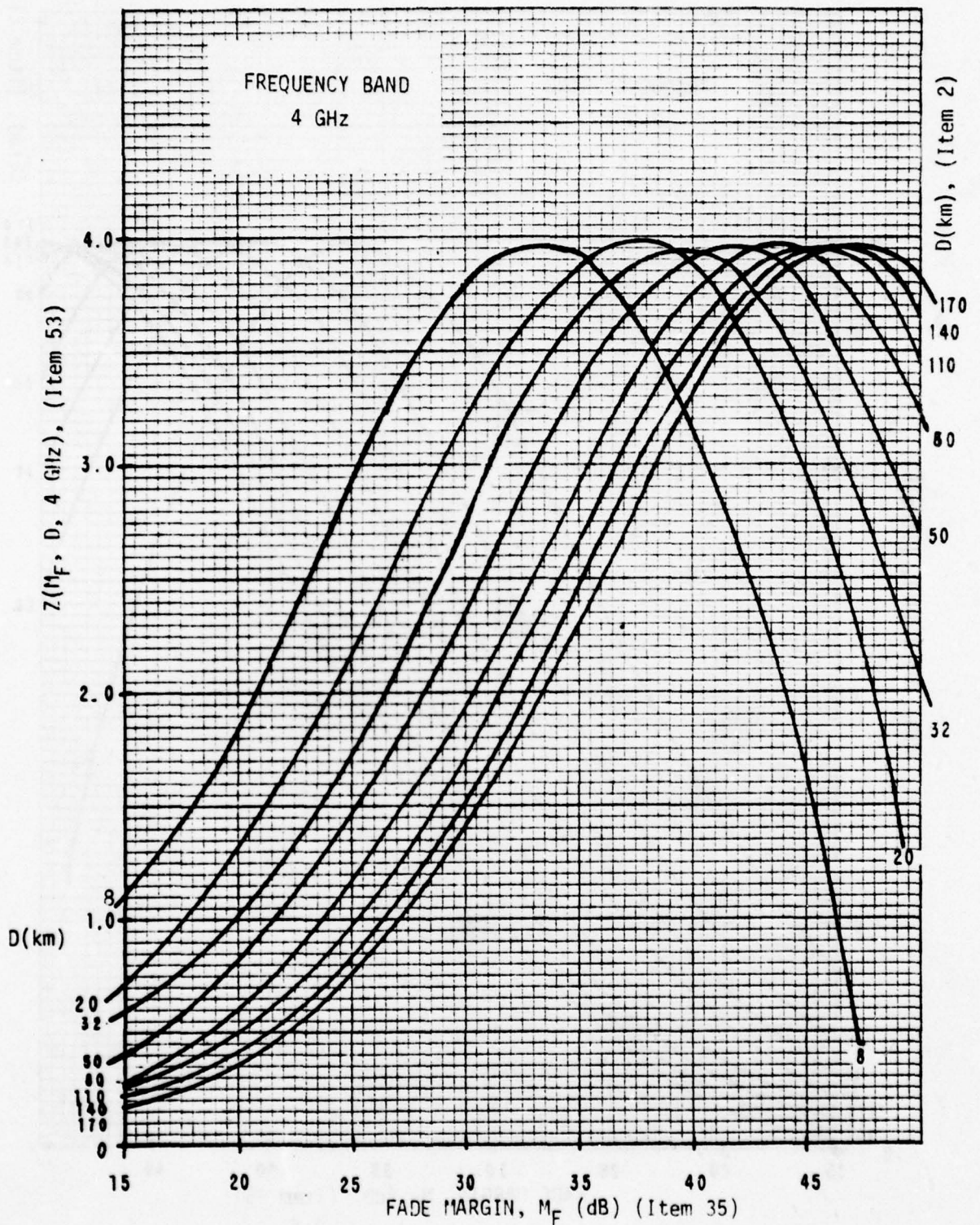
Figure B-3b. Z Factor as a Function of Fade Margin and Path Length, for the 4 GHz Frequency Band
