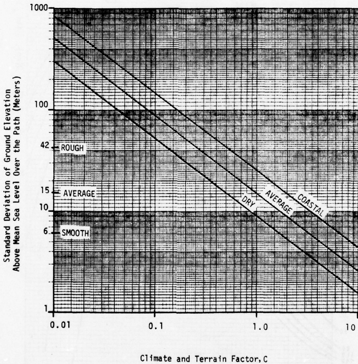
Figure B-2. C Factor as a Function of Terrain Roughness and Climate
