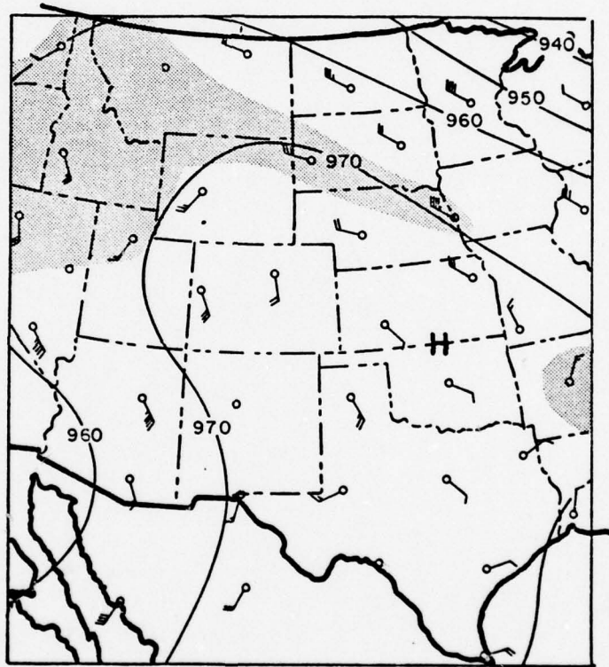
Figure 2-3 300 millibar analysis 1 August 1976 0000 GMT (from Maddox, et al., 1977). Dewpoint depression \leq 10^{\circ}\text{C} is shaded.
