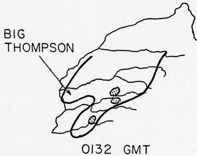
Figure 4-4 Limon radar echoes with drainage basins superimposed 1 August 1976 0132 GMT. Solid line encloses VIP levels 1 and 2. VIP level 3 is shaded.
