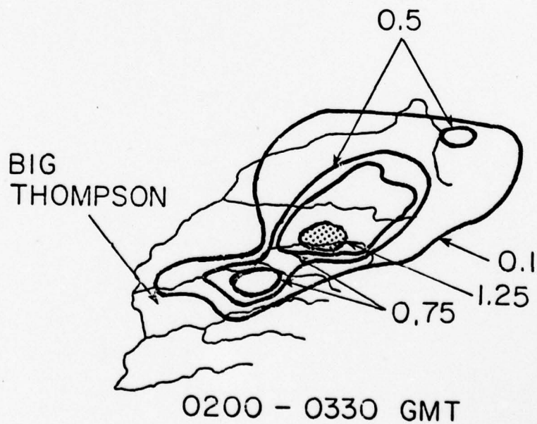
Figure 4-17 Satellite-derived half-hourly isohyet analysis (in), 0200-0330 GMT, 1 August 1976.
