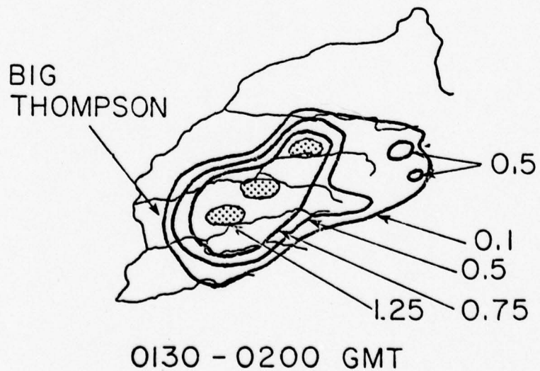
Figure 4-15 Satellite-derived half-hourly isohyet analysis (in), 0130-0200 GMT, 1 August 1976.
