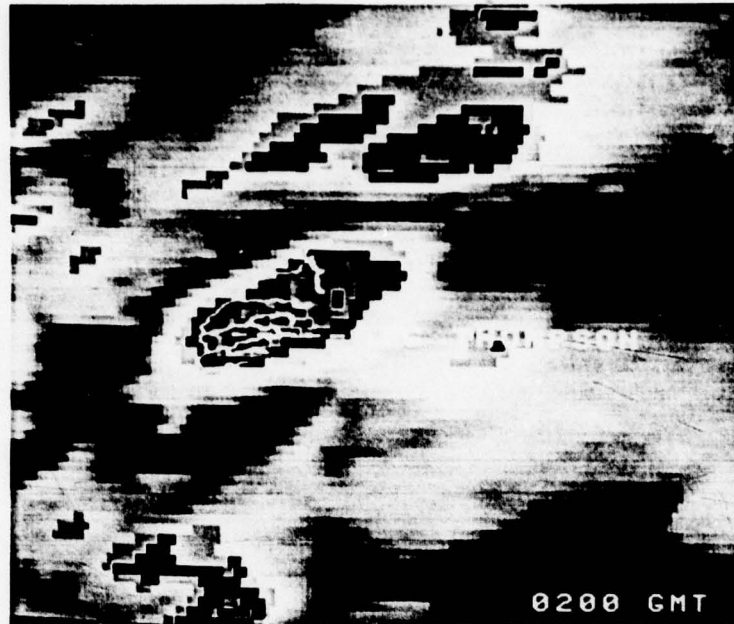
Figure 4-14 Infrared image 1 August 1976 0200 GMT with drainage area overlay.
