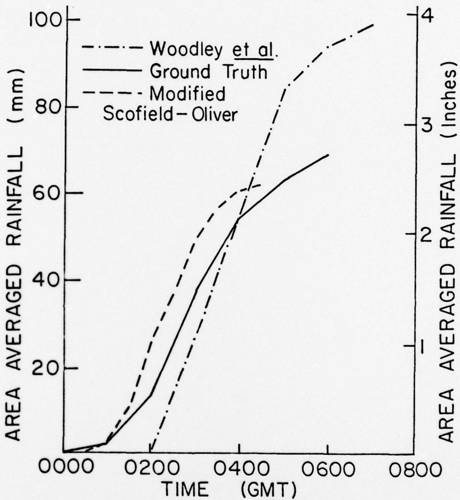
Figure 4-21 Cumulative area-averaged rainfall for the Big Thompson Basin on 1 August 1976.
