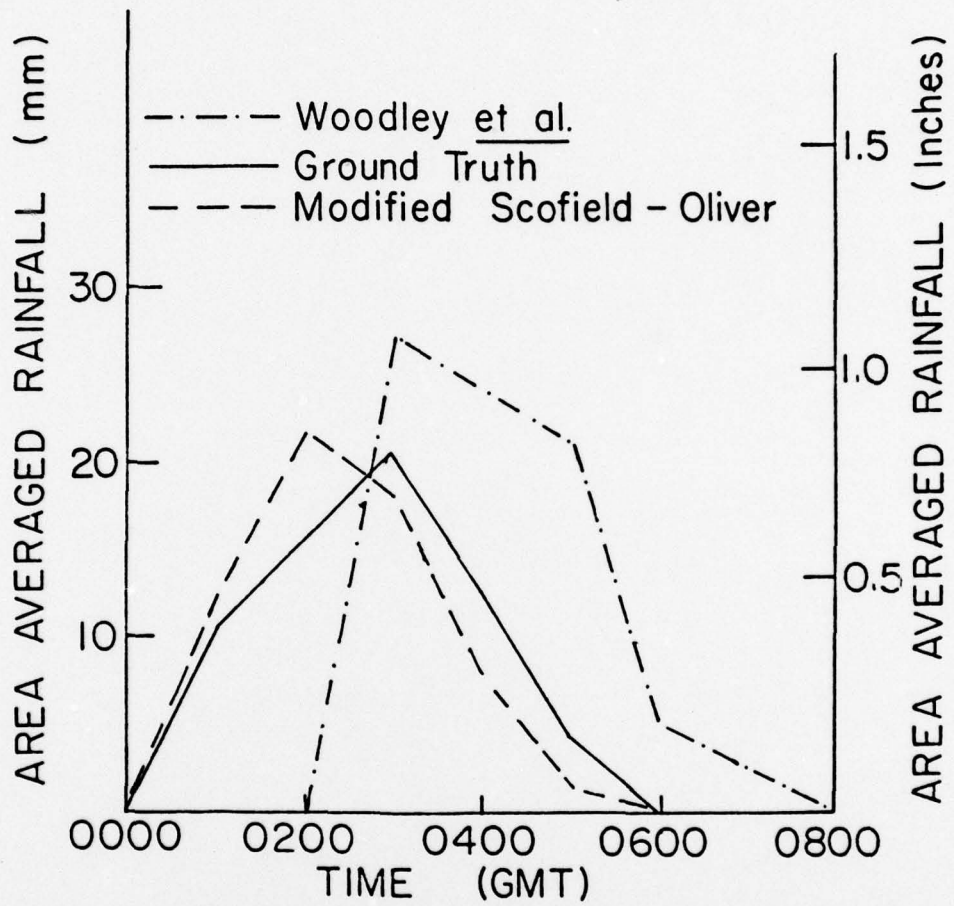
Figure 4-22 Hourly area-averaged rainfall for the Big Thompson, Little Thompson and St. Vrain Drainage Basins on 1 August 1976.
