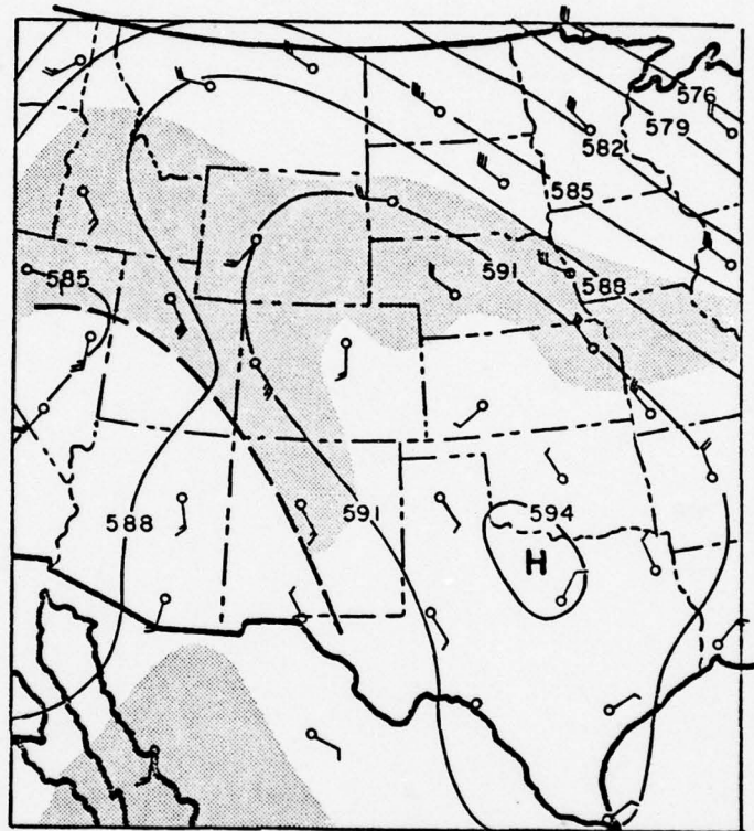
Figure 2-2 500 millibar analysis 1 August 1976 0000 GMT (from Maddox, et al., 1977). Dewpoint depression \leq 6^{\circ}\text{C} is shaded.
