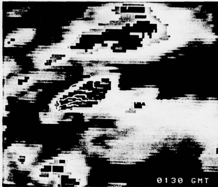
Figure 4-12 Infrared image 1 August 1976 0130 GMT with drainage area overlay.
