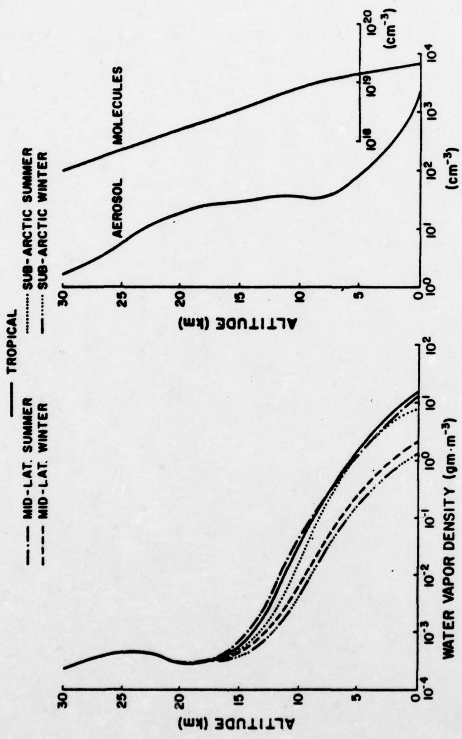
Figure 5. Water vapor density profiles in the model atmosphere.
