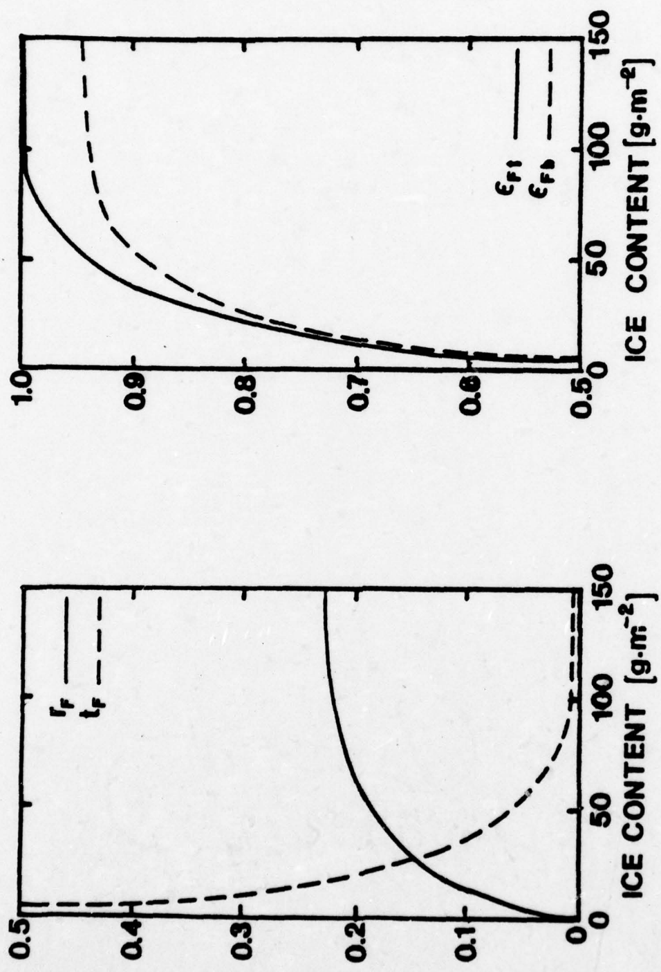
Figure 16. Infrared radiative properties of a cirrus cloud.
