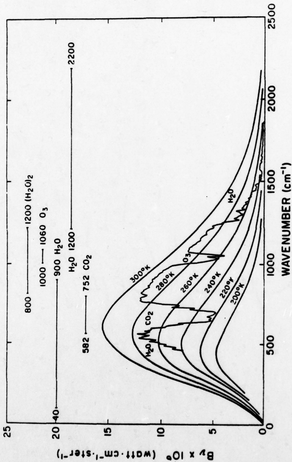
Figure 2. Infrared spectrum.
