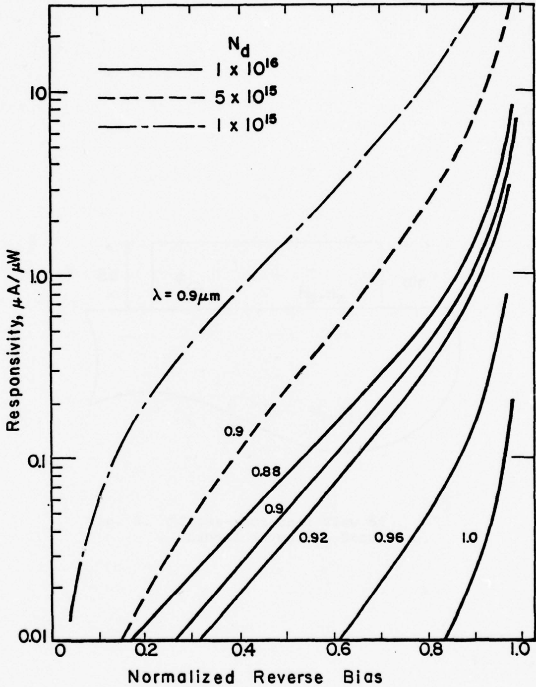
Fig. 4. Calculated Responsivity as a Function of Bias, Wavelength, and Doping Level for a 100 \mu\text{m} Long EAP Detector.
