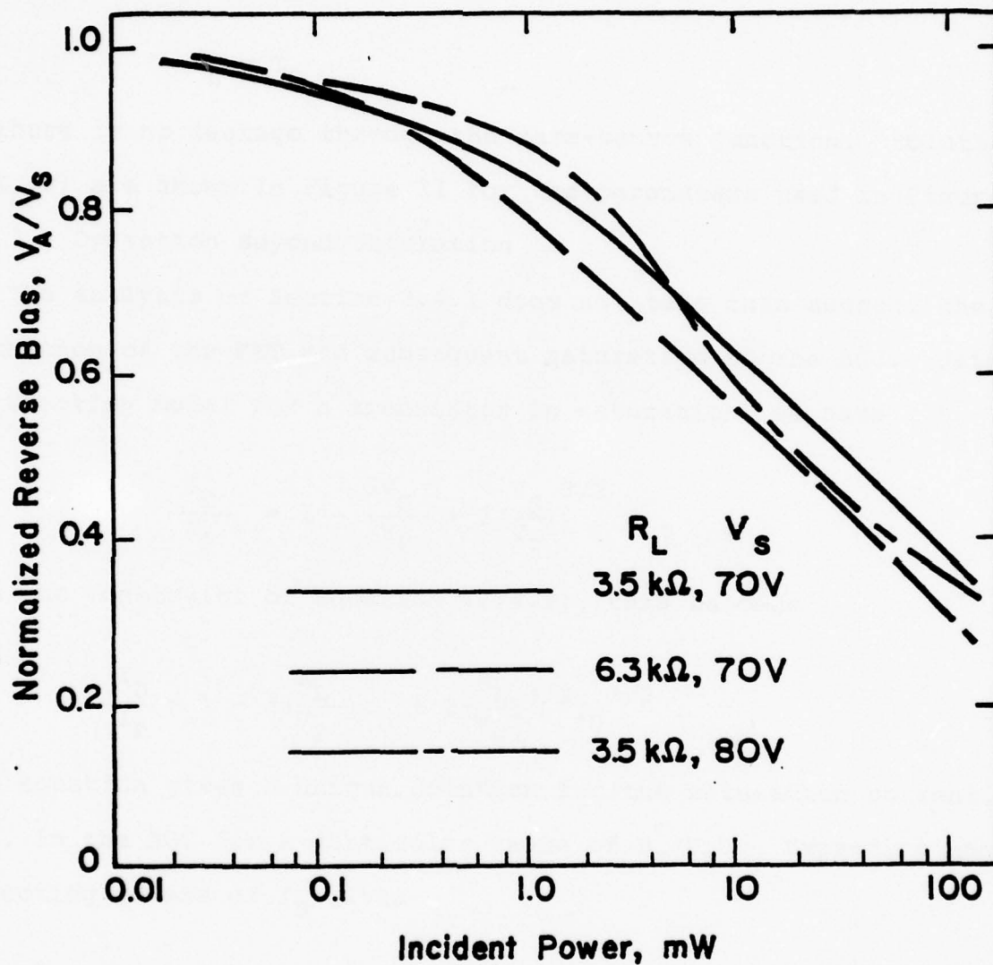
Fig. 10. Detector Bias Voltage Dependence on Incident Power for Various Values of Initial Bias and Load Resistor.
