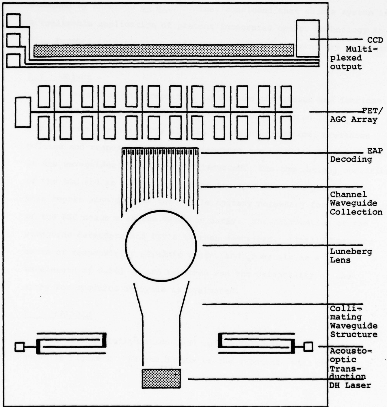
Fig. 1. A Hypothetical GaAs Ioc for real-time Spectrum Analysis.
