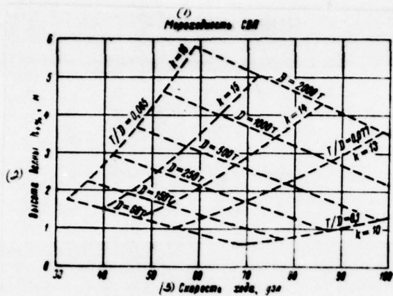
Fig. 192. Seaworthiness of promising SVP (normal accelerations w \leq 0.5 g).
