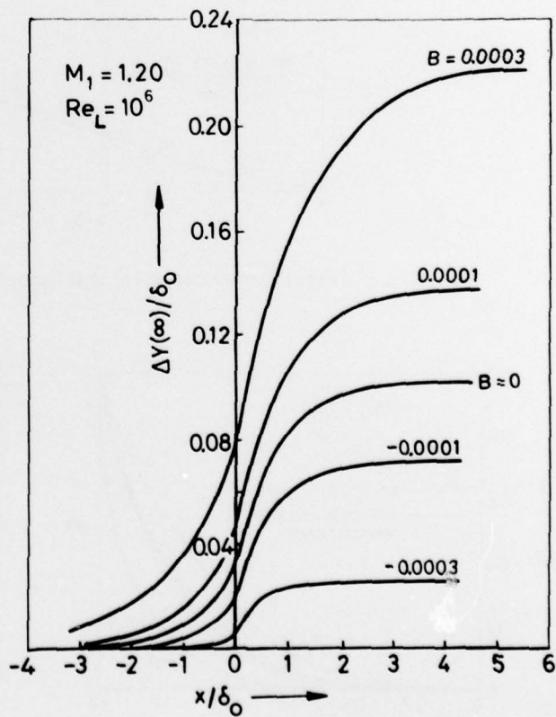
Fig. 13 Interactive Displacement Thickness Distributions with Suction or Blowing
