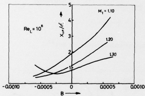
Fig. 12 Upstream Influence vs. Mass Transfer Parameter
