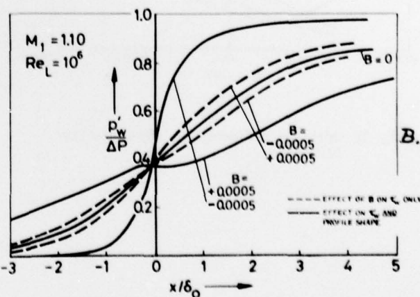
Fig. 10 Influence of the Mass Transfer Effect-Model on the Interaction Solution
