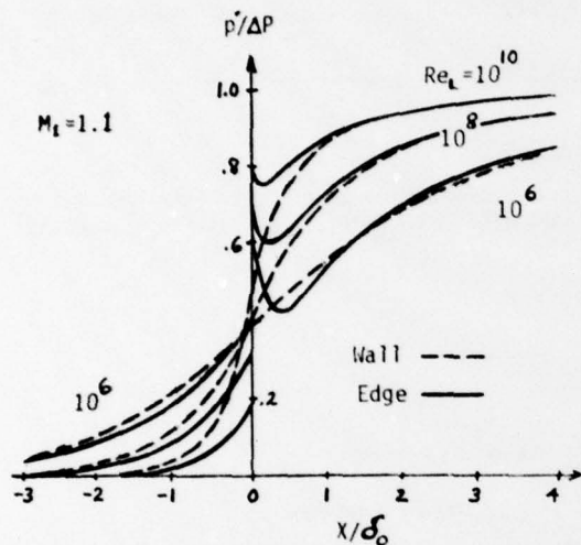
Fig. 3 Reynolds Number Influence on Interaction Pressure Field
