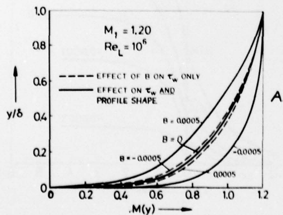
Fig. 10 Influence of the Mass Transfer Effect-Model on the Interaction Solution
