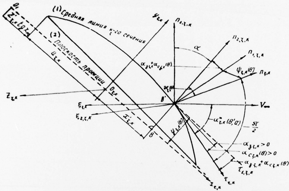
Fig. 2. Coordinate system of wing section. KEY: (1) Middle line of k -th section, (2) Projection plane.
