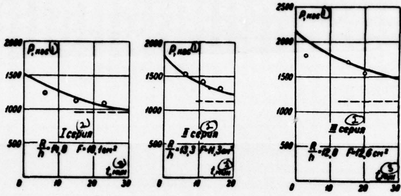
Fig. 5.8. The theoretical curve of prolonged critical force according to expression (5.13.1) and experimental points (o) ( \bar{G} = 6000 ; \tilde{Q} = 85 ).
