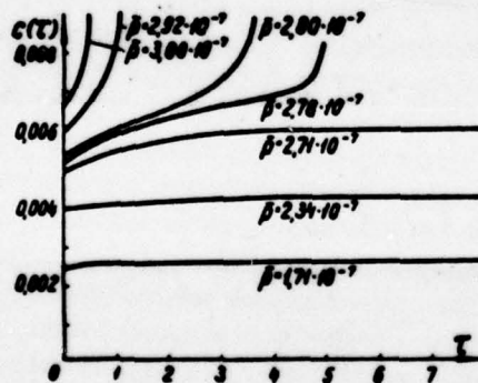
Fig. 5.3. Diagrams c-\tau with transverse load \bar{p} of different intensity (results are calculated with the aid of BESH-2).
