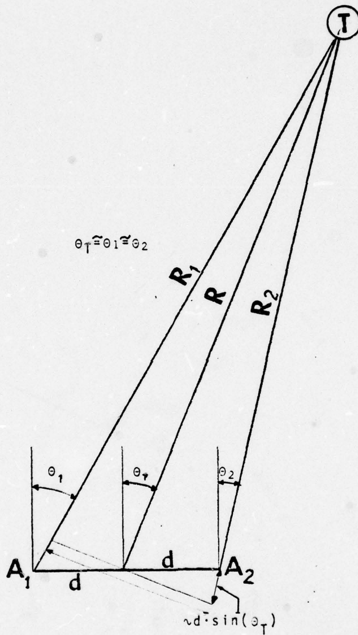
Figure 2.2-5. Wavefront relationships.
