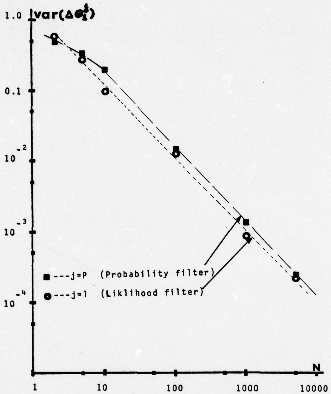
Fig. 5.2-9. The variance of \theta_1 as a function of the sample's number.
