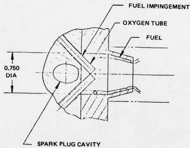
ORIGINAL DESIGN
