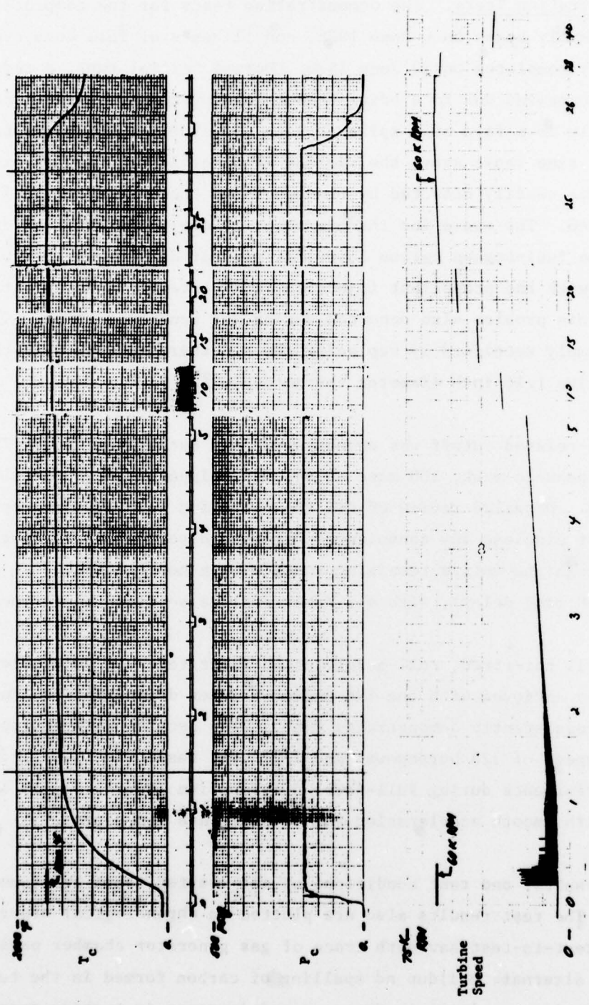
Figure 130. IPU Engine Starter Demonstrator Performance During Full-Power Acceleration (Run 13.01)
