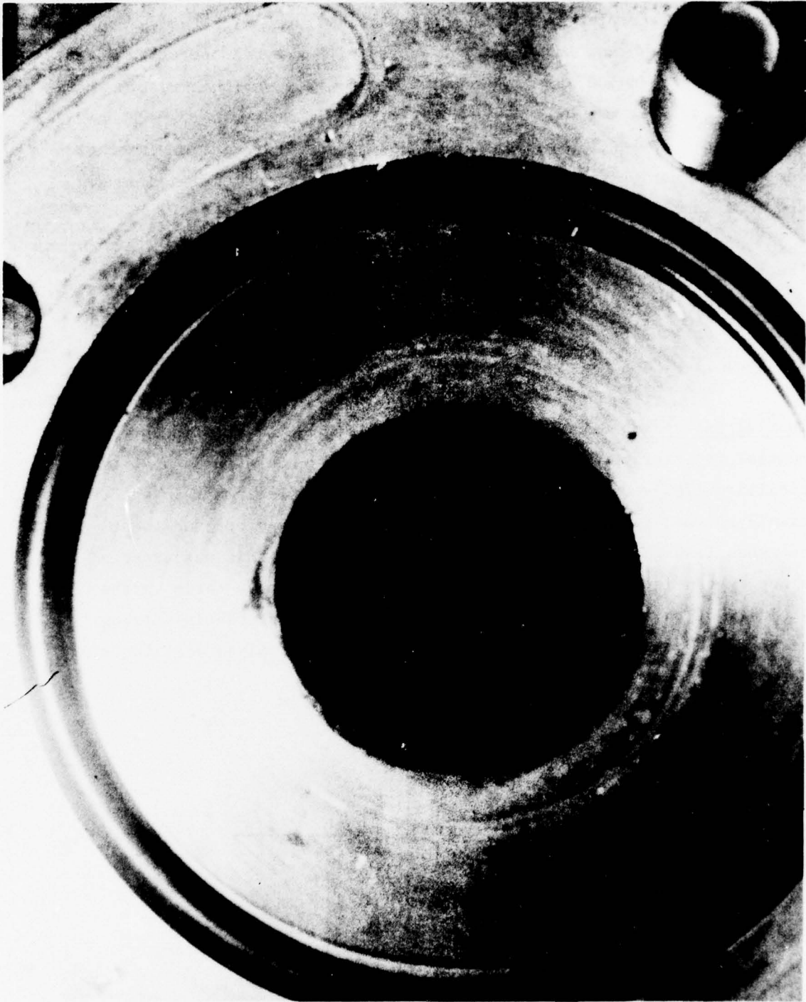
Figure 45. Carbon Buildup in Combustor Body After Triplet Injector First Test Series
