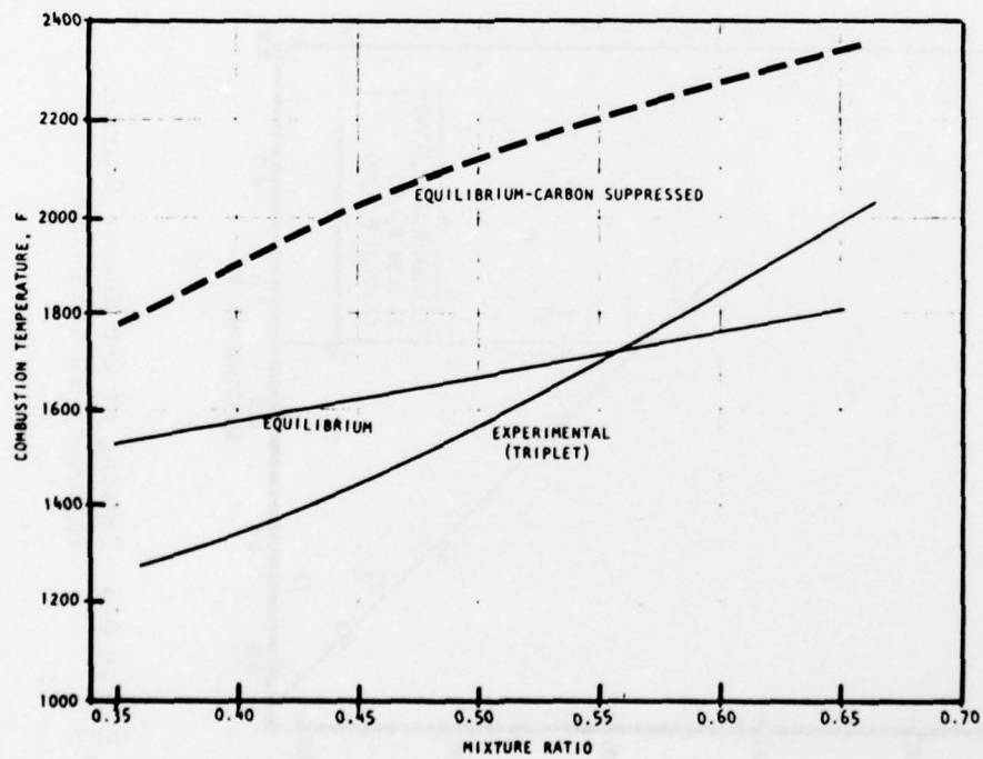
Figure 63. Oxygen/JP-4 Combustion Temperature
