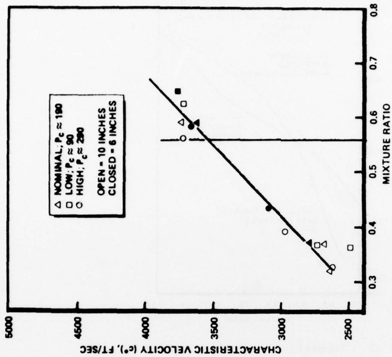
Figure 60. Testing of 2-D Recess Coaxial Injector, 10-Inch Combustor
