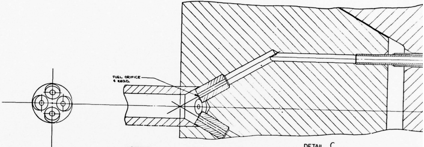
DETAIL C 10X SIZE
