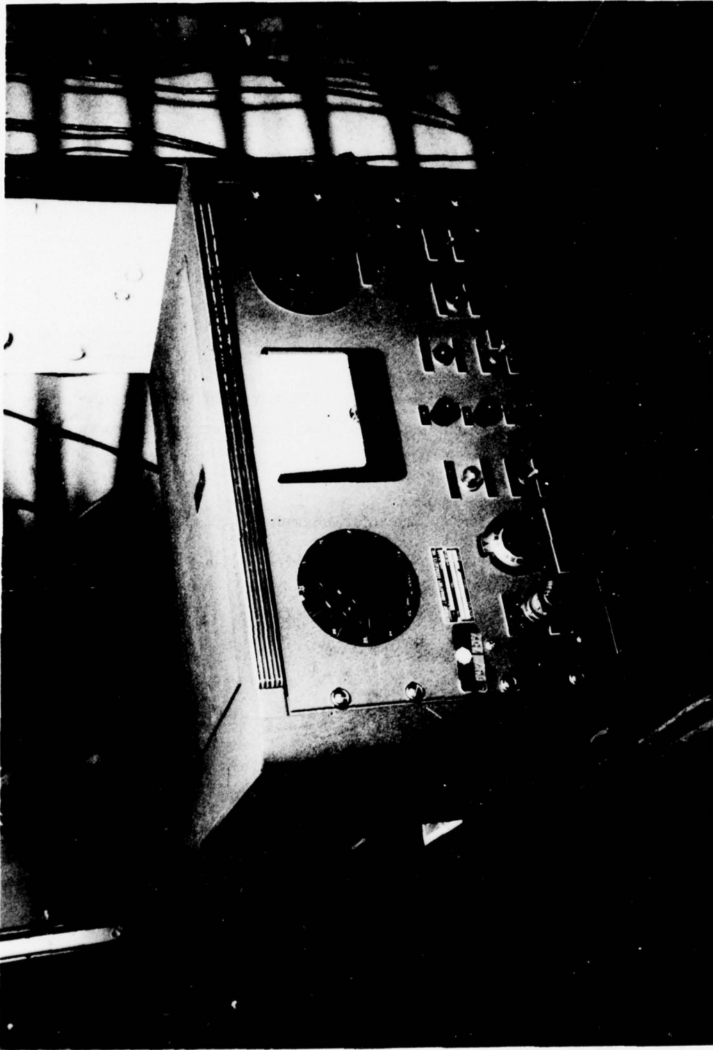
Figure 5. Variable Energy Spark Exciter
