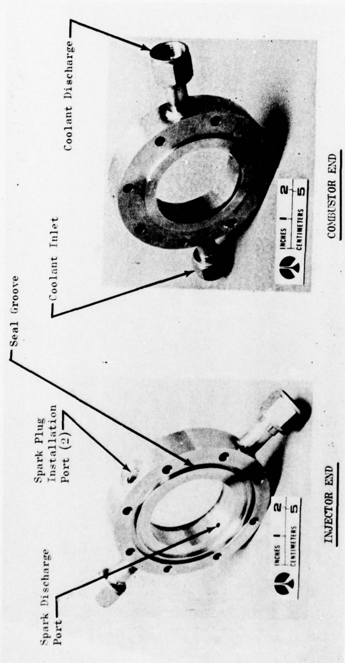
Figure 31. Sparkplug Wafer
