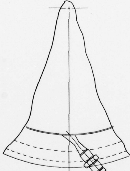
SECTION C-C ROTATED 32°
