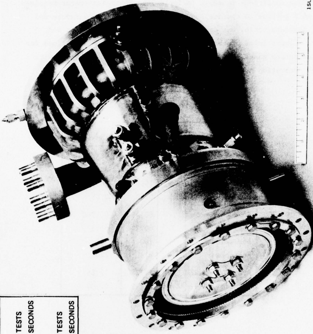
Figure 107. Mark 44 F Fuel Turbopump
