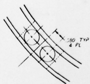
VIEW D SCALE 8:1
