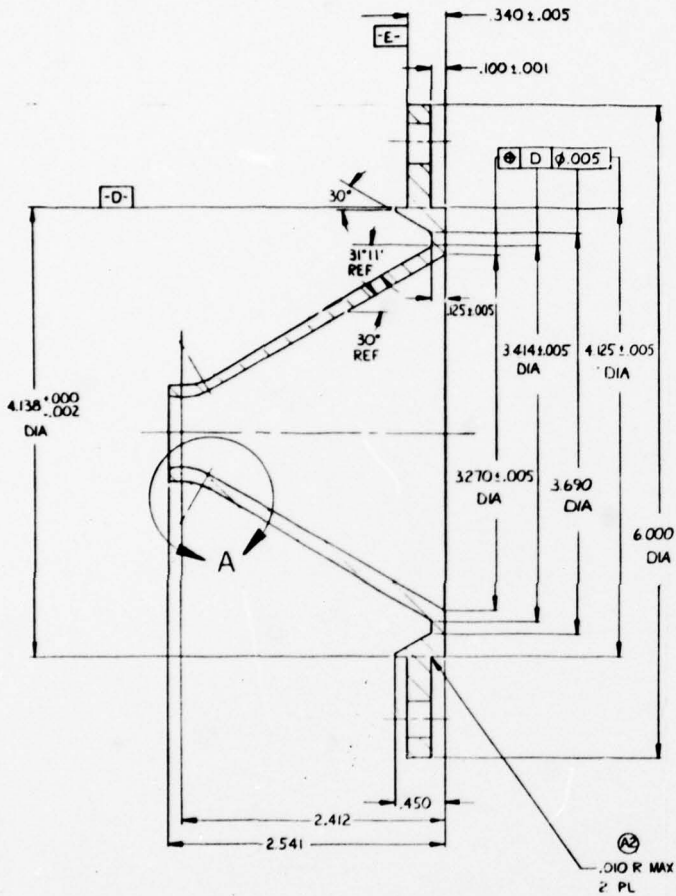
SECTION B-B
