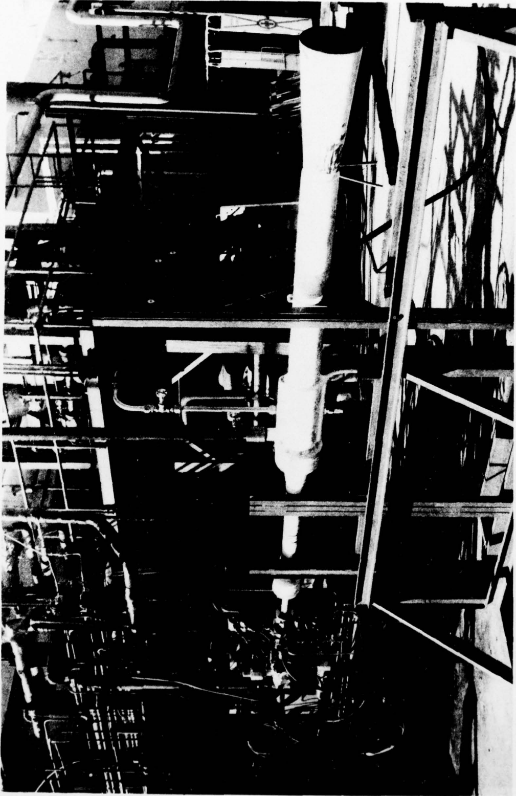
Figure 38. Low-Power Gas Generator High-Altitude Ignition Test Installation
