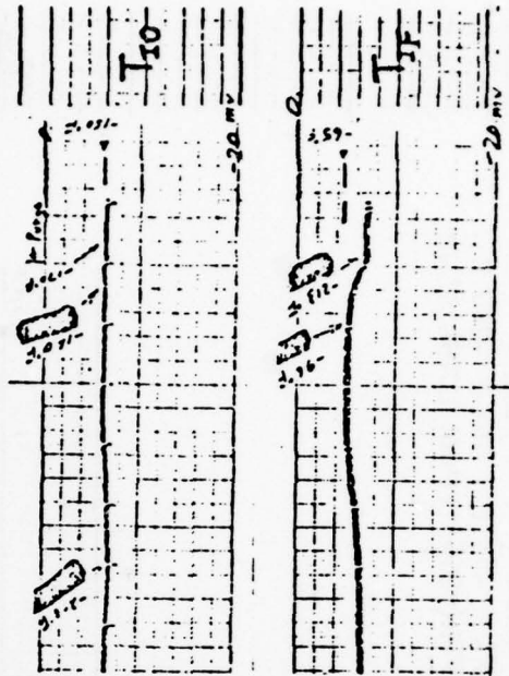
Figure 77. Ignition Diagnostics for Cold Propellants (JP-4 = -70F, GOX = -170F)
