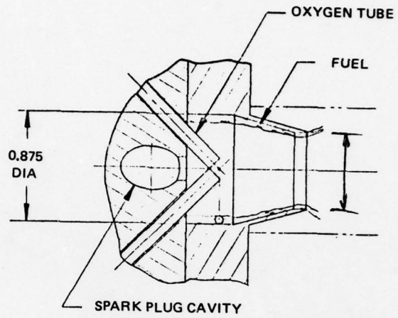
MODIFIED DESIGN
