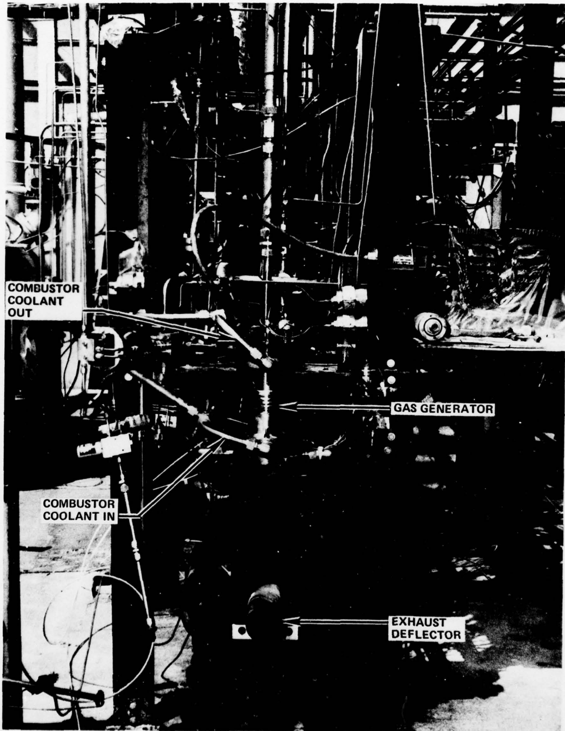
Figure 36. Overall High-Power Gas Generator Test Installation
