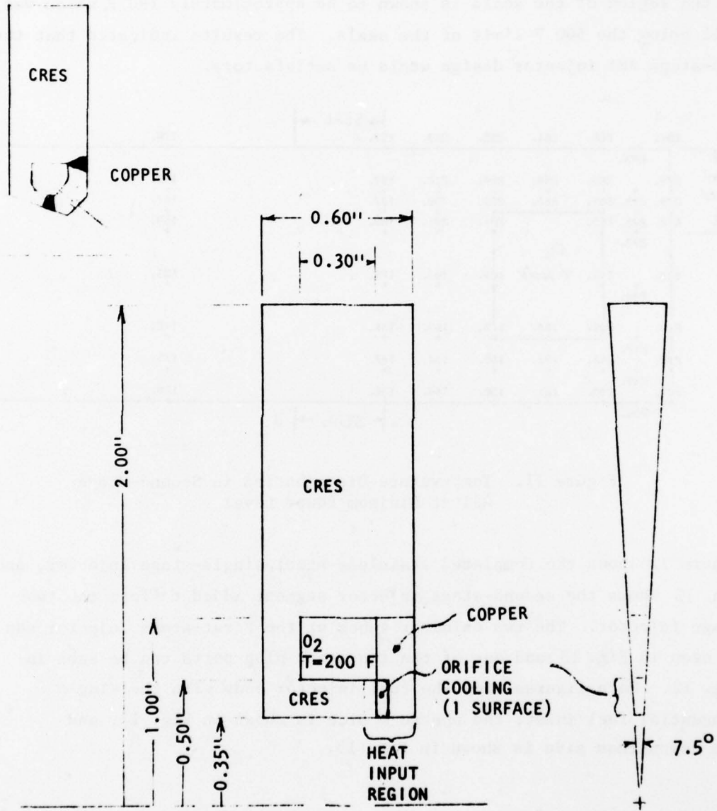
Figure 10. ASI Second Stage, 3-Dimensional Thermal Model
