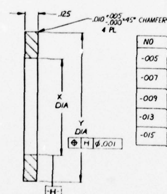
DETAIL -005, -007, -009, -013, -015 RINGS NO SCALE
