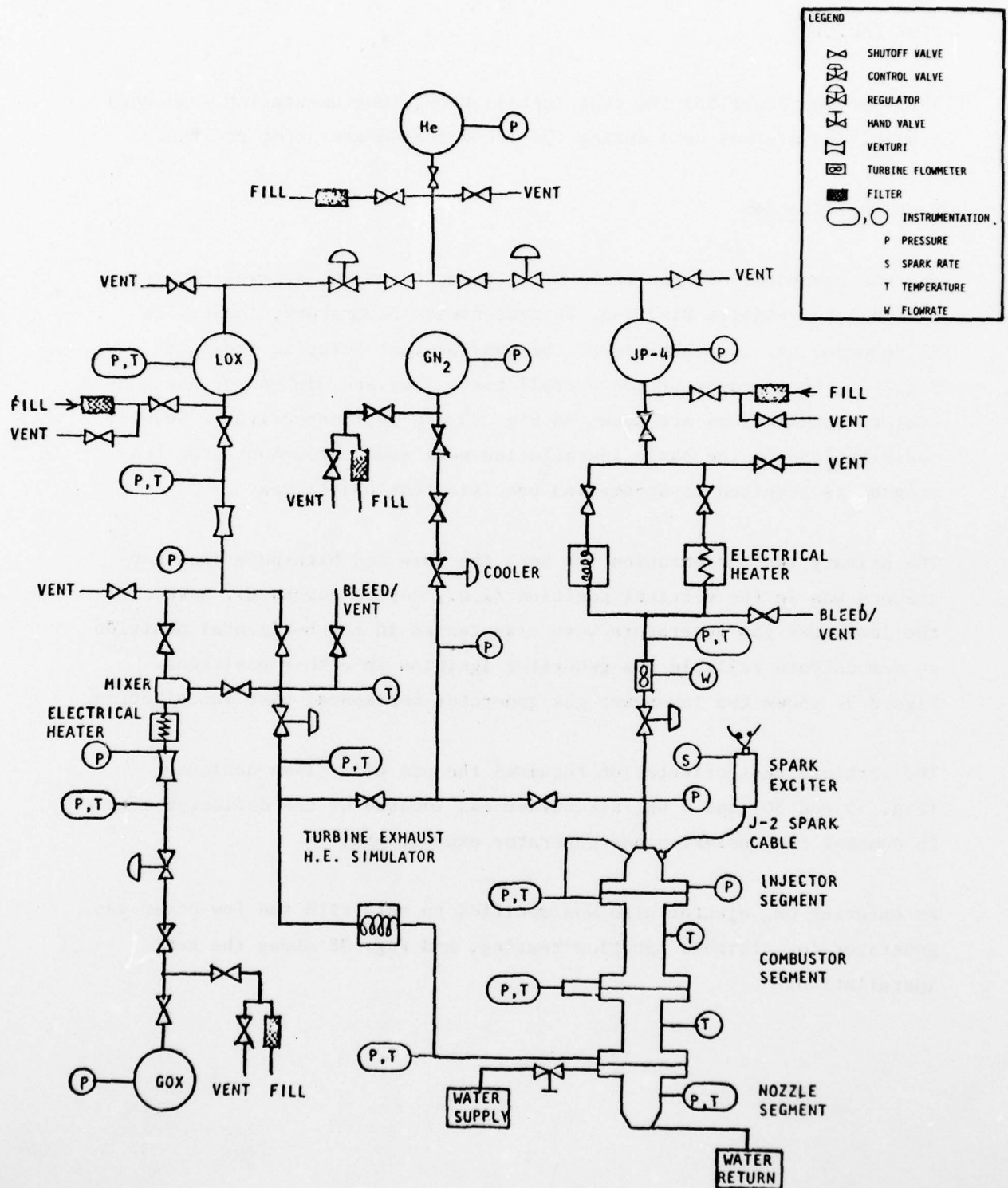
Figure 34. Gas Generator Test Installation Schematic and Instrumentation
