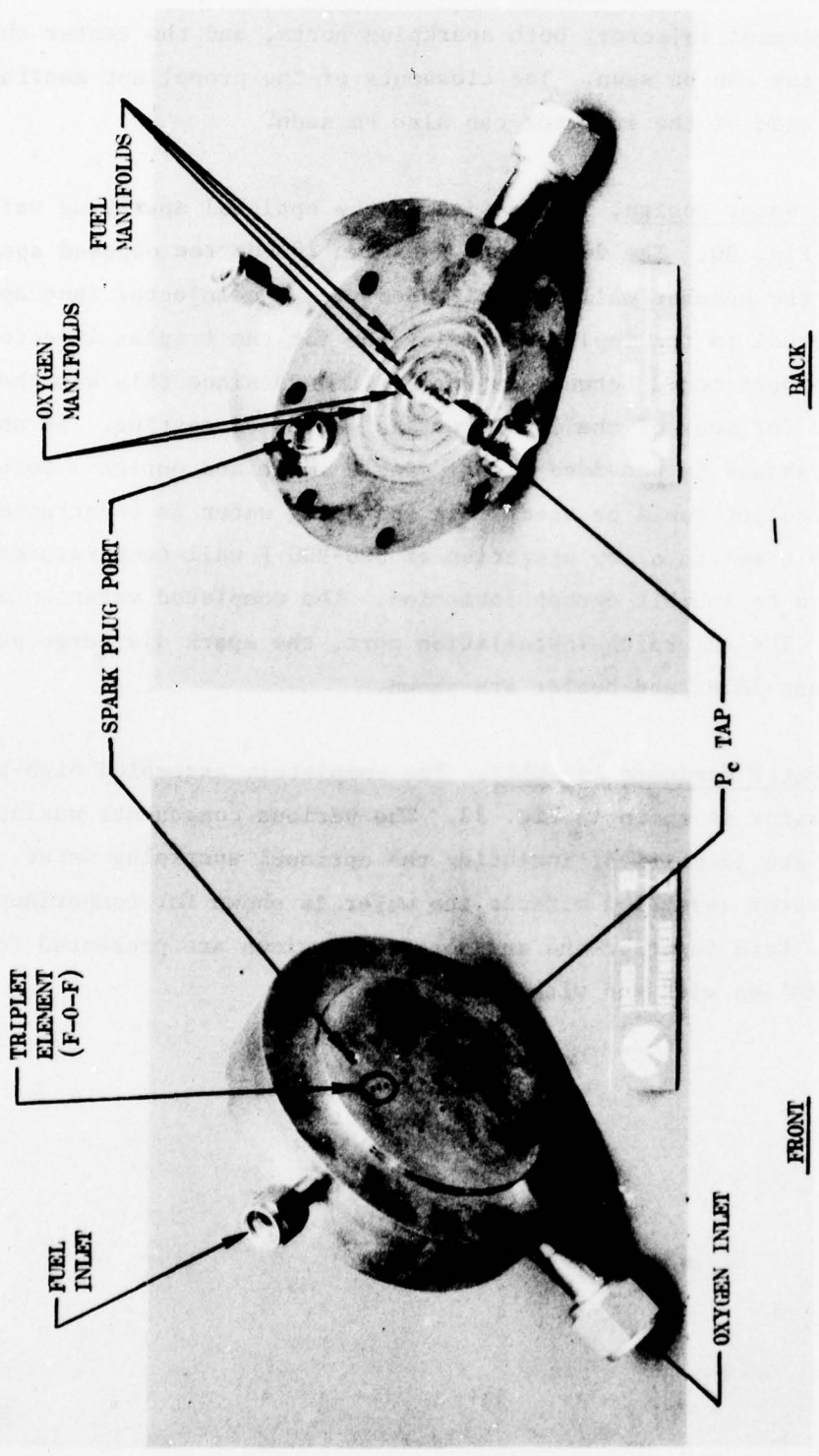
Figure 29. High-Power Gas Generator Injector
