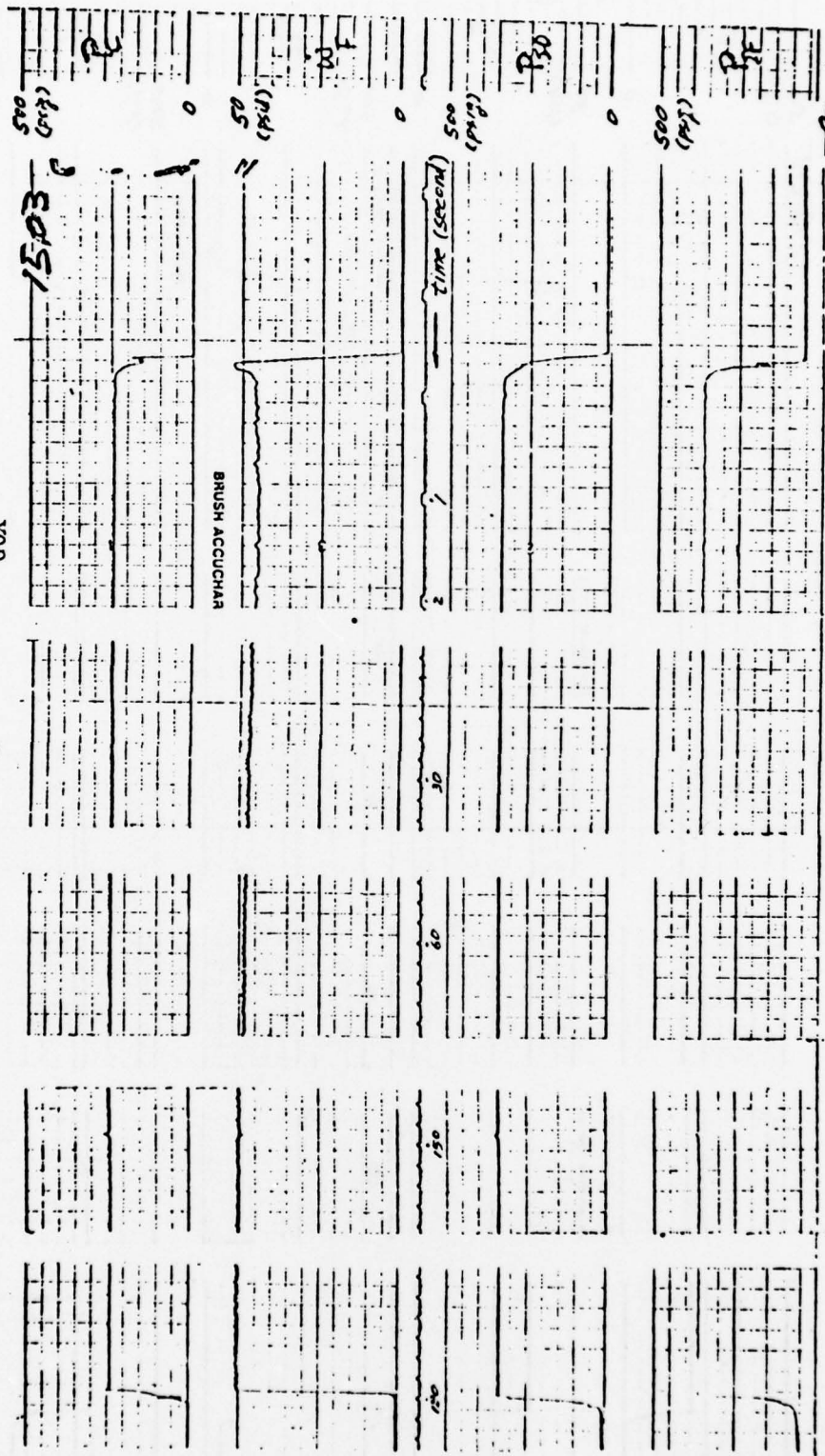
Figure 72. Long Duration Test at 130% Power Level (MR = 0.57)
