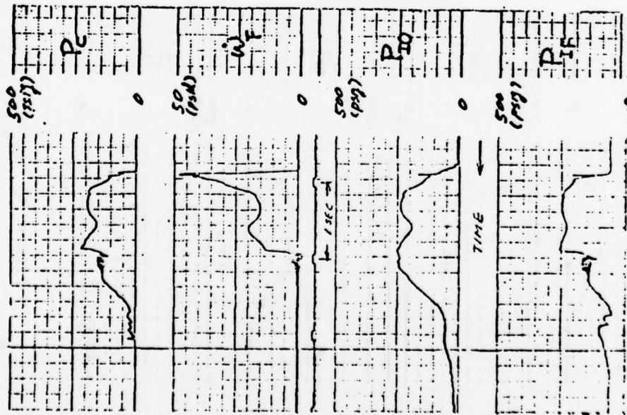
Figure 77. Ignition Diagnostics for Cold Propellants (JP-4 = -70F, GOX = -170F)
