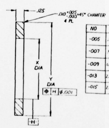
DETAIL -005, -007, -009, -013, -015 RINGS NO SCALE
