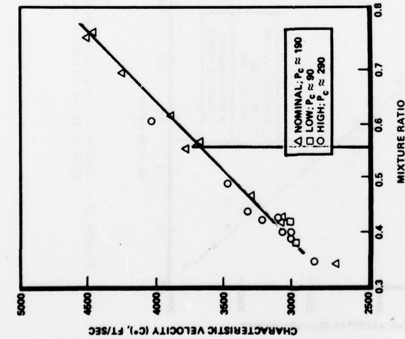
Figure 56. ASI Injector Evaluation Test Summary, 10-Inch Combustor
