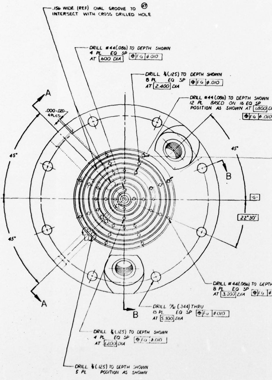
DETAIL -003 BODY
