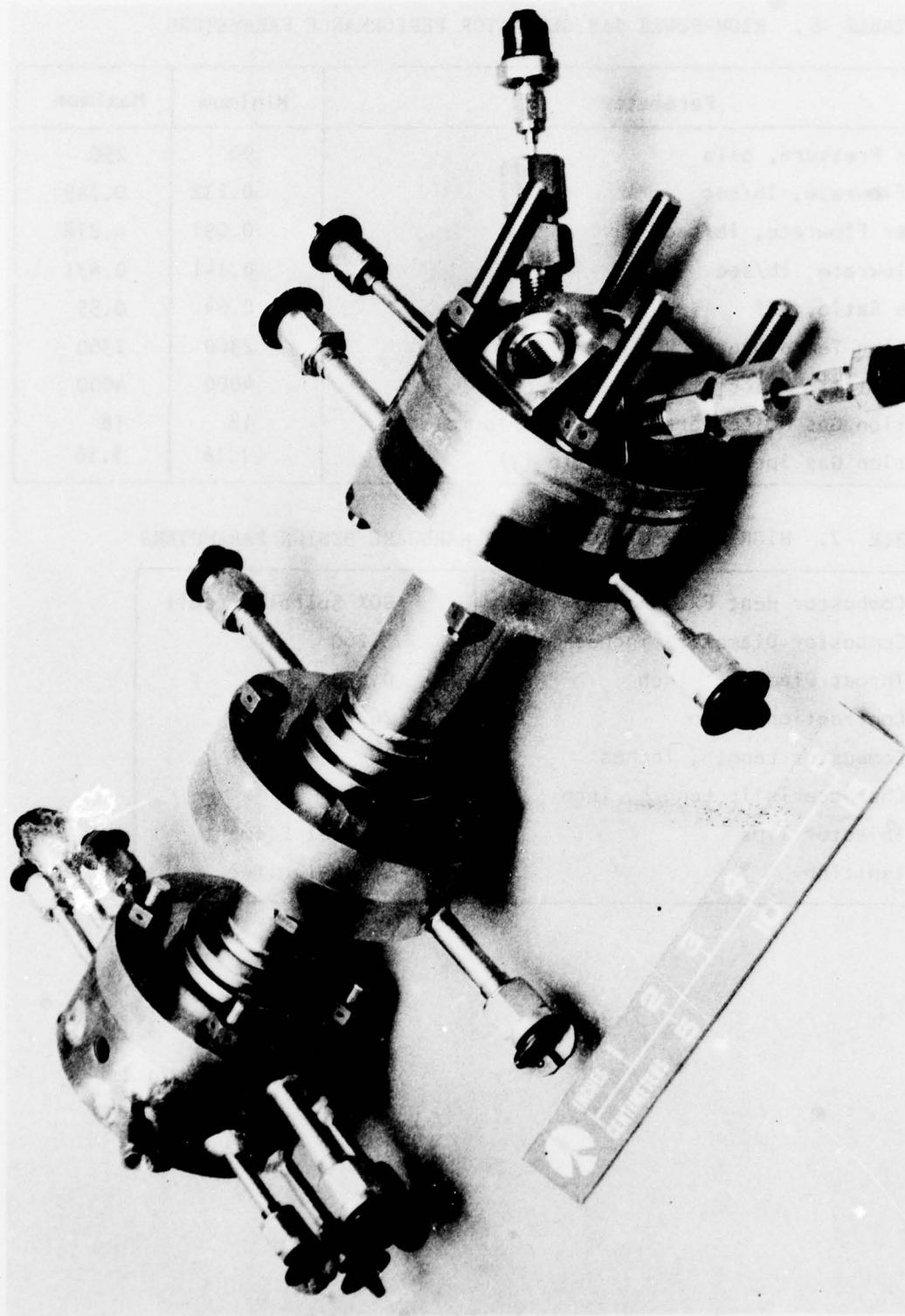
Figure 19. Low-Power Gas Generator Test Hardware Assembly (Two-Stage ASI Injector/1 inch Combustor)
