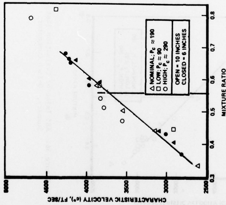
Figure 58. Combustor Length Variation With Triplet Injector
