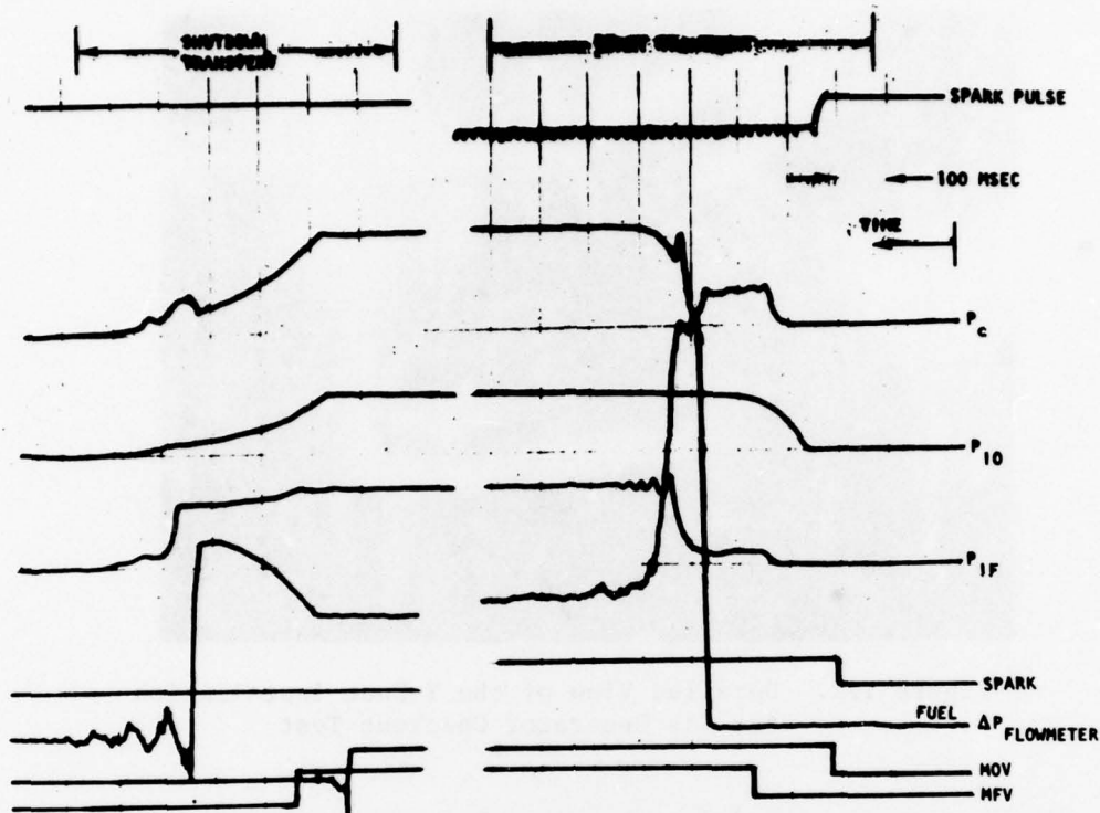
Figure 120. Oscillograph Showing Start and shutdown Transient (Test 2.06)
