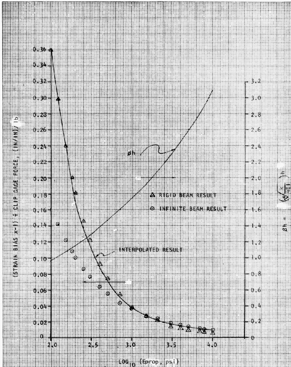
Figure 11. Strain Bias as a Function of Propellant Modulus Produced by Deflection of Mounting Pins (Eccentricity = 0.050 in.; Gage Length = 0.400 in; Sample Bending Ignored.)
