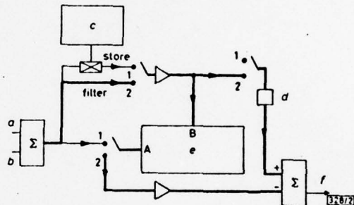
Fig. 2 S.A.W. implementation of narrowband interference canceller
