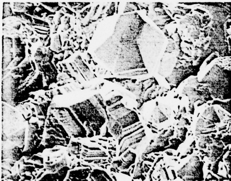
Fig. 3. Examples of GaN crystals grown on the surface of the melt in the horizontal gradient transport arrangement (800X).
