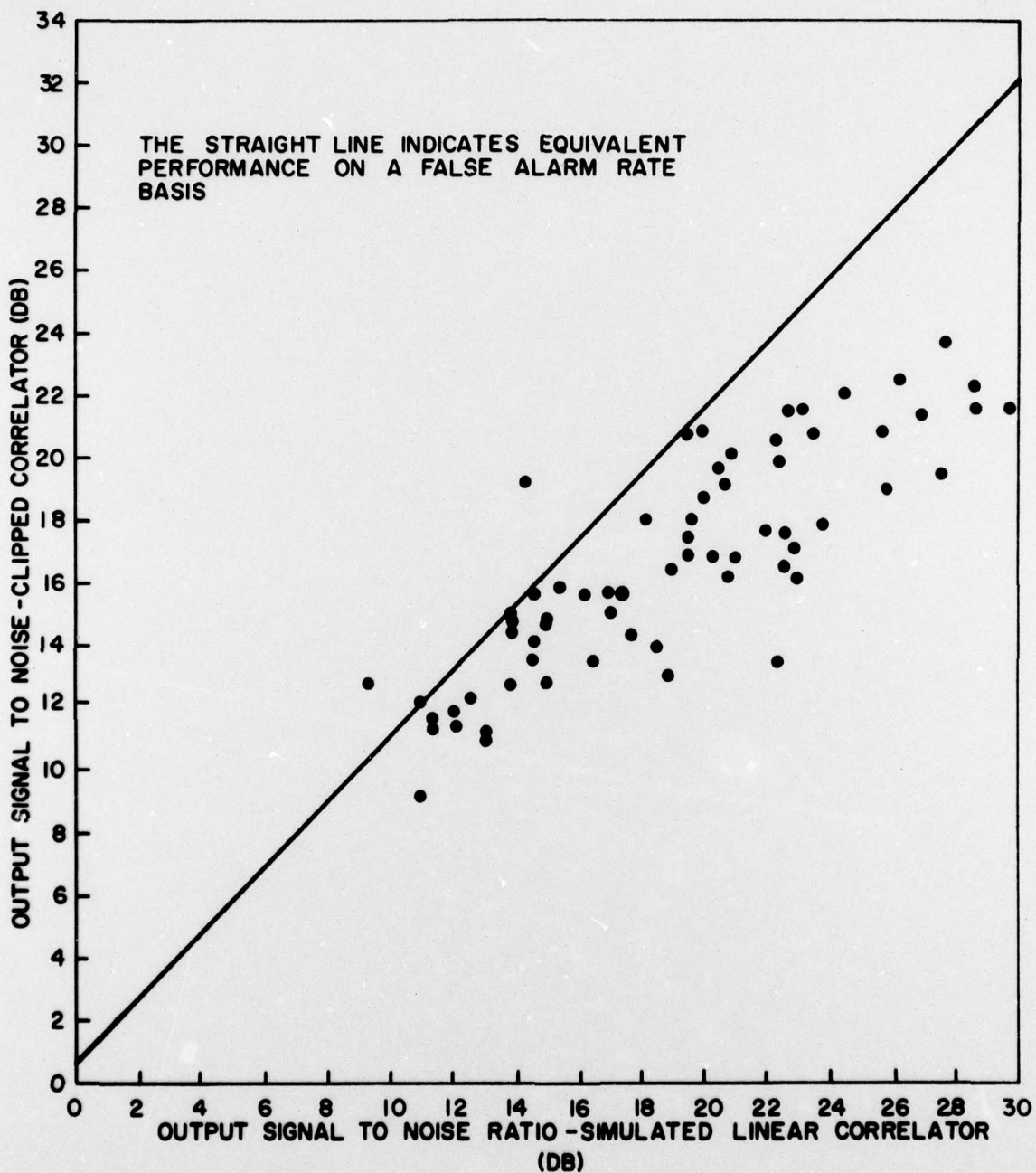
FIG.3 - OUTPUT SIGNAL TO NOISE RATIO FROM THE CLIPPED CORRELATOR VS OUTPUT SIGNAL TO NOISE RATIO FROM THE SIMULATED LINEAR CORRELATOR
