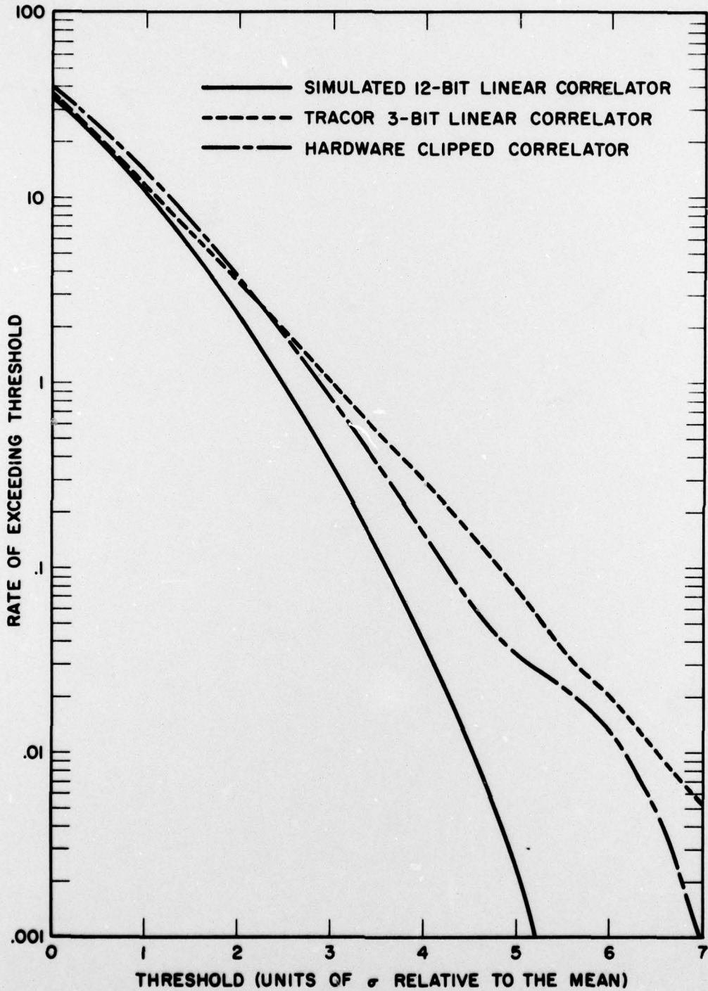
FIG. 4 - RATE OF EXCEEDING THRESHOLD VS THRESHOLD SETTING
