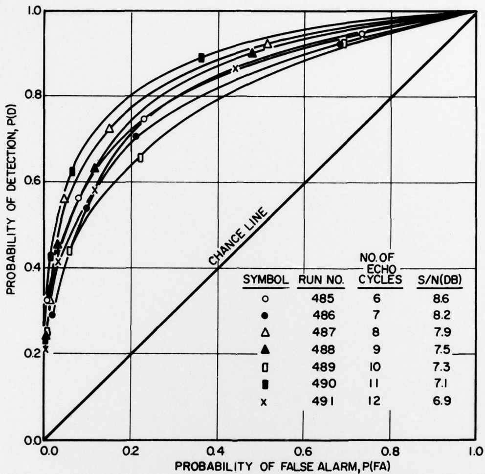
FIG. 4 - OBSERVER'S ROC CURVES FOR GROUP II FILM STRIPS. THE INDICATED S/N ARE AT THE INPUT TO THE DISPLAY.
