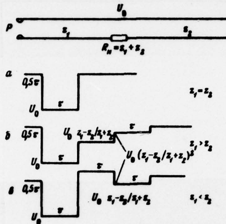
Fig. 2. Shaping of the pulses in a double shaping line at different ratios of wave impedances of its lines.
