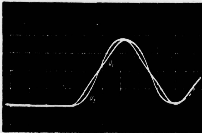
Fig. 4. Charged voltages on lines of DFL V_1 on \Pi_1 and V_2 on \Pi_2 . Scale along the horizontal is 0.2 \mu\text{s/cm} and along the vertical, 200 \text{ kV/cm} .
