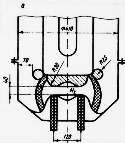
Fig. 1. Schematic diagram of the generator
