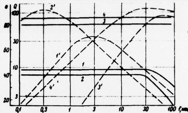
Fig. 3. Frequency dependences of the dielectric constant \epsilon_1 (solid lines) and quality Q = 1/\text{tg } \delta (dashed lines): 1.1 1 - technical glycerine ( \rho = 1.7 \cdot 10^6 ); 2.2 1 - glycerine "r" ( \rho = 60 \cdot 10^6 ); 3.3 1 - distilled water ( \rho = 10^4 ); 4.4 1 - thoroughly cleaned water ( \rho = \sim 10^6 ); \rho - volume resistance [ohms.cm].
