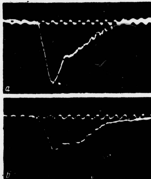
Fig. 4. Shape of pulses of accelerating voltage a) and current b) of the beam. Marks are 100 MHz.
