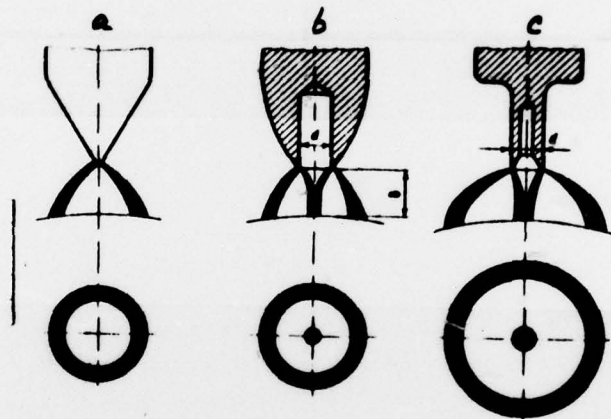
Fig. 5. Trajectories of electrons and shape of the beam on the anode for different emitters. The energy of the electrons W_e = 1 + 1.5 \text{ MeV} , \delta = 2 \text{ cm} ; d = 1.2 \text{ cm} .
