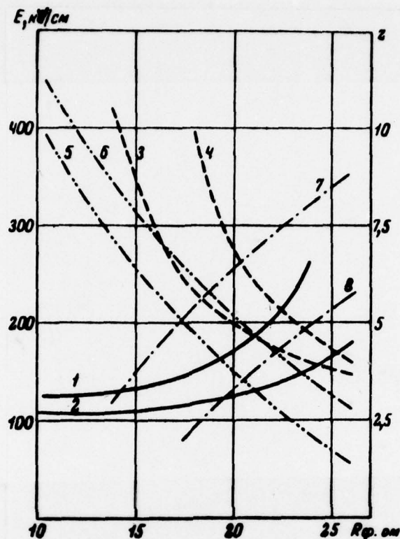
Fig. 3. Field strength in lines and wave impedances as a function of the geometry of the lines. 1 - E_H when D_1 = 60 cm; 2 - E_H when D_1 = 70 cm; 3 - E_{BH} when D_3 = 20 cm; 4 - E_{BH} when D_3 = 28 cm; 5 - Z_{HAP} when D_1 = 60 cm; 6 - Z_{HAP} when D_1 = 70 cm; 7 - when D_3 = 20 cm; 8 - Z_{BH} when D_3 = 28 cm.
