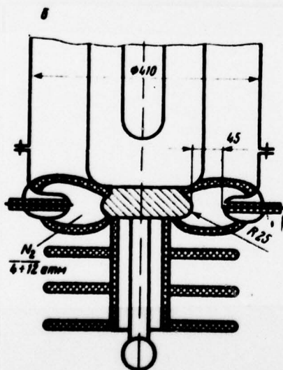
Fig. 2. Spark gap of the double shaping line of axial (a) and radial (b) types.
