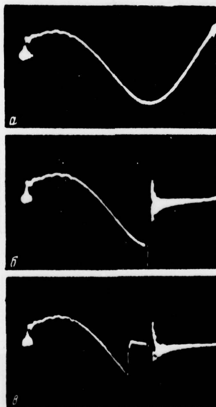
Fig. 3. Voltage on the accelerator tube during the whole cycle of operation of the apparatus. a - spark gap-peaker did not trigger; b - spark gap triggered (a jump in the voltage on the tube is evident); c - in the pre-impulse stage there occurred a "cutoff" of the voltage (breakdown of the vacuum gap). Sweep is 5 ms/cm.
