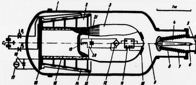
Fig. 1. Schematic cross section of the apparatus
