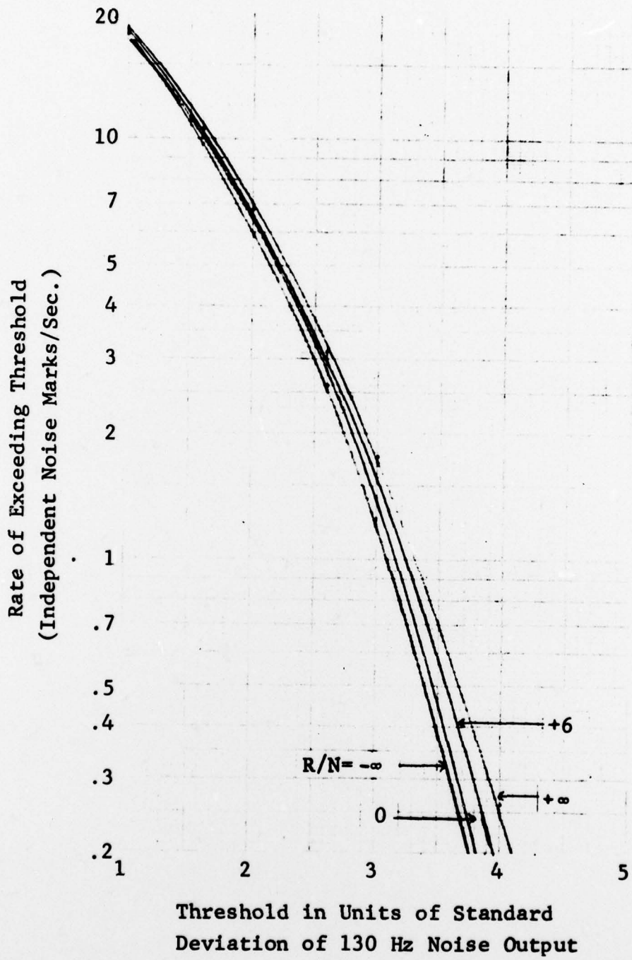
Fig. 7 - Mean-Divider Output Clutter Statistics for Different Values of Reverberation-to-Noise Ratio
