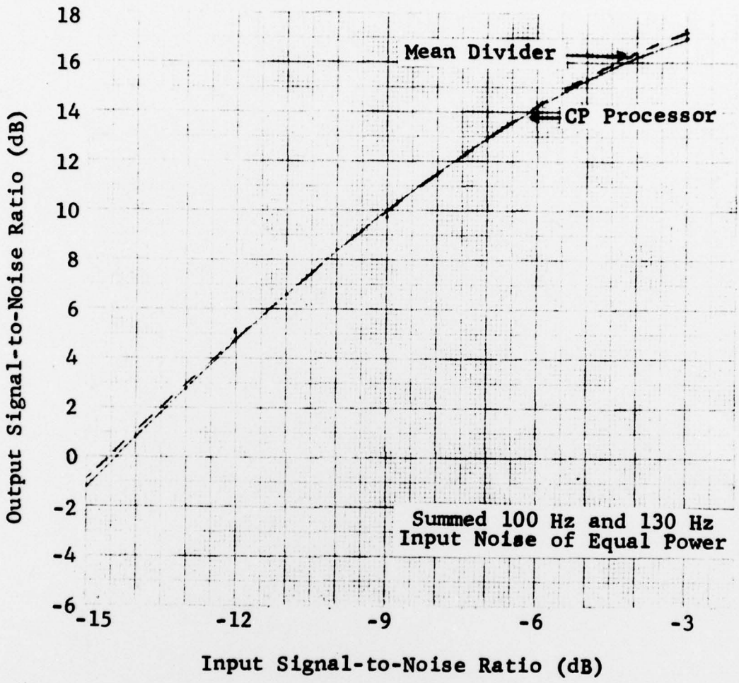
Fig. 10 - Processing Gain for CP Processor and Mean-Divider, Summed 100 Hz and 130 Hz Input Noise
