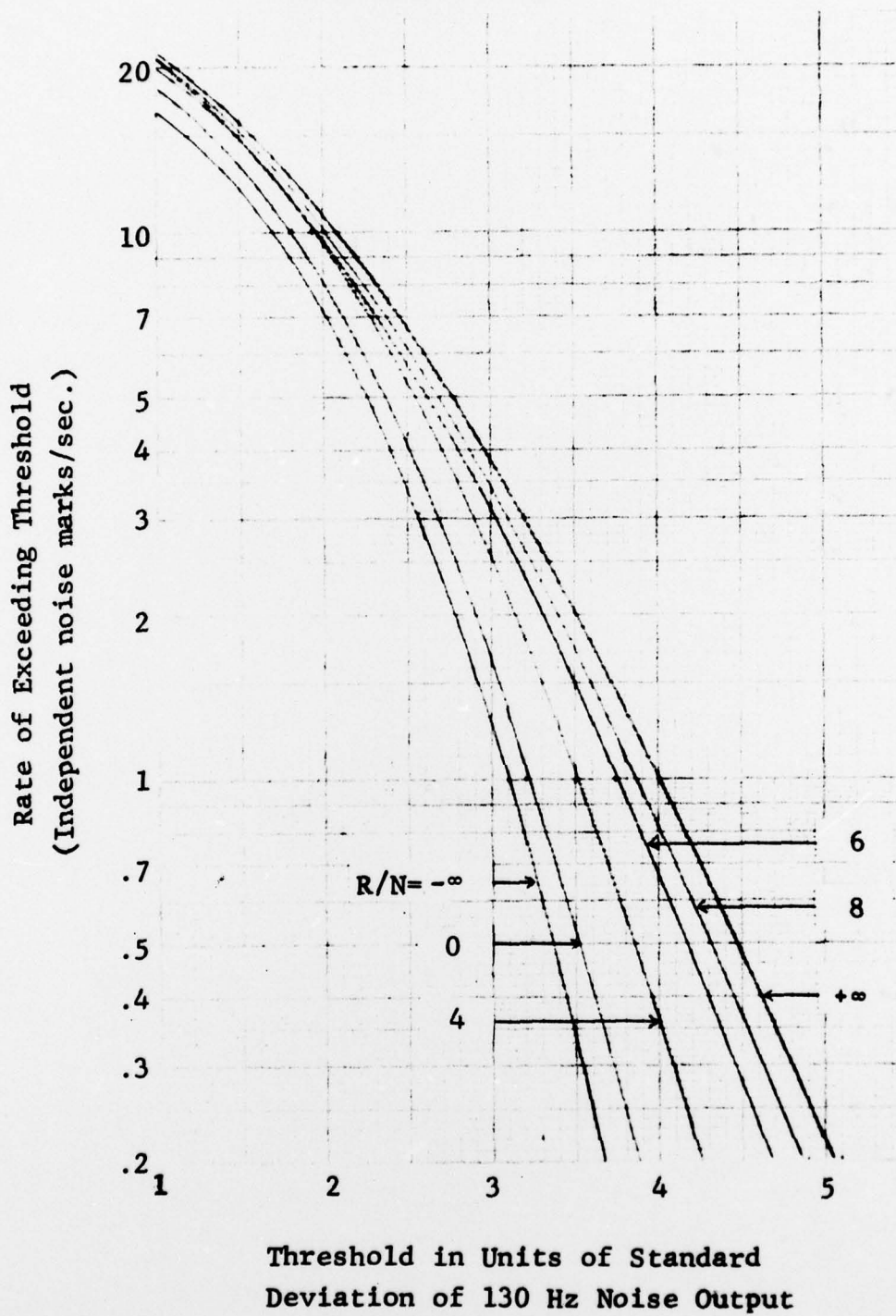
Fig. 6 - CP Processor Output Clutter Statistics for Different Values of Reverberation-to-Noise Ratio
