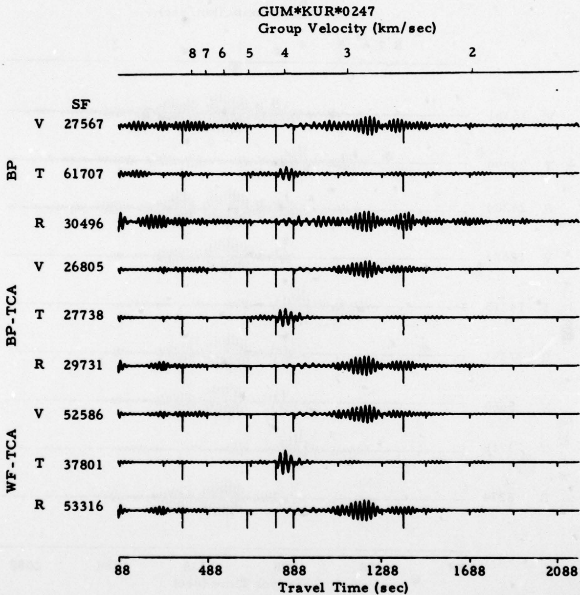
FIGURE II-3 POLARIZATION FILTER RESULTS (Strauss, 1978) (PAGE 2 OF 5)
