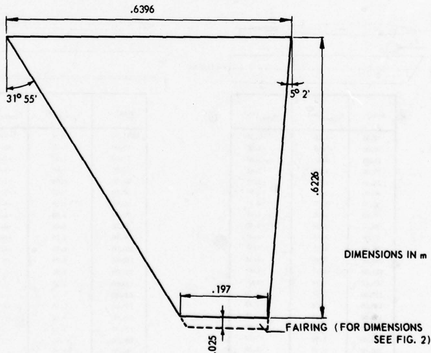
Fig. 1 Dimensions of the wing
