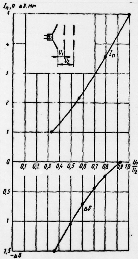
Fig. 8. Characteristics of the electron guns EP-6 and EP-9.
