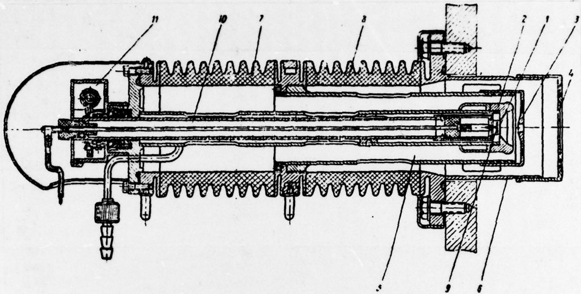
Fig. 7. Overall view of the electron gun EP-9.
