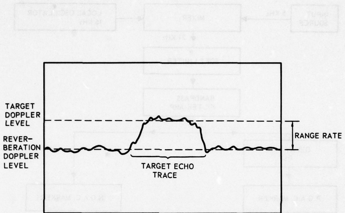
Figure 1. Simulated output trace of FACT unit showing the target echo and re- verberation region.
