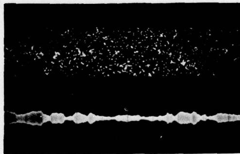
Figure 17. Photographs showing DACIM I and FACT unit outputs for similar inputs, consisting of 30 ms pulses plus narrowband noise centered at 5 KHz, with a bandwidth of 35 Hz. The sine wave frequency was 5080 Hz simulating a Doppler shift of 80 Hz or approximately 23 Knots. The rms signal to noise ratio is given for each trace.
