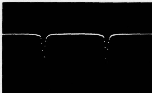
Figure 18. Photographs showing the FACT unit and DACIM I outputs for an input consisting of two sine wave components. The input signal is given by the relation x(t) = A_1 \sin(2\pi f_1 t) + A_2 \sin(2\pi f_2 t) where f_1 = 5010 Hz, f_2 = 5000 Hz, A_1 = 1.1 vrms and A_2 = 1.0 vrms. The FACT unit Doppler scale is approximately 100 Knots/division. The DACIM I Doppler scale is approximately 50 Knots/division.
