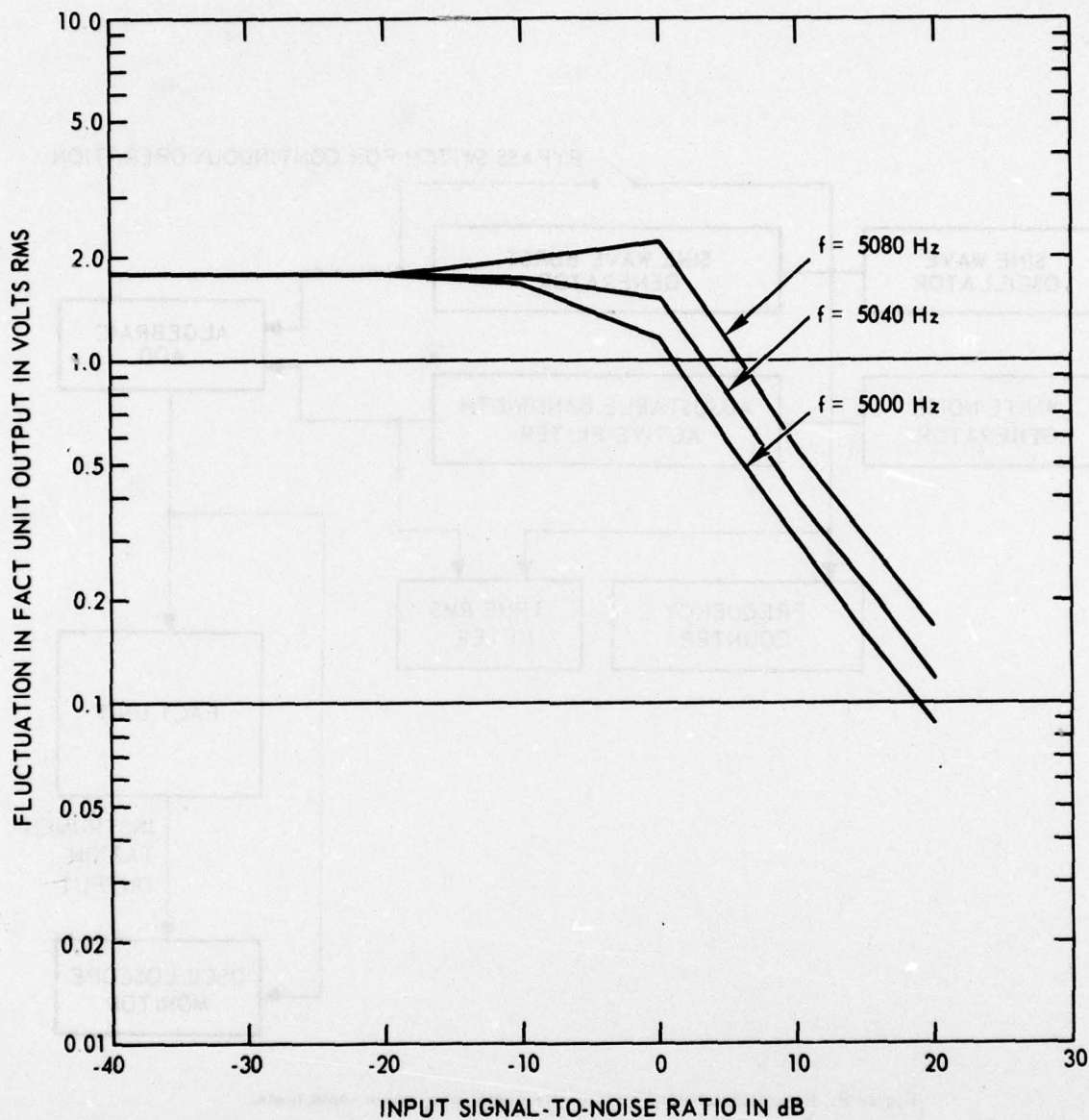
Figure 8. Rms fluctuation in FACT unit output vs signal-to-noise ratio for an input consisting of a pure sine wave plus narrow band noise. The noise bandwidth is 40 Hz centered at 5 KHz, and the noise amplitude is 0.2 vrms. One volt rms fluctuation is approximately equivalent to 17 knots rms fluctuation. The sine wave frequency for each curve is indicated.
