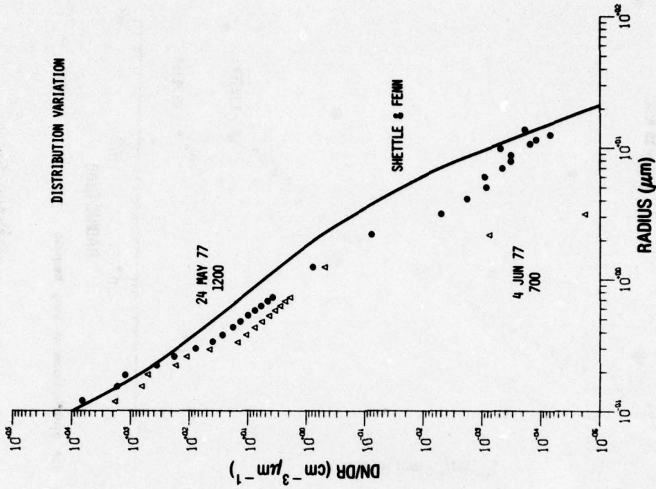
Fig. 17 - Atlantic and Mediterranean size distributions compared with predictions of Shettle and Fenn model
