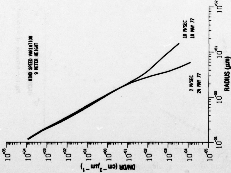
Fig. 16 - Comparison of size distributions at two windspeeds
