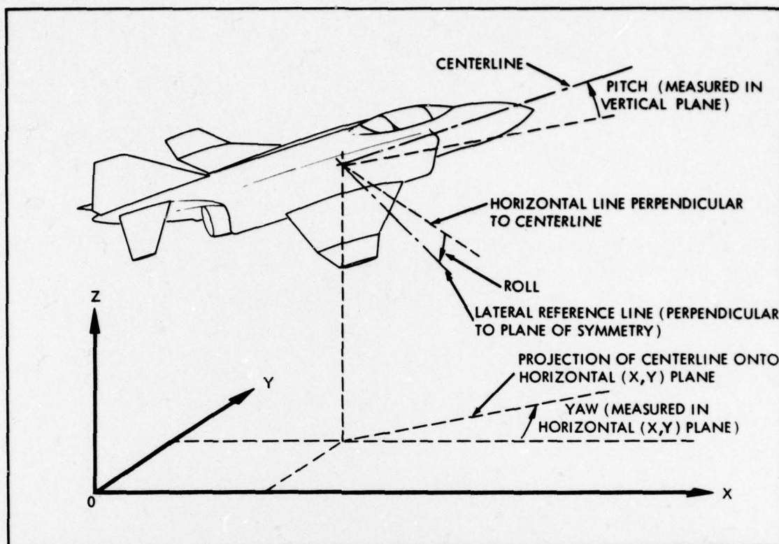
Figure 1. Description of Aircraft Yaw, Pitch, and Roll Angles
