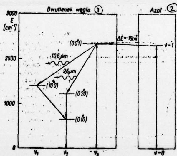
Fig 2. Diagram of the lower oscillatory energy levels of CO 2 and N 2 molecules
