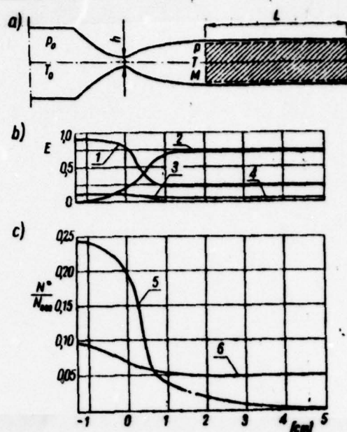
Fig 3. Typical work condition of the gas dynamic laser (initial mixture parameters: 0.075 \text{CO}_2 , 0.913 \text{N}_2 , 0.012 \text{H}_2\text{O} , p_0 = 17 ata, T_0 = 1400^\circ\text{K} , nozzle parameters: h = 0.8 mm, A/A^* = 14 , mixture parameters of the nozzle exhaust: T = 354^\circ\text{K} , M = 4.02 , p = 0.086 ata)
