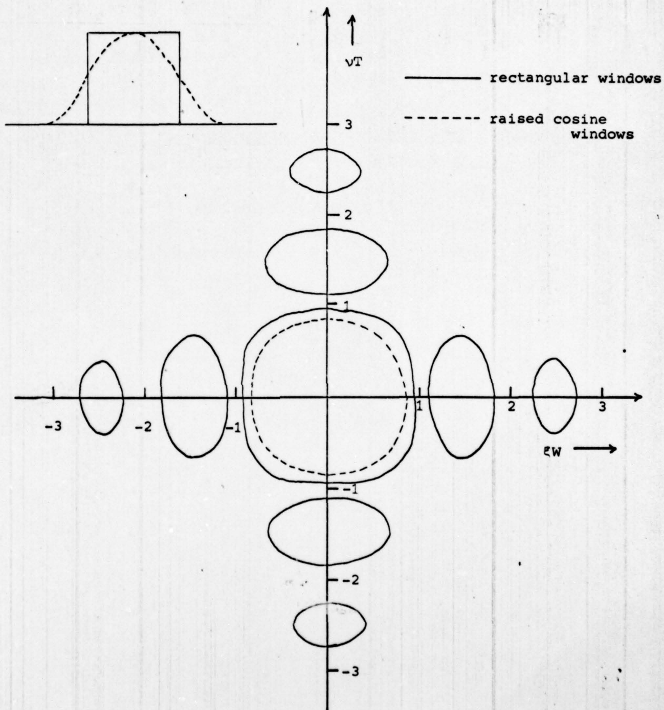
Fig. 4 Occupancy Patterns of Segmented Channels With Raised Cosine and Rectangular Gates for a 10% Threshold Level.
