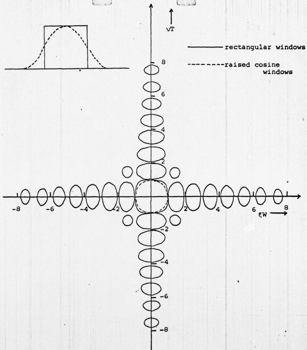
Fig. 5 Occupancy Patterns of Segmented Channels with Raised Cosine and Rectangular Gates for a 3% Threshold Level.
