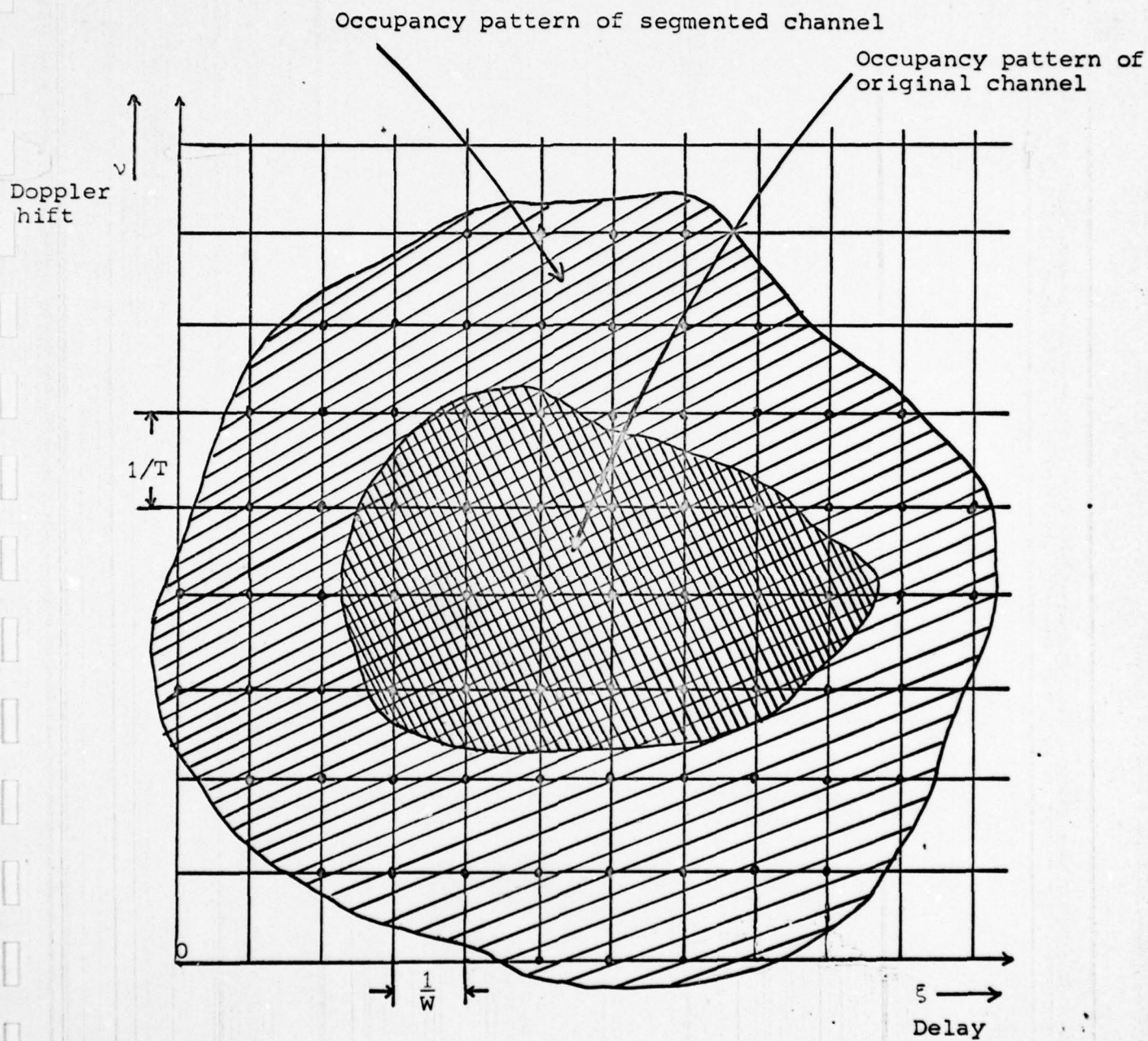
Figure 3 DISCRETE SPECTRAL REPRESENTATION OF SEGMENTED CHANNEL
