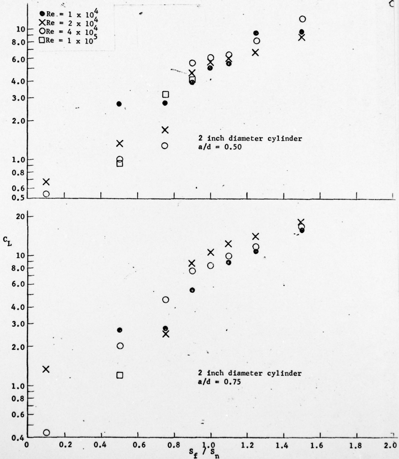
Figure 5 continued - Variation of Lift Coefficient as Function of the Ratio of Forced to Natural Strouhal Numbers for Various Reynolds Number and Ratio of Amplitude to Diameter
