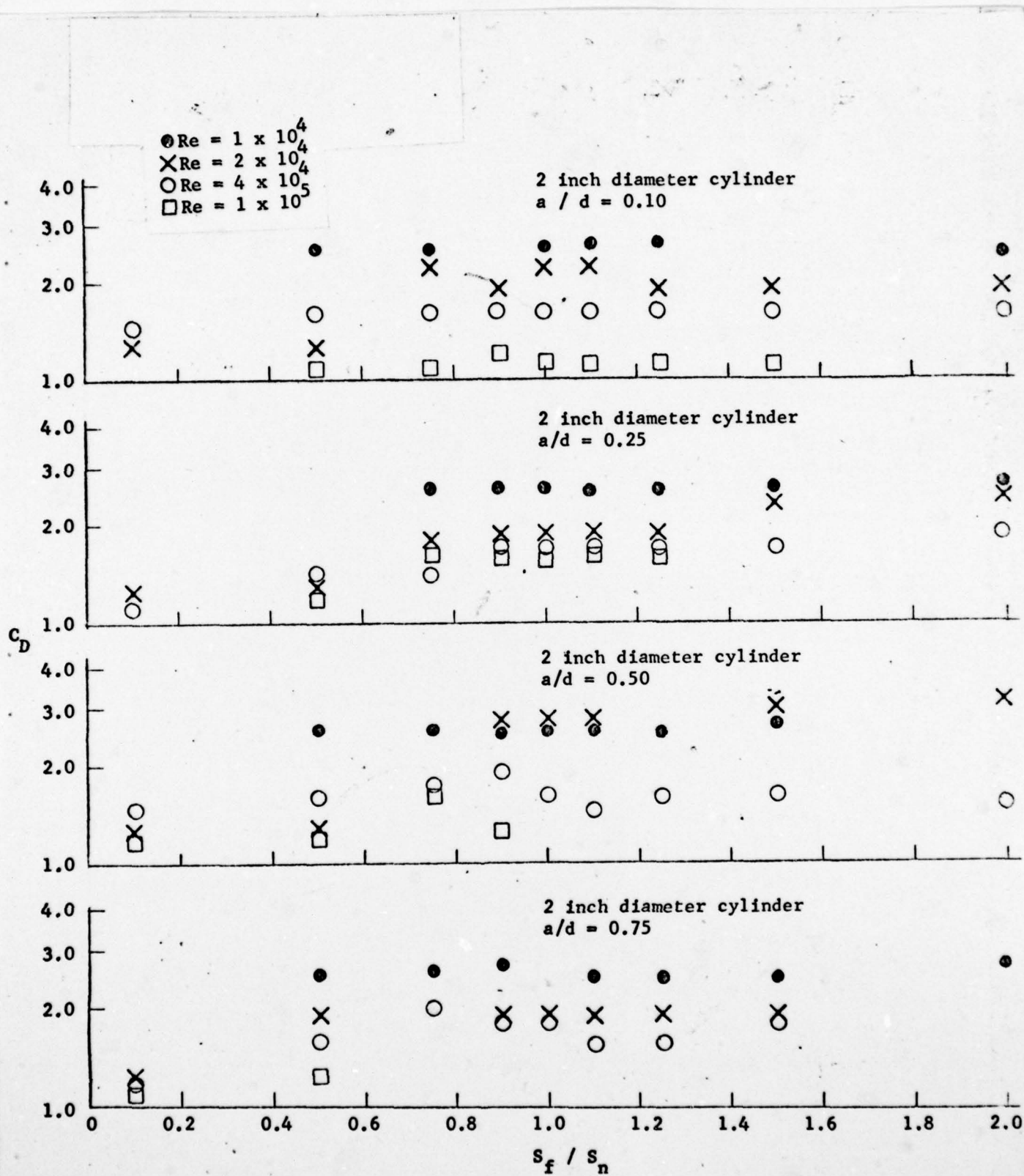
Figure 4 - Variation of Drag Coefficient as Function of the Ratio of Forced to Natural Strouhal Numbers for Various Reynolds Number and Ratio of Amplitude to Diameter
