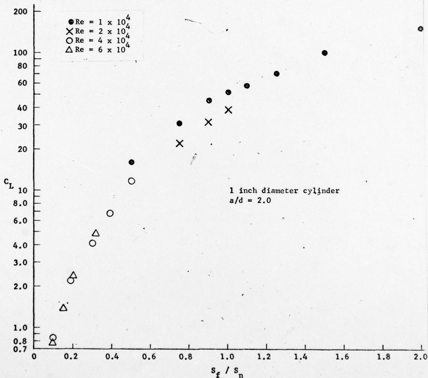
Figure 5 continued - Variation of Lift Coefficient as Function of the Ratio of Forced to Natural Strouhal Numbers for Various Reynolds Number and Ratio of Amplitude to Diameter
