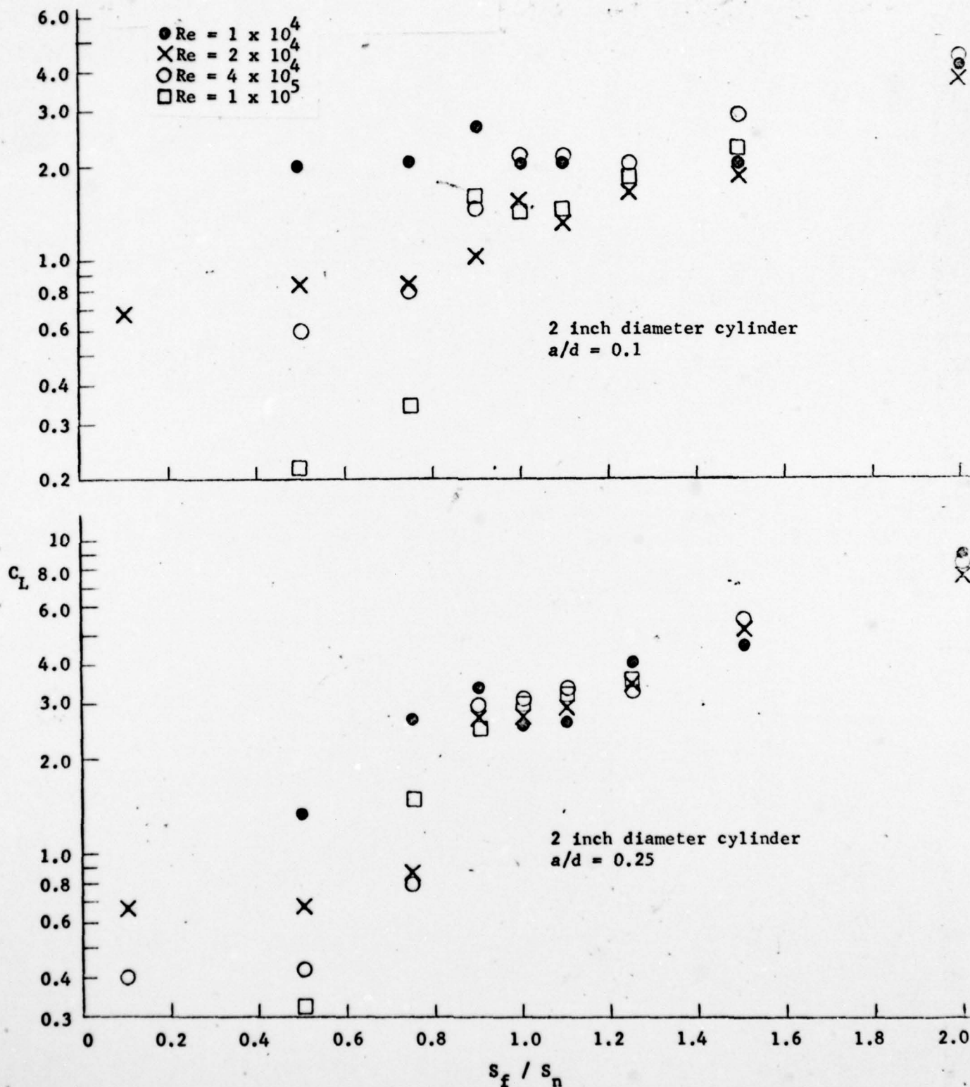
Figure 5 - Variation of Lift Coefficient as Function of the Ratio of Forced to Natural Strouhal Numbers for Various Reynolds Number and Ratio of Amplitude to Diameter
