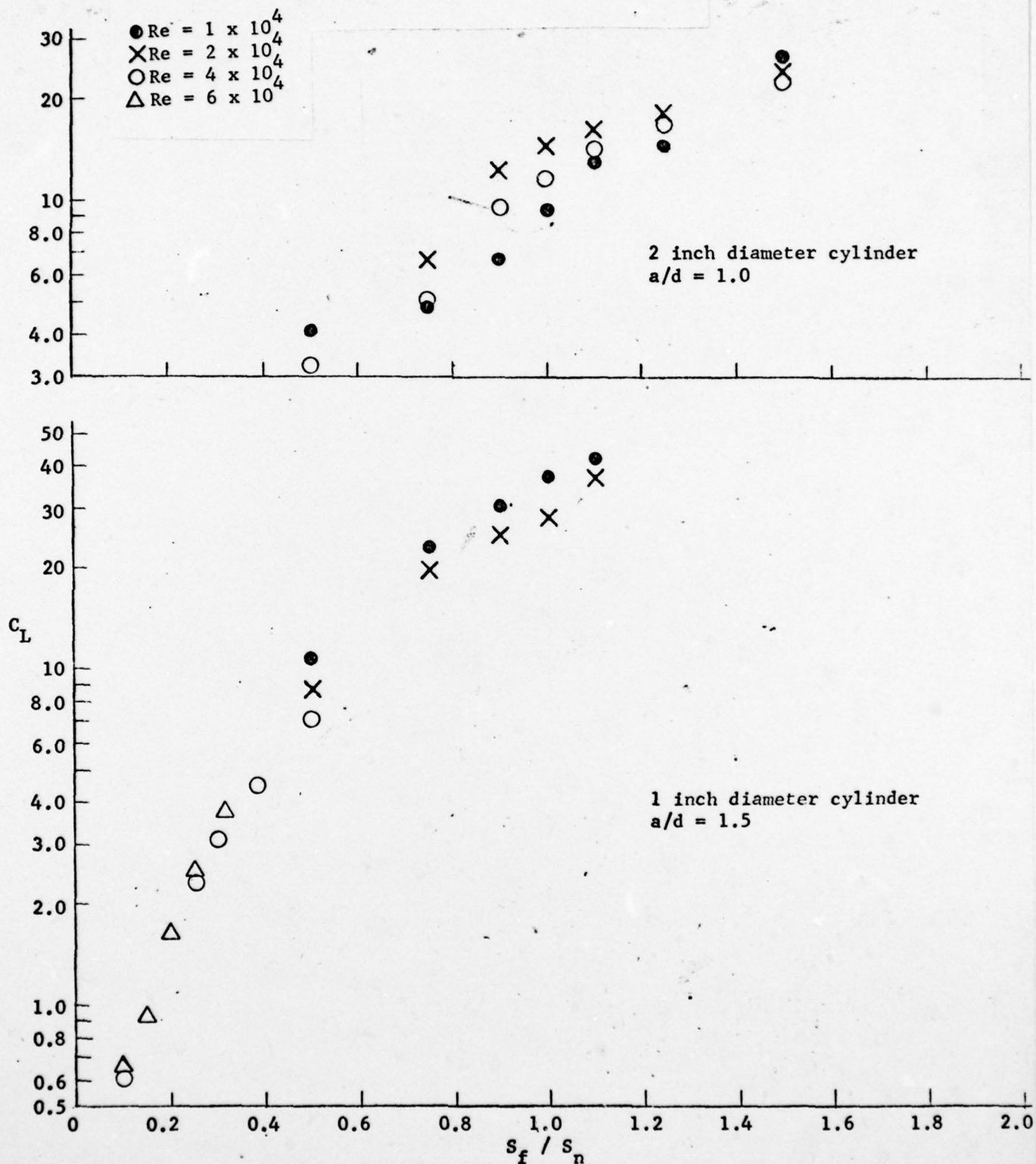
Figure 5 continued - Variation of Lift Coefficient as Function of the Ratio of Forced to Natural Strouhal Numbers for Various Reynolds Number and Ratio of Amplitude to Diameter
