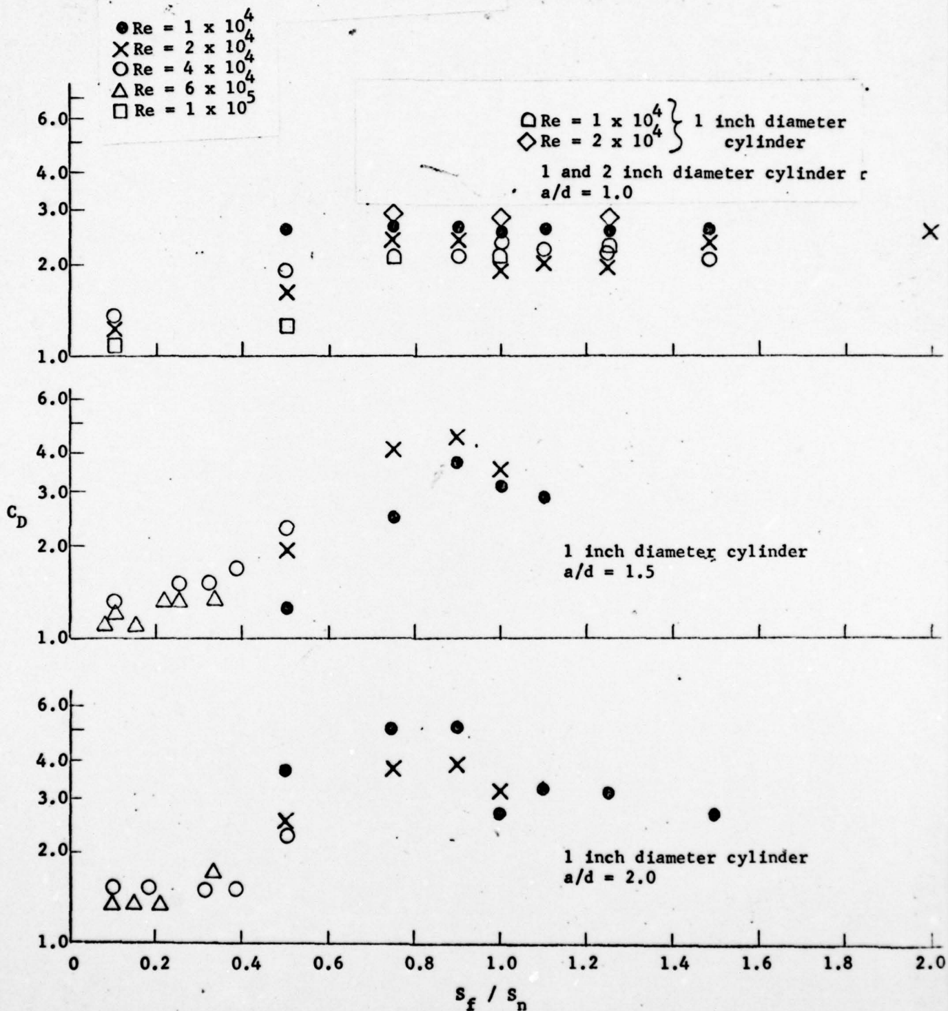
Figure 4 continued - Variation of Drag Coefficient as Function of the Ratio of Forced to Natural Strouhal Numbers for Various Reynolds Number and Ratio of Amplitude to Diameter
