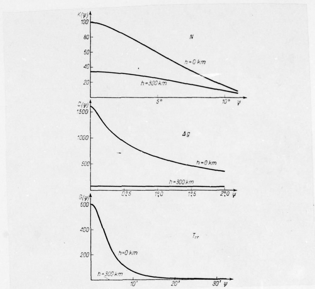
Fig. 2. Course of covariance function for geoid undulation K(\psi) , gravitational anomaly C(\psi) and gradient of the second order G(\psi)
